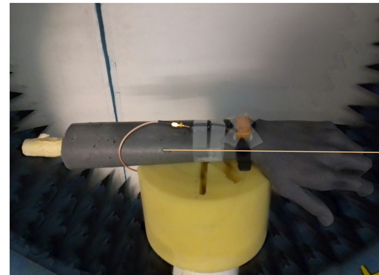
Total efficiency and max gain measurement setup
