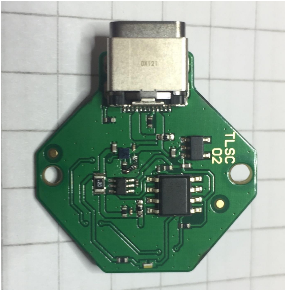
Charger PCB, bottom
