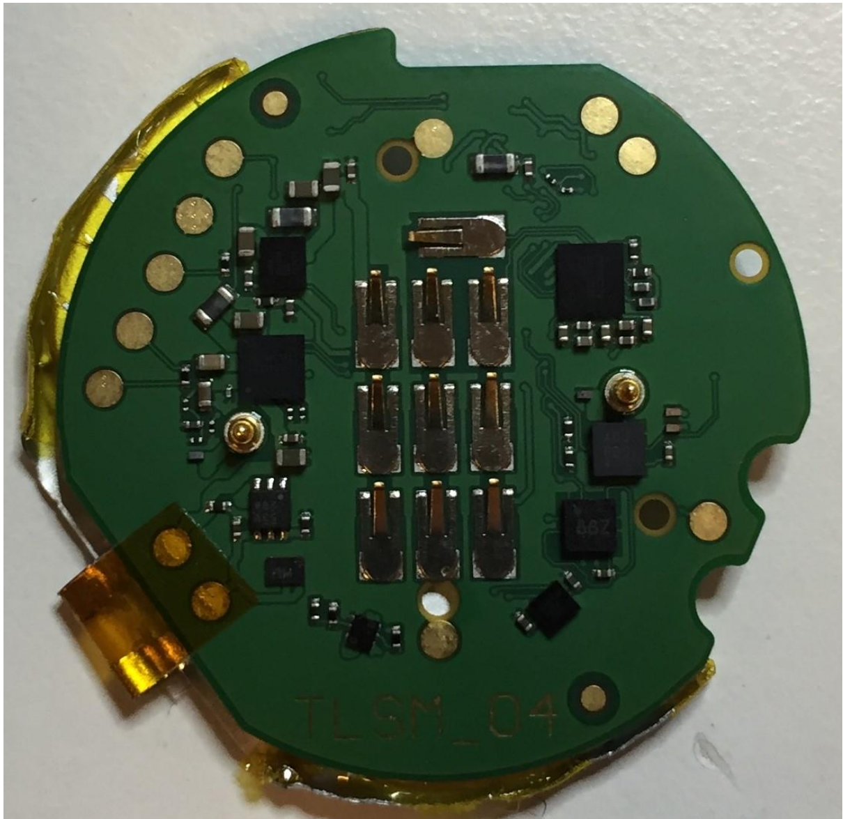
Charger PCB, top:
