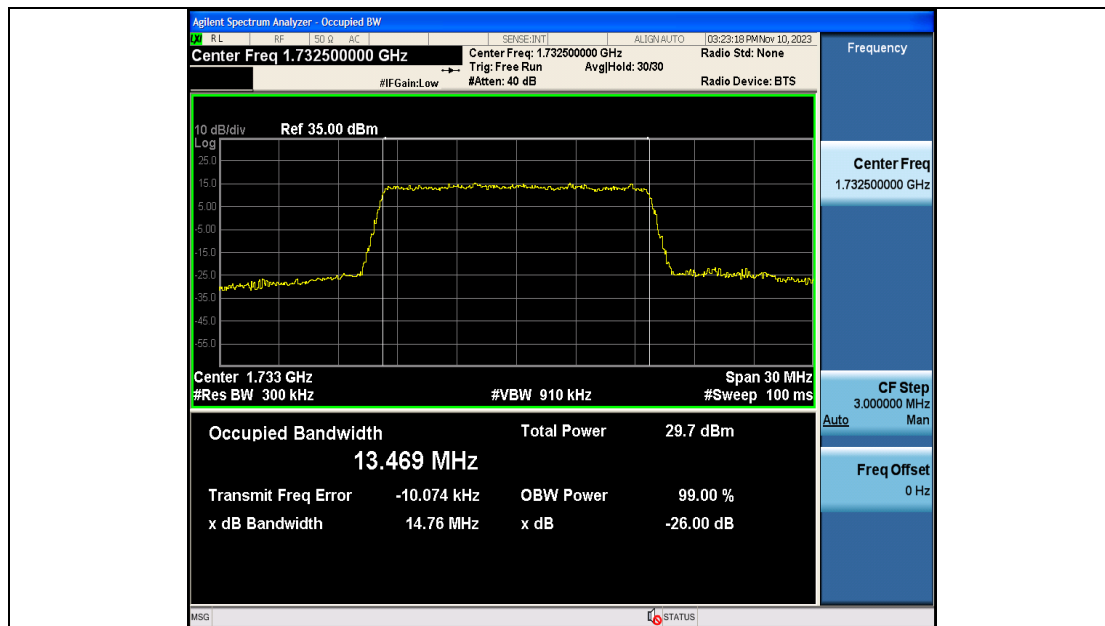
Band4-15MHz-QPSK-20175-75RB#0-PASS
