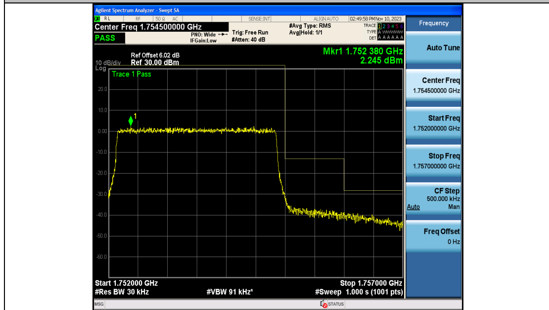
Band4_3MHz_16QAM_20385_15RB#0
