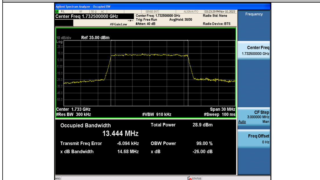
Band4-15MHz-16QAM-20175-75RB#0-PASS
