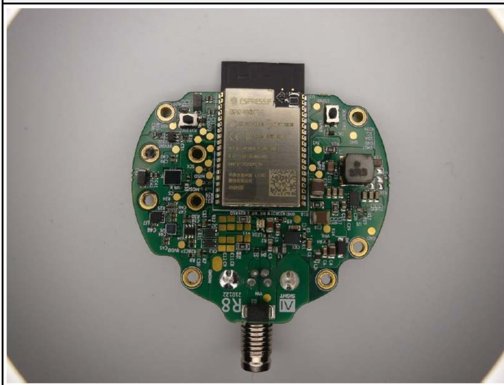
PCB with radio module (Bottom View)
