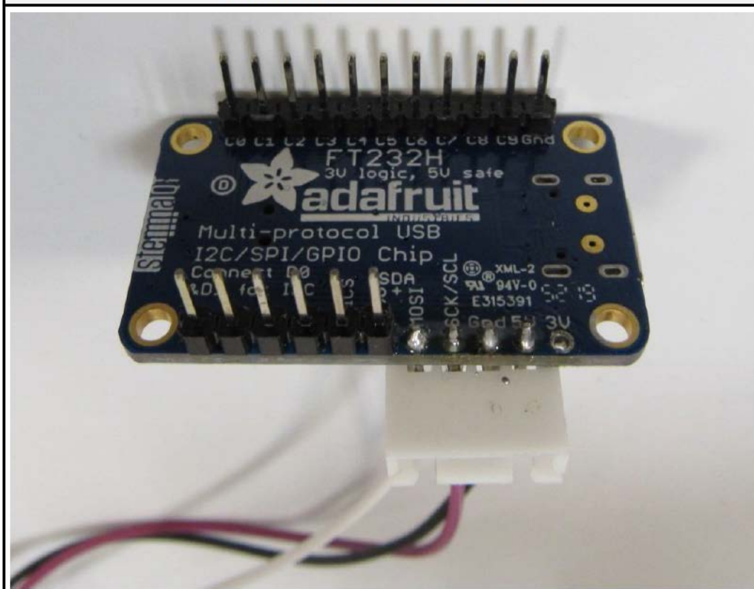
Evaluation Board Bottom View
