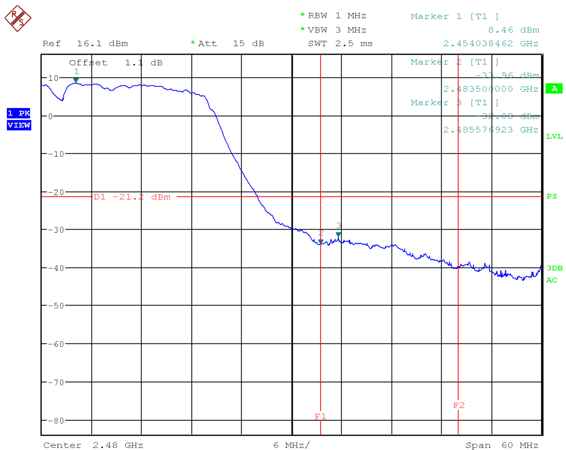
Figure 54: Chart of band-edge measurement on highest channel (PK) in modulation IEEE 802.11 n (HT40)
