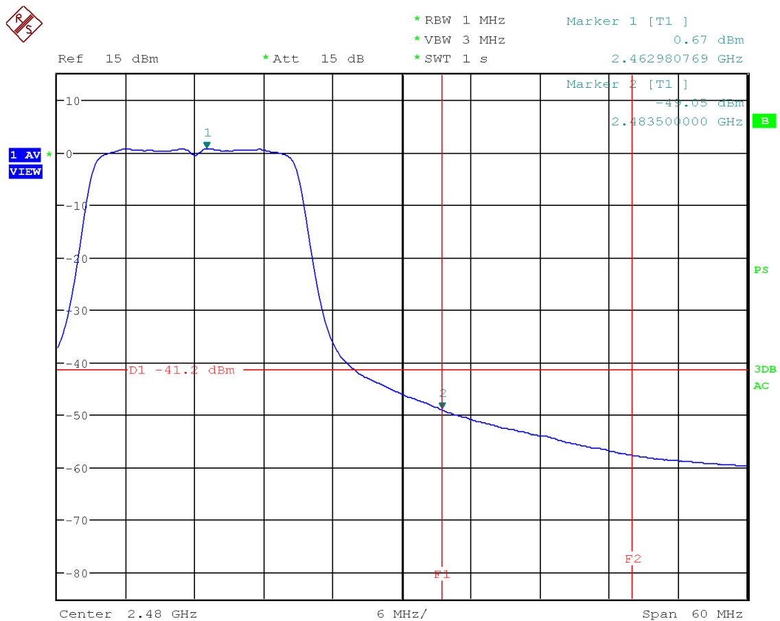
Figure 52: Chart of band-edge measurement on highest channel (AV) in modulation IEEE 802.11 n (HT20)
