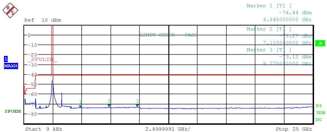
Figure 77: Chart of emissions test from 9 kHz to 25 GHz on middle channel in modulation IEEE 802.11 n (HT40), RMS-detector
