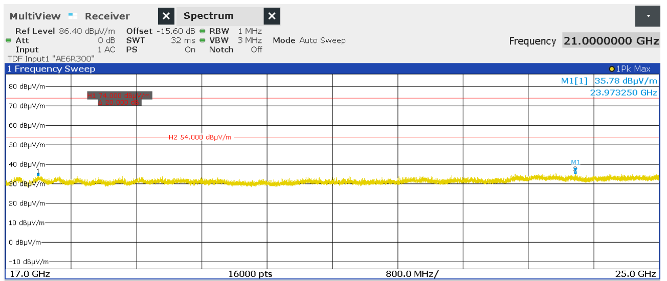
Figure 83: Chart of exploratory radiated emissions measurement from 17 GHz to 25 GHz on lowest channel
