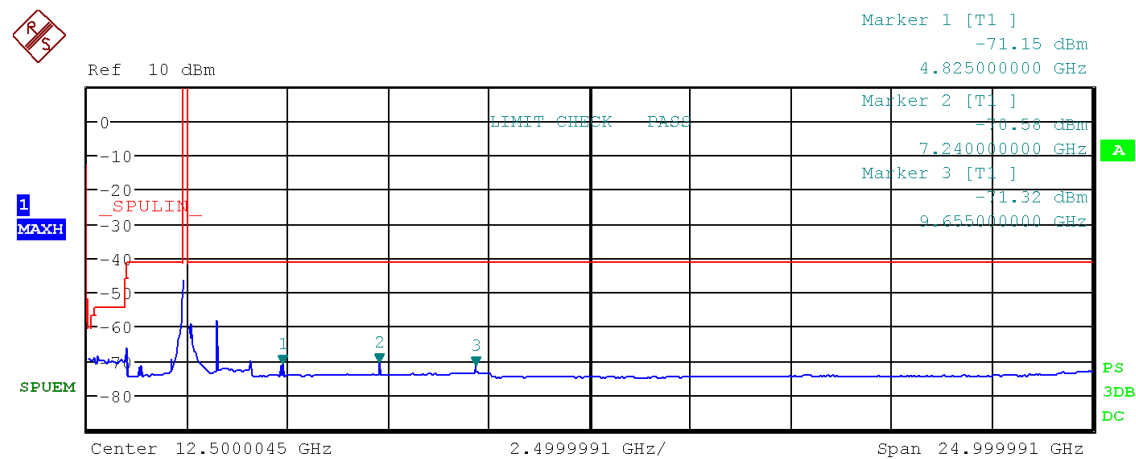
Figure 63: Chart of emissions test from 9 kHz to 25 GHz on lowest channel in modulation IEEE 802.11 g, RMS-detector
