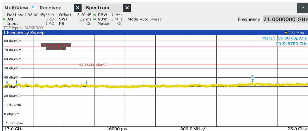
Figure 85: Chart of exploratory emissions measurement from 17 GHz to 25 GHz on middle channel
