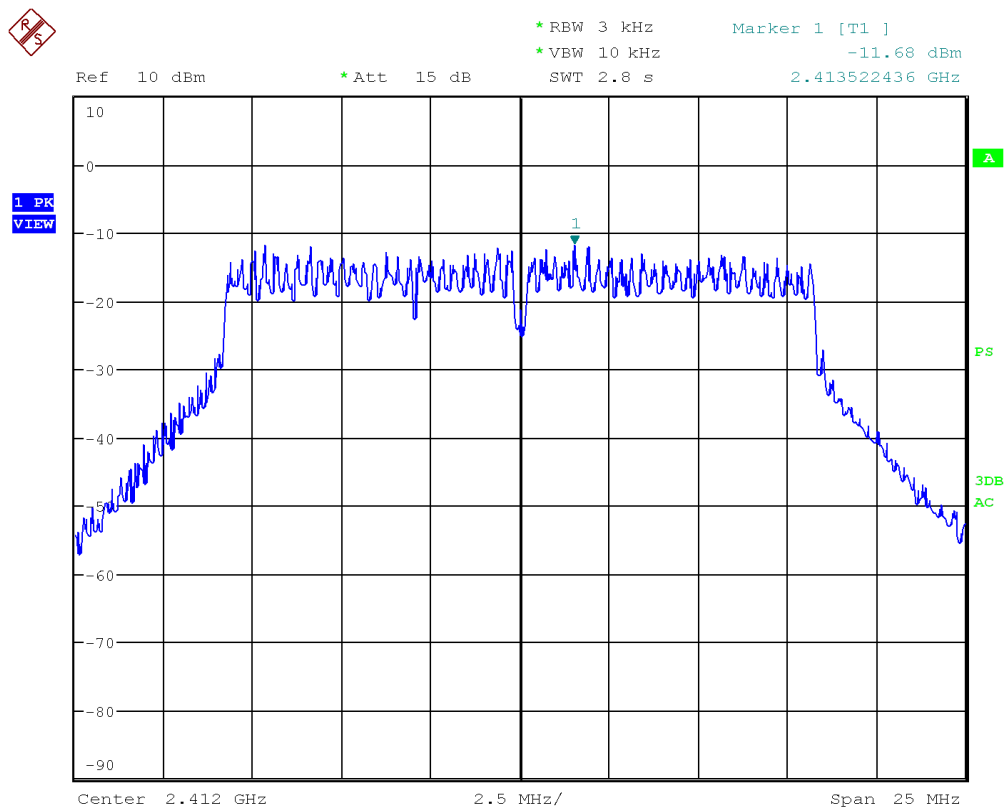
Figure 35: Chart of power spectral density on lowest channel in modulation IEEE 802.11 g
