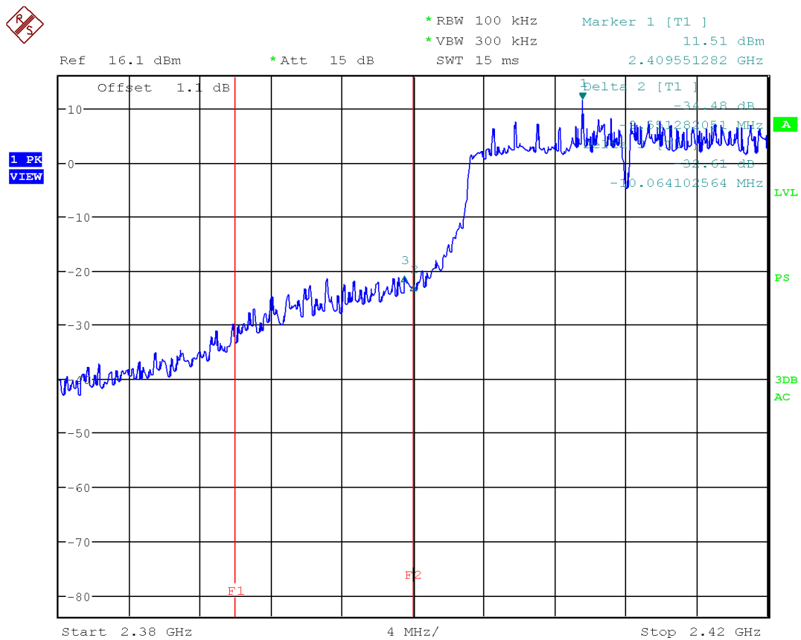
Figure 50: Chart of band-edge measurement on lowest channel in modulation IEEE 802.11 n (HT20)
