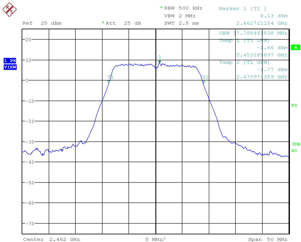
Figure 25: Chart of occupied bandwidth test on highest channel in modulation IEEE 802.11 g
