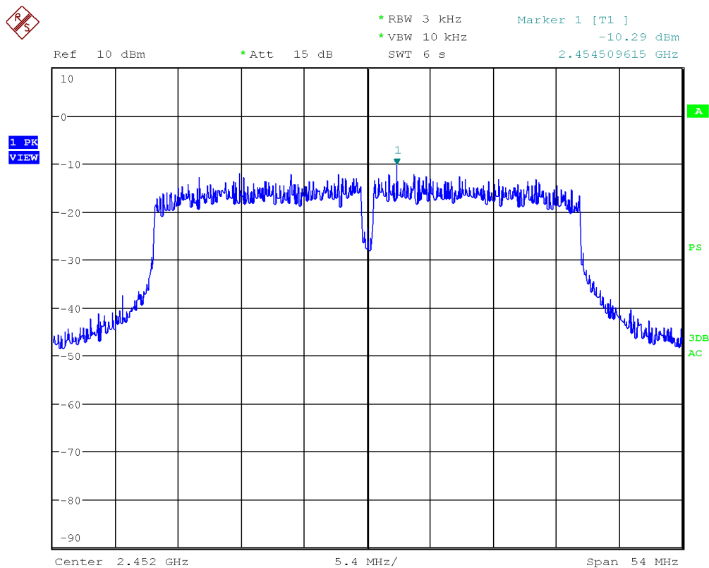
Figure 43: Chart of power spectral density on highest channel in modulation IEEE 802.11 n (HT40)
