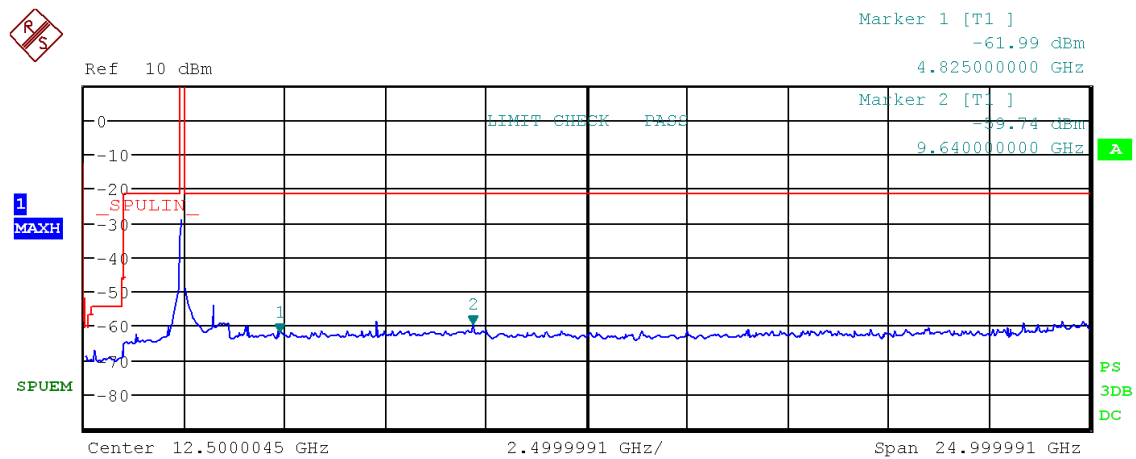
Figure 62: Chart of emissions test from 9 kHz to 25 GHz on lowest channel in modulation IEEE 802.11 g, PK-detector
