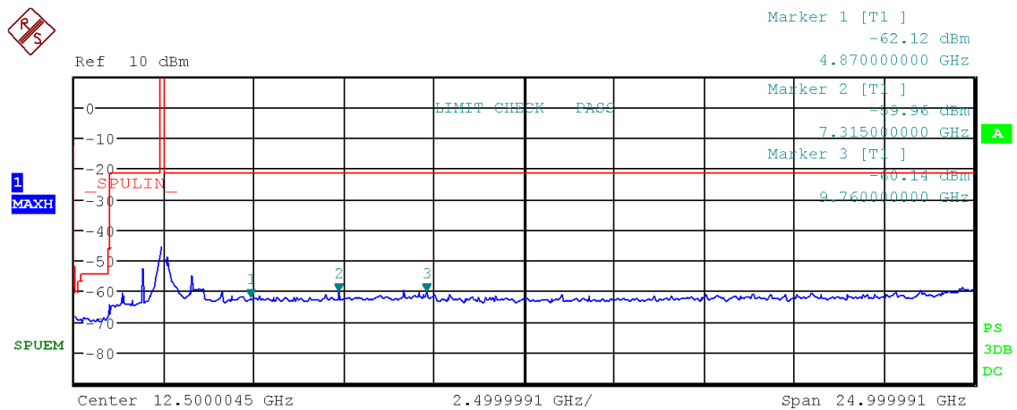
Figure 64: Chart of emissions test from 9 kHz to 25 GHz on middle channel in modulation IEEE 802.11 g, PK-detector
