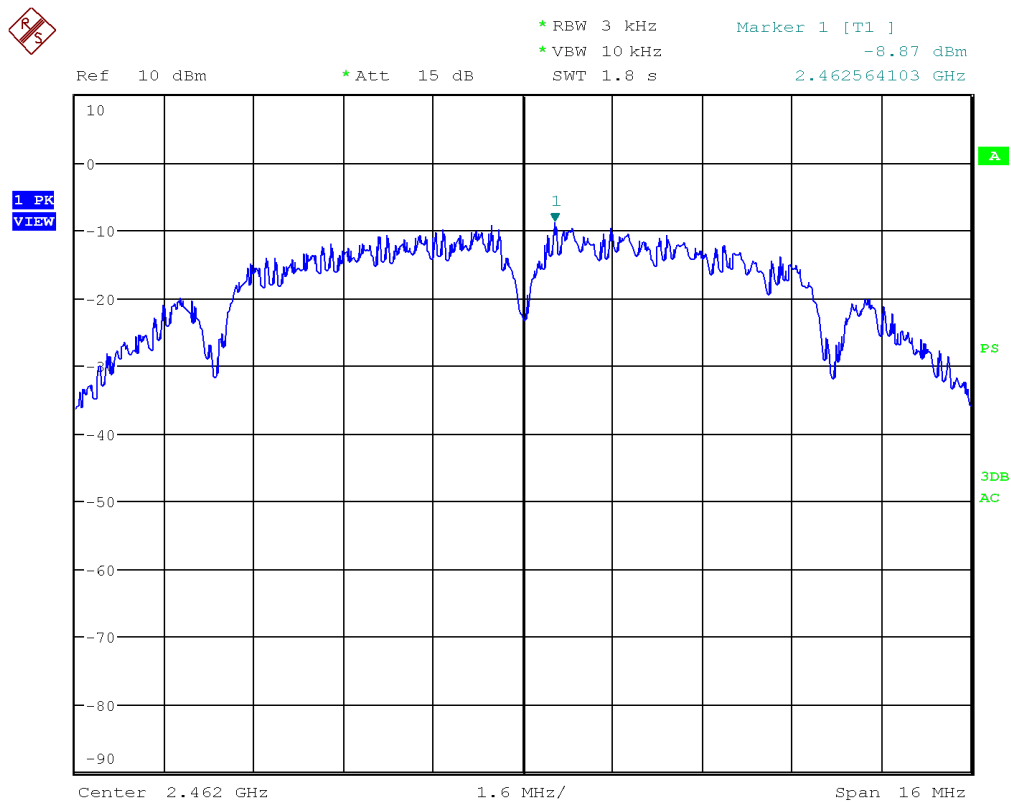
Figure 34: Chart of power spectral density on highest channel in modulation IEEE 802.11 b
