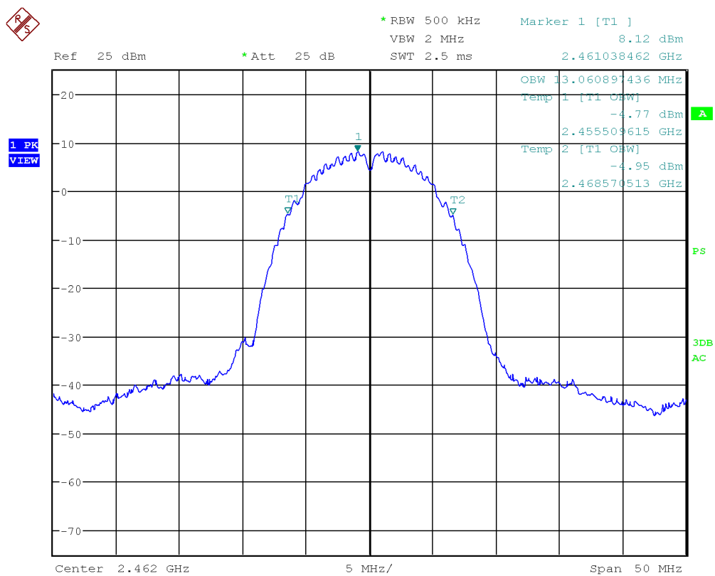
Figure 22: Chart of occupied bandwidth test on highest channel in modulation IEEE 802.11 b
