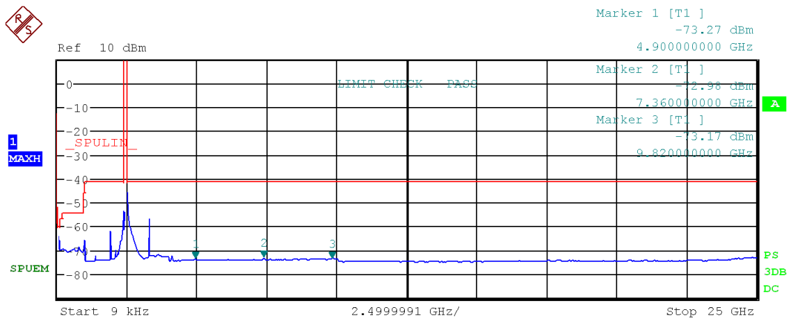
Figure 79: Chart of emissions test from 9 kHz to 25 GHz on highest channel in modulation IEEE 802.11 n (HT40), RMS-detector
