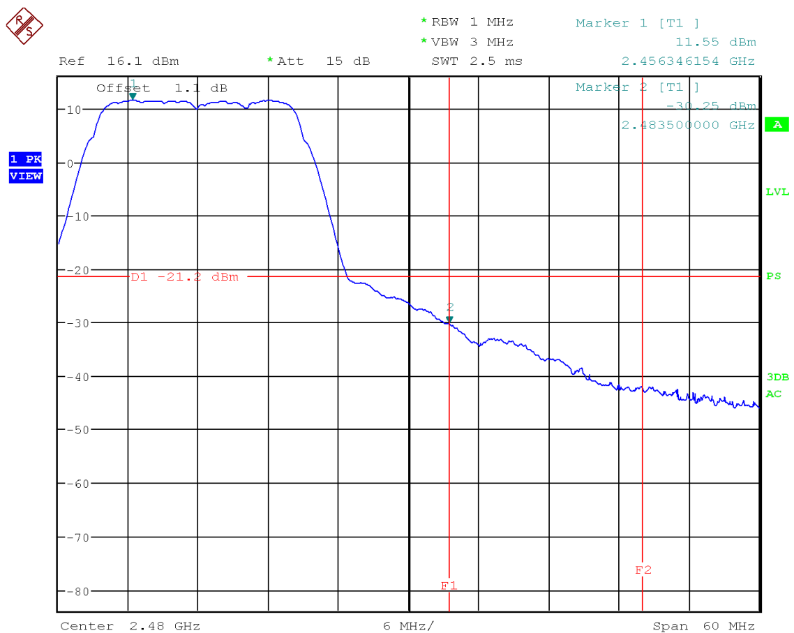
Figure 51: Chart of band-edge measurement on highest channel (PK) in modulation IEEE 802.11 n (HT20)
