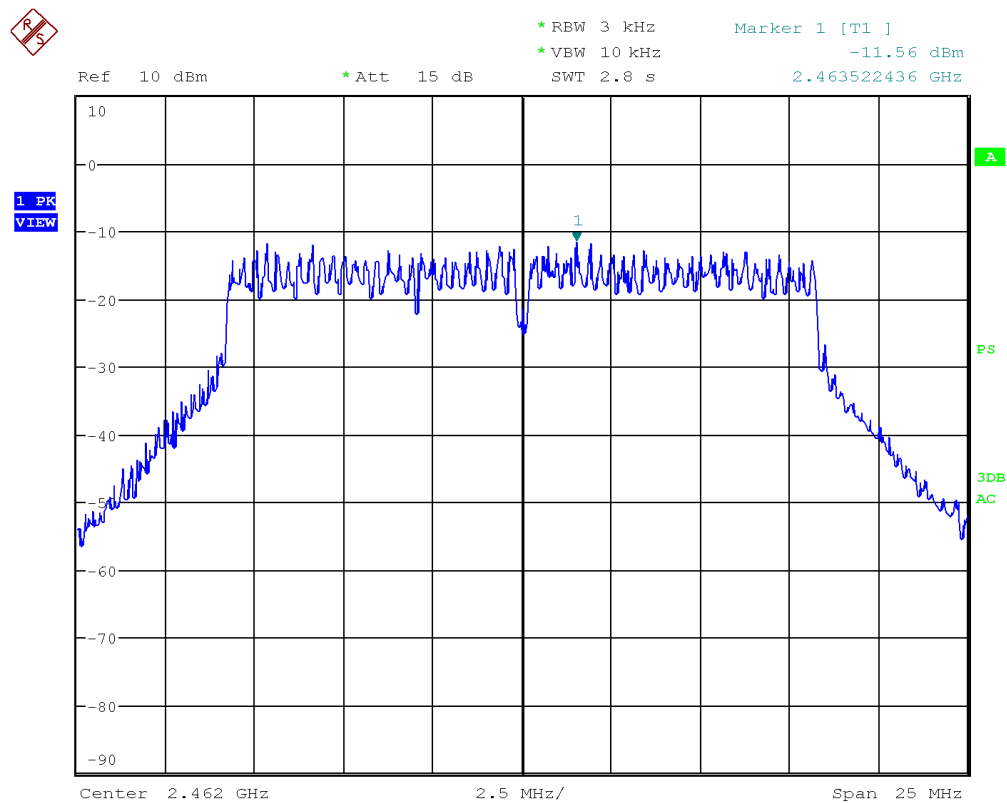
Figure 37: Chart of power spectral density on highest channel in modulation IEEE 802.11 g
