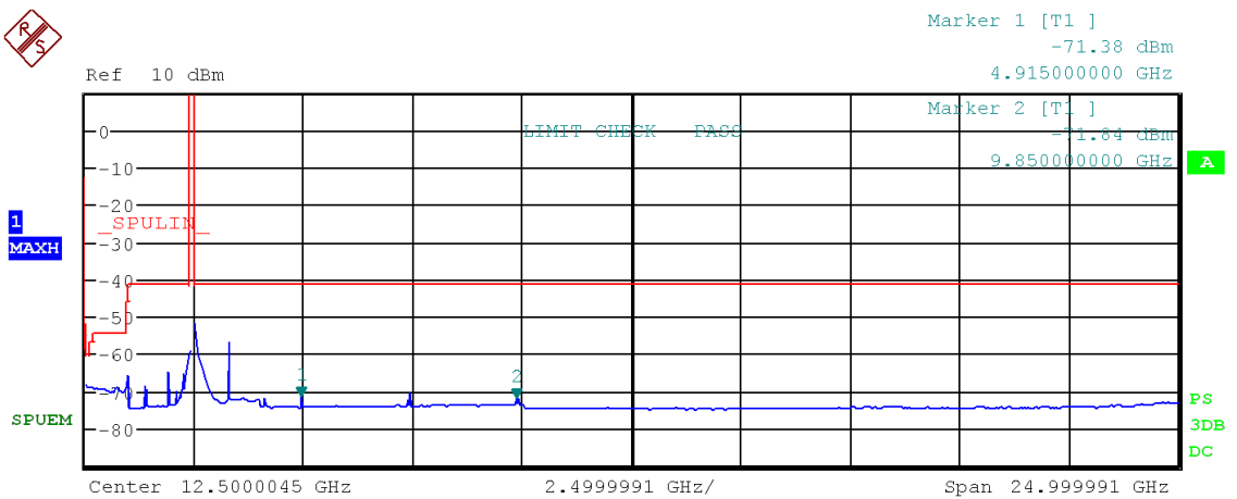
Figure 73: Chart of emissions test from 9 kHz to 25 GHz on highest channel in modulation IEEE 802.11 n (HT20), RMS-detector
