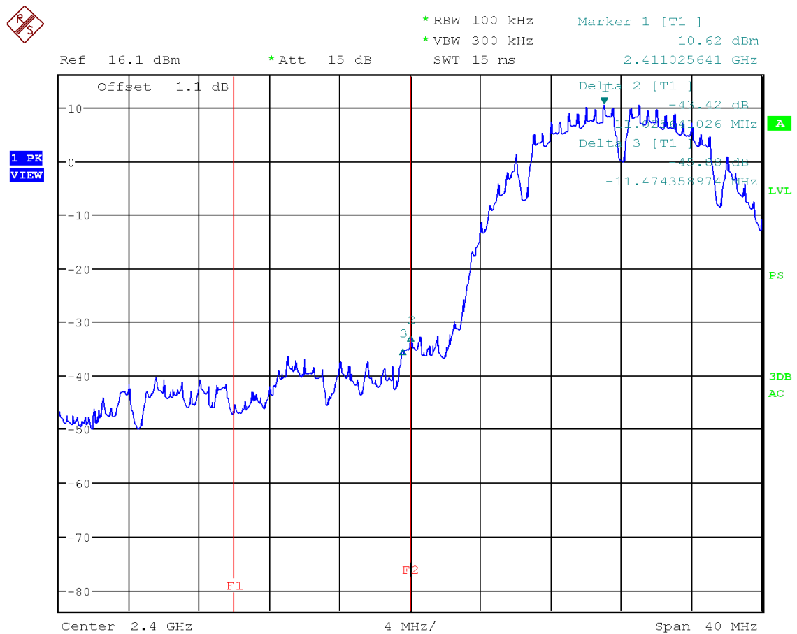
Figure 44: Chart of band-edge measurement on lowest channel in modulation IEEE 802.11 b
