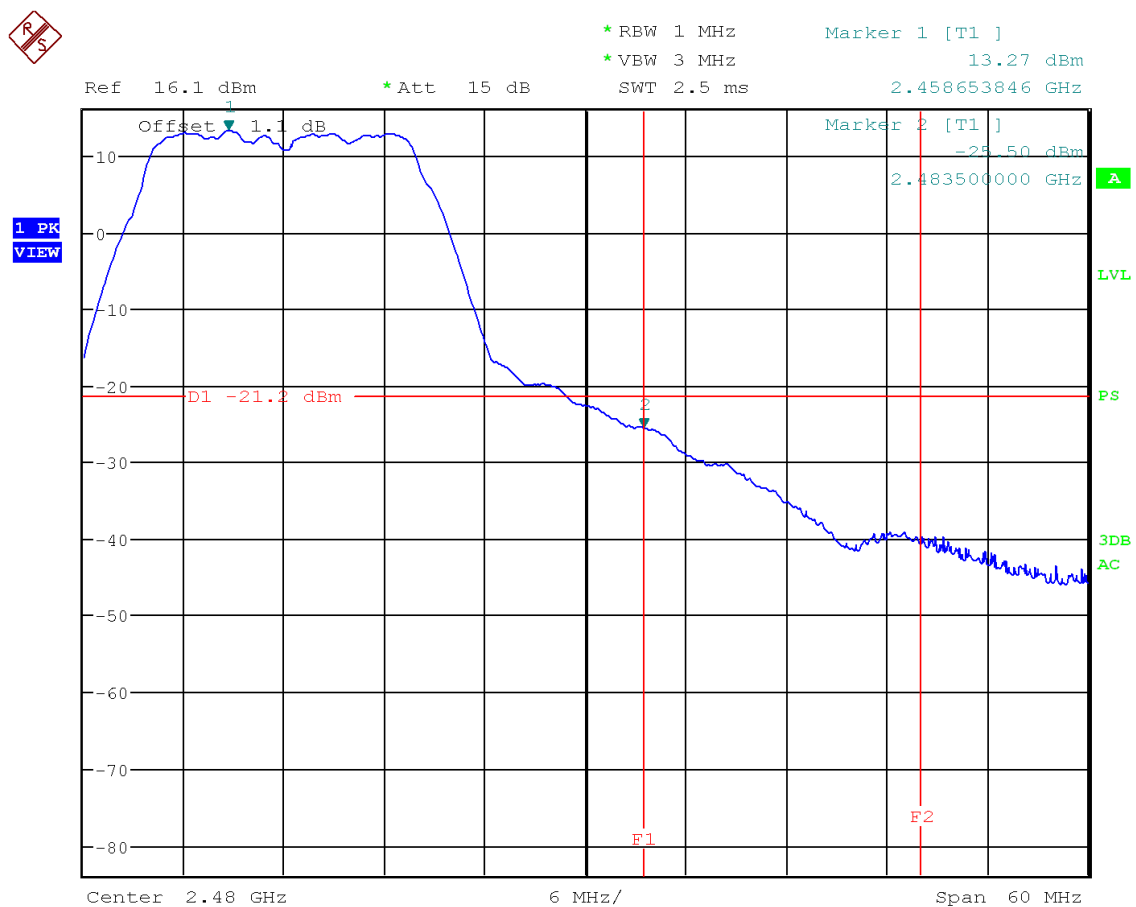
Figure 48: Chart of band-edge measurement on highest channel (PK) in modulation IEEE 802.11 g
