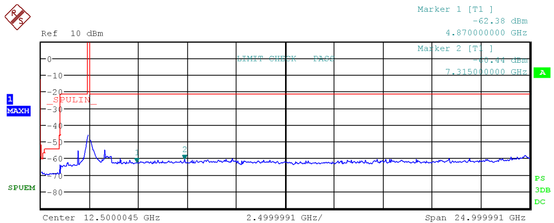
Figure 70: Chart of emissions test from 9 kHz to 25 GHz on middle channel in modulation IEEE 802.11 n (HT20), PK-detector
