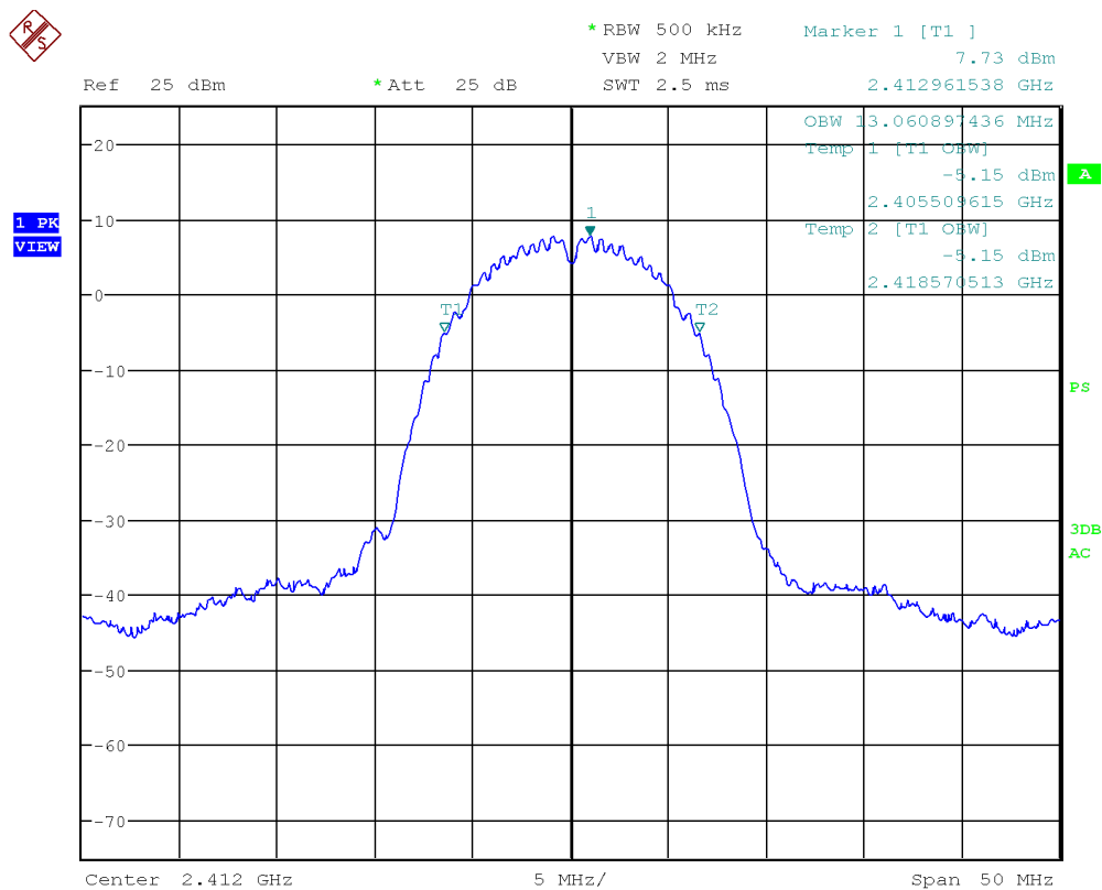
Figure 20: Chart of occupied bandwidth test on lowest channel in modulation IEEE 802.11 b
