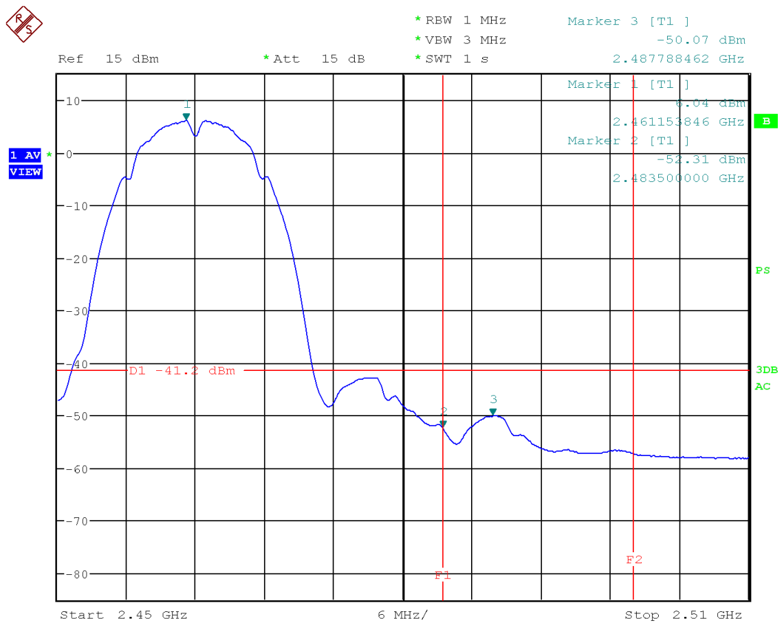
Figure 46: Chart of band-edge measurement on highest channel (AV) in modulation IEEE 802.11 b
