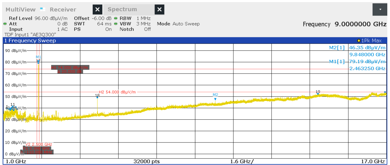
Figure 86: Chart of radiated emissions pre-measurement from 1 GHz to 17 GHz on highest channel, EUT position Y, antenna polarization vertical
