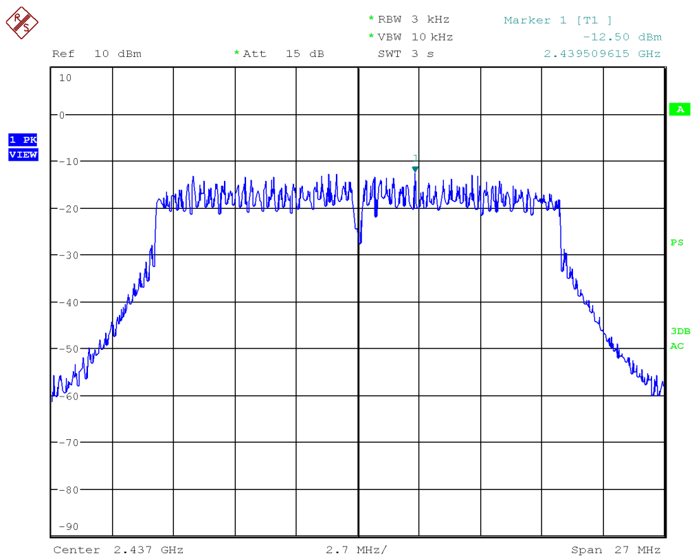
Figure 39: Chart of power spectral density on middle channel in modulation IEEE 802.11 n (HT20)
