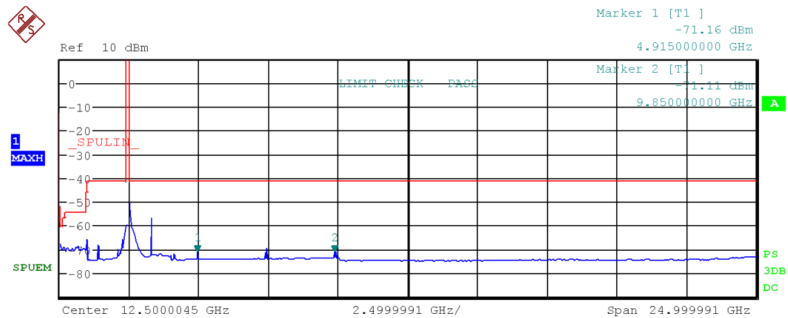
Figure 67: Chart of emissions test from 9 kHz to 25 GHz on highest channel in modulation IEEE 802.11 g, RMS-detector
