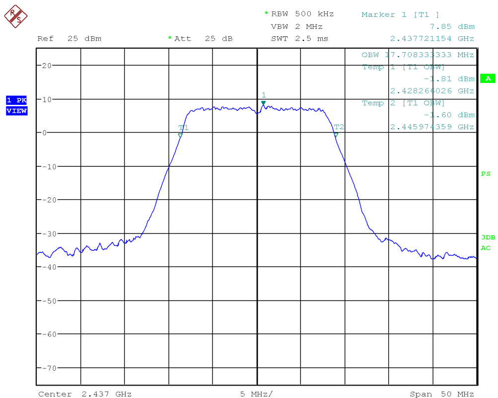
Figure 24: Chart of occupied bandwidth test on middle channel in modulation IEEE 802.11 g
