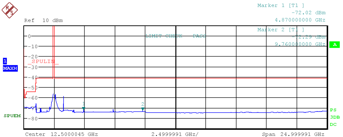
Figure 71: Chart of emissions test from 9 kHz to 25 GHz on middle channel in modulation IEEE 802.11 n (HT20), RMS-detector
