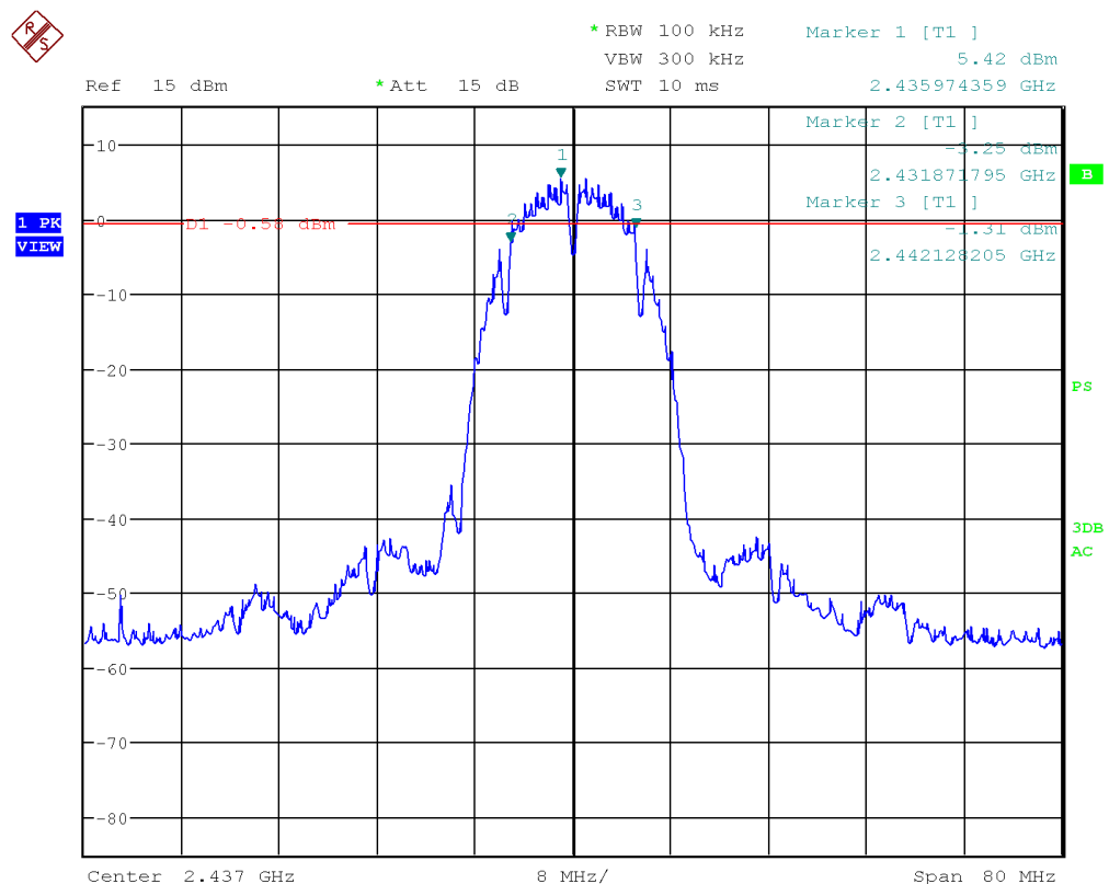
Figure 9: Chart of 6 dB bandwidth test on middle channel in modulation IEEE 802.11 b
