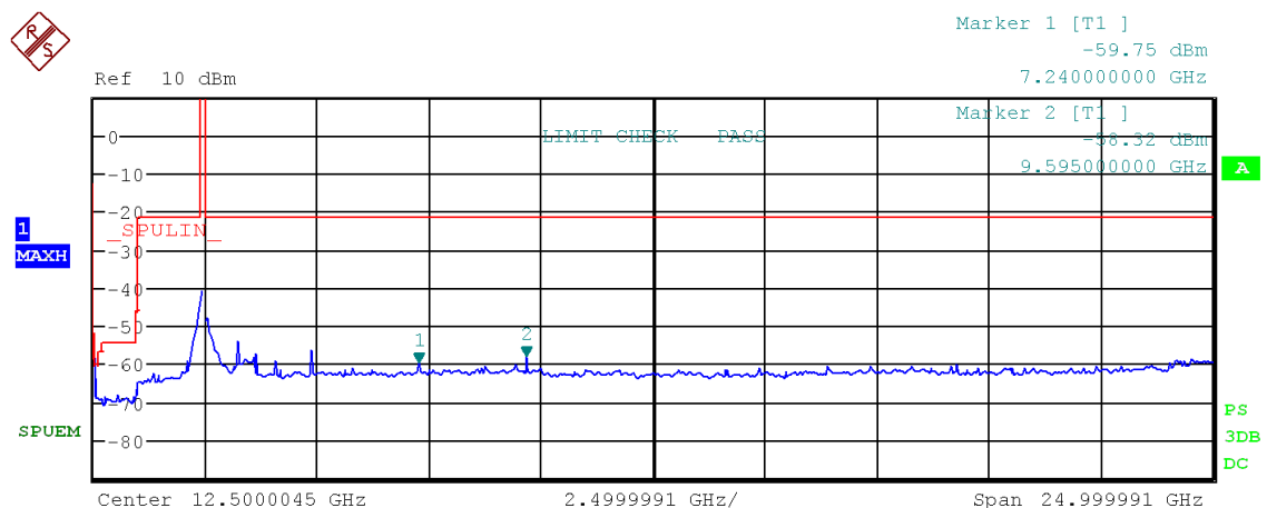
Figure 56: Chart of emissions test from 9 kHz to 25 GHz on lowest channel in modulation IEEE 802.11 b, PK-detector
