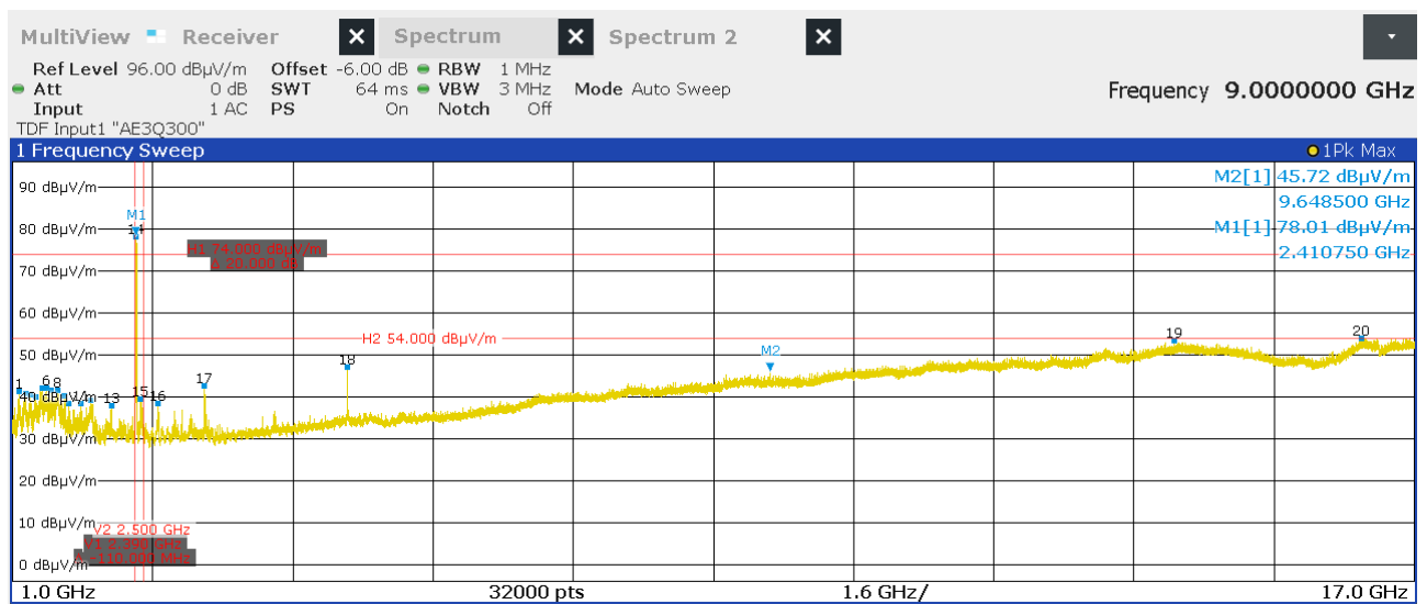
Figure 82: Chart of radiated emissions pre-measurement from 1 GHz to 17 GHz on lowest channel, EUT position Y, antenna polarization vertical
