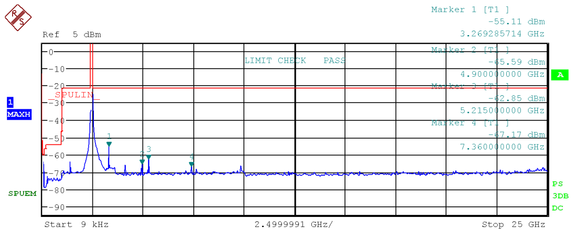
Figure 78: Chart of emissions test from 9 kHz to 25 GHz on highest channel in modulation IEEE 802.11 n (HT40), PK-detector
