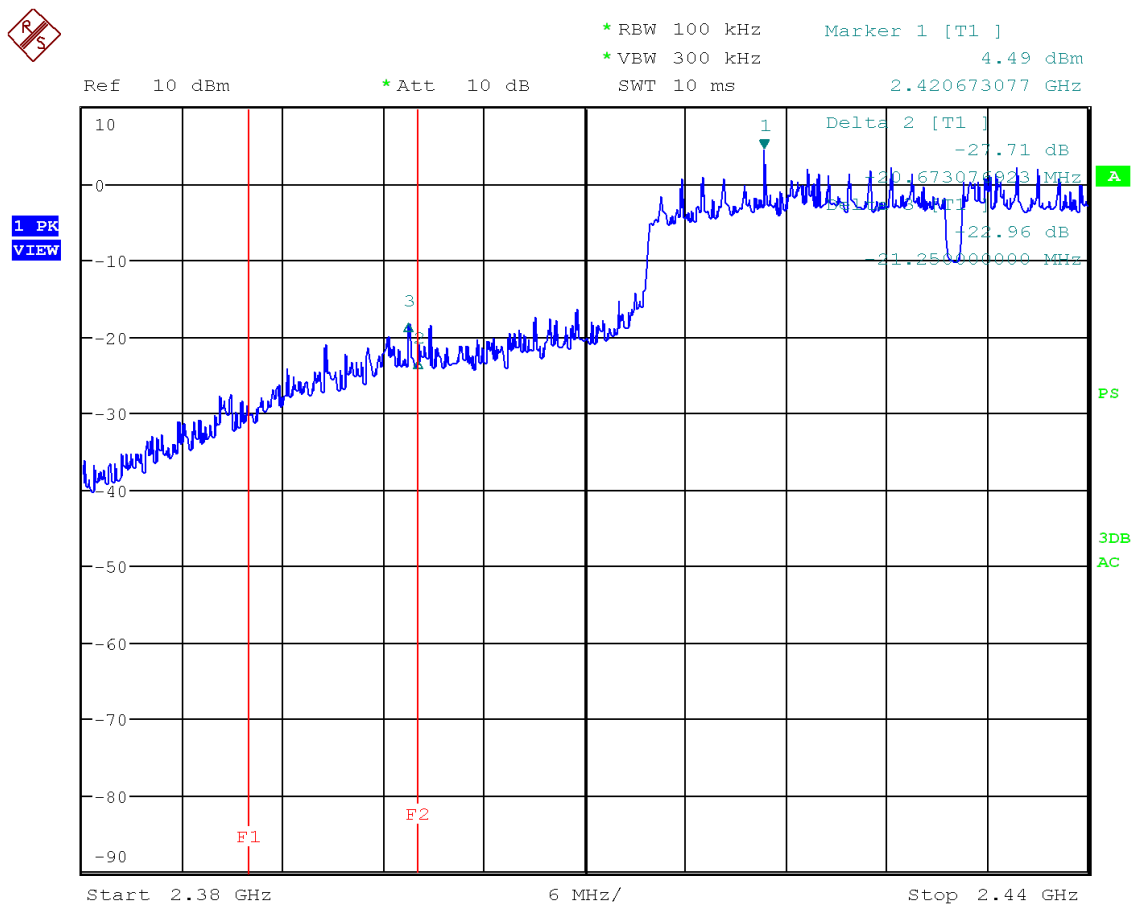
Figure 53: Chart of band-edge measurement on lowest channel in modulation IEEE 802.11 n (HT40)
