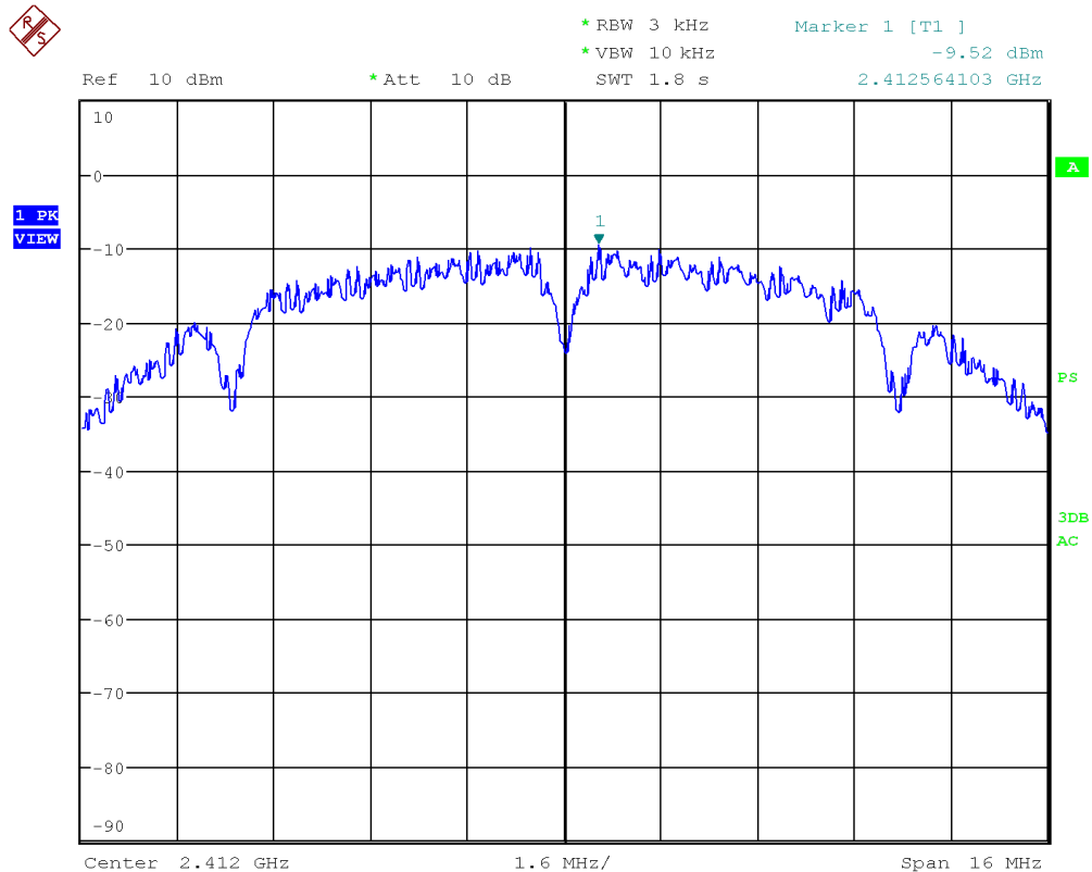
Figure 32: Chart of power spectral density on lowest channel in modulation IEEE 802.11 b
