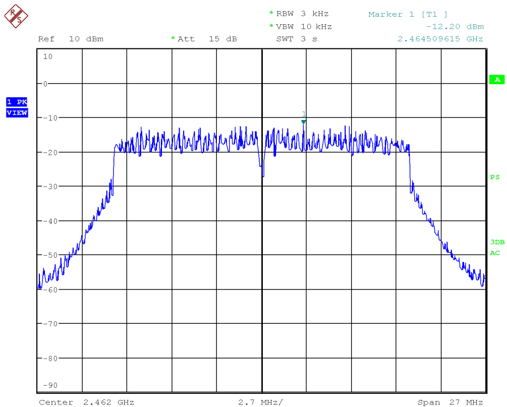
Figure 40: Chart of power spectral density on highest channel in modulation IEEE 802.11 n (HT20)
