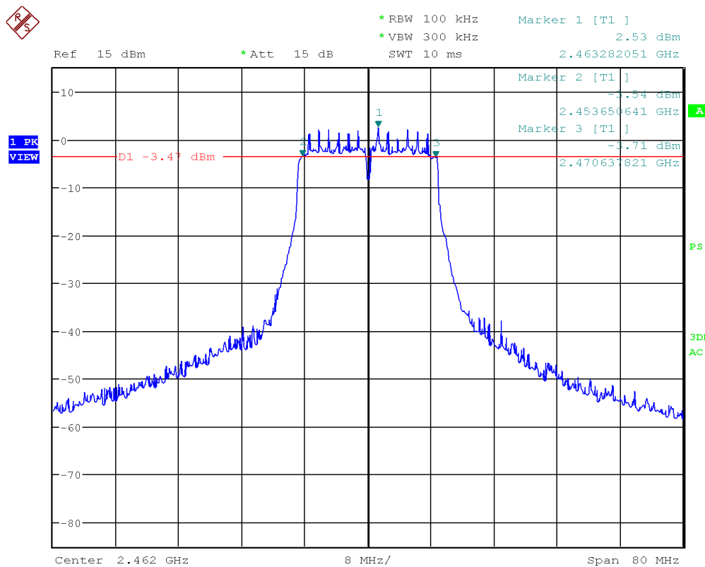
Figure 16: Chart of 6 dB bandwidth test on highest channel in modulation IEEE 802.11 n (HT20)
