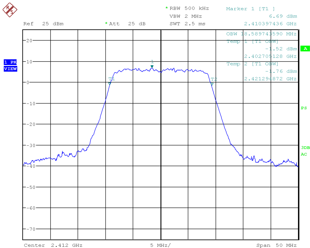
Figure 26: Chart of occupied bandwidth test on lowest channel in modulation IEEE 802.11 n (HT20)
