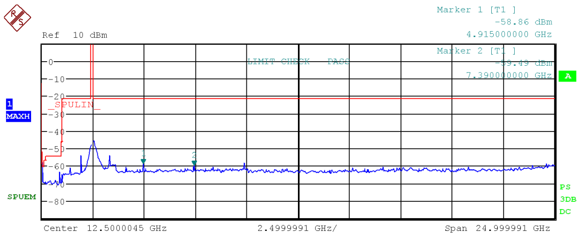
Figure 60: Chart of emissions test from 9 kHz to 25 GHz on highest channel in modulation IEEE 802.11 b, PK-detector
