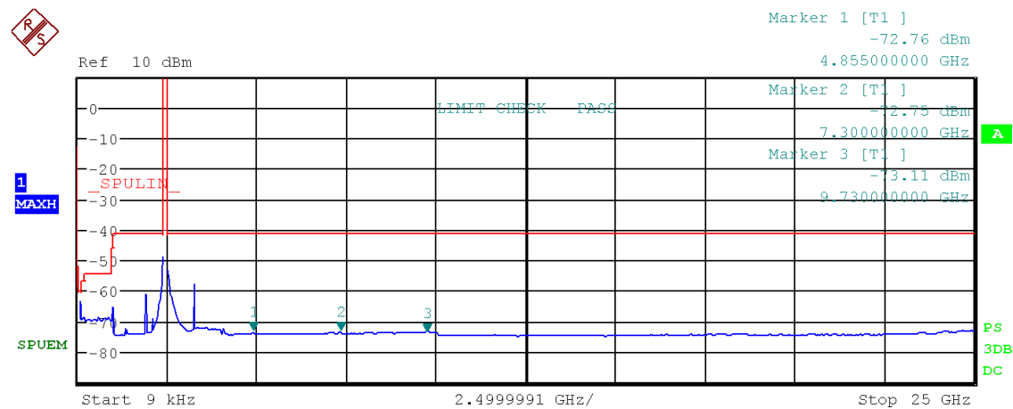
Figure 75: Chart of emissions test from 9 kHz to 25 GHz on lowest channel in modulation IEEE 802.11 n (HT40), RMS-detector
