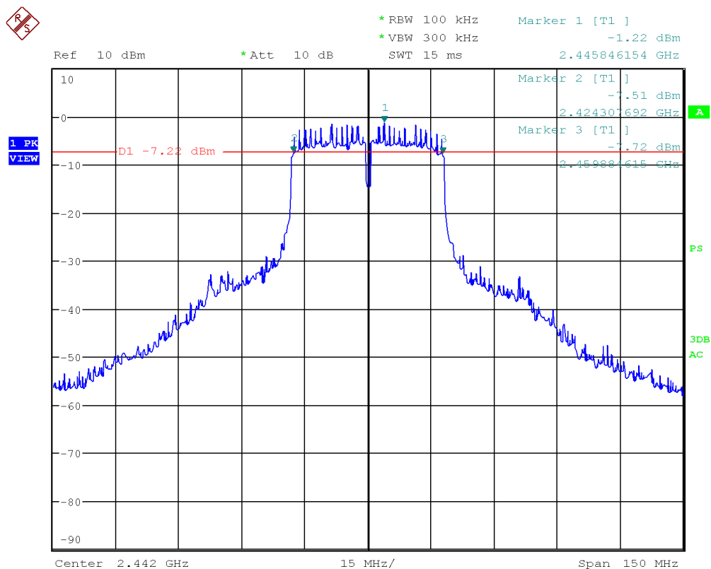
Figure 18: Chart of 6 dB bandwidth test on middle channel in modulation IEEE 802.11 n (HT40)
