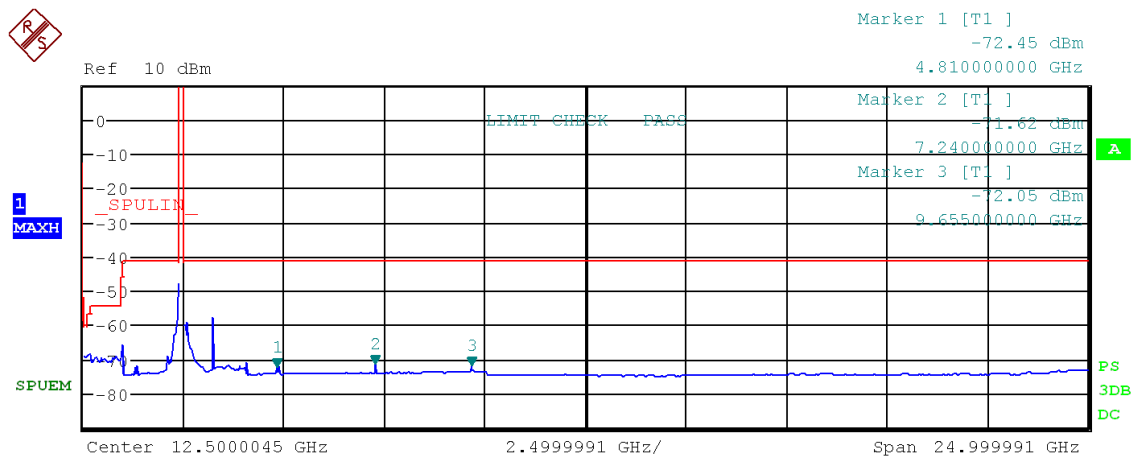
Figure 69: Chart of emissions test from 9 kHz to 25 GHz on lowest channel in modulation IEEE 802.11 n (HT20), RMS-detector
