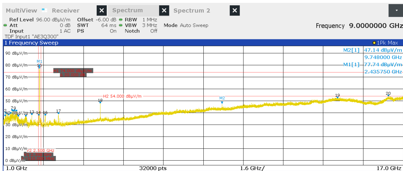
Figure 84: Chart of radiated emissions pre-measurement from 1 GHz to 17 GHz on middle channel, EUT position Y, antenna polarization vertical
