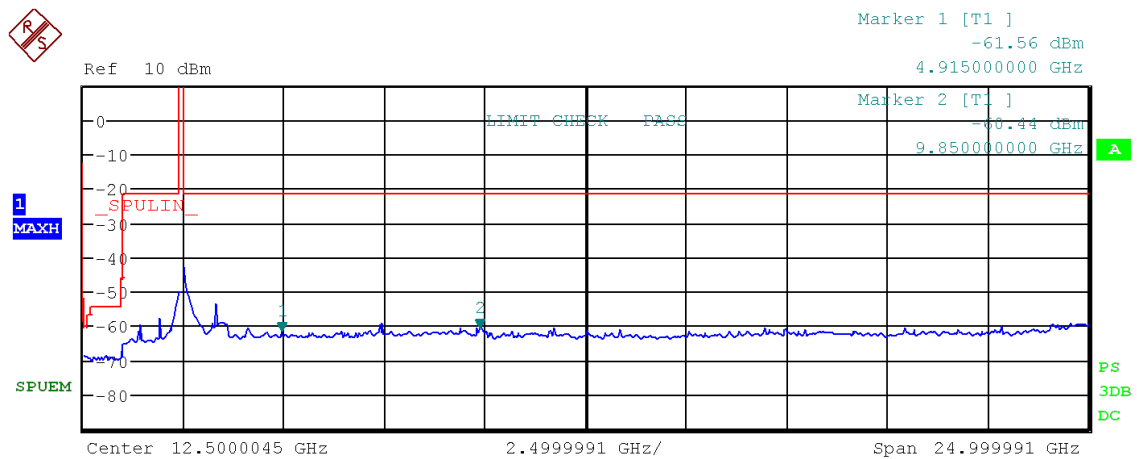
Figure 72: Chart of emissions test from 9 kHz to 25 GHz on highest channel in modulation IEEE 802.11 n (HT20), PK-detector
