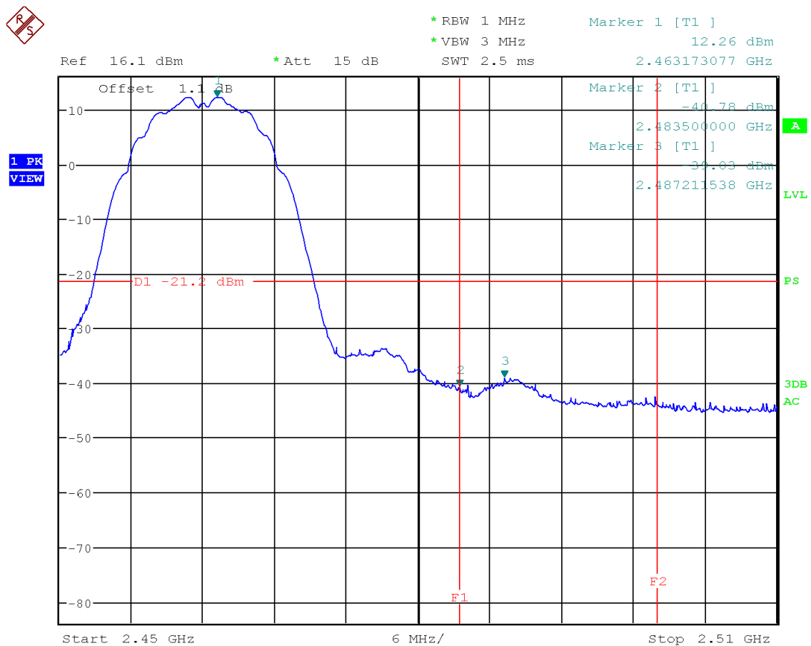
Figure 45: Chart of band-edge measurement on highest channel (PK) in modulation IEEE 802.11 b
