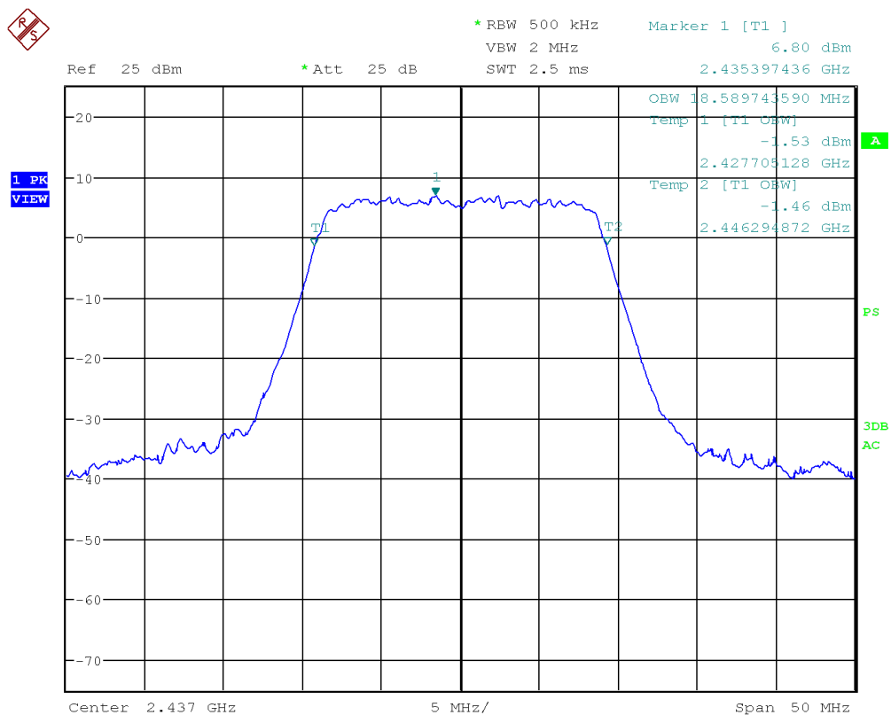
Figure 27: Chart of occupied bandwidth test on middle channel in modulation IEEE 802.11 n (HT20)
