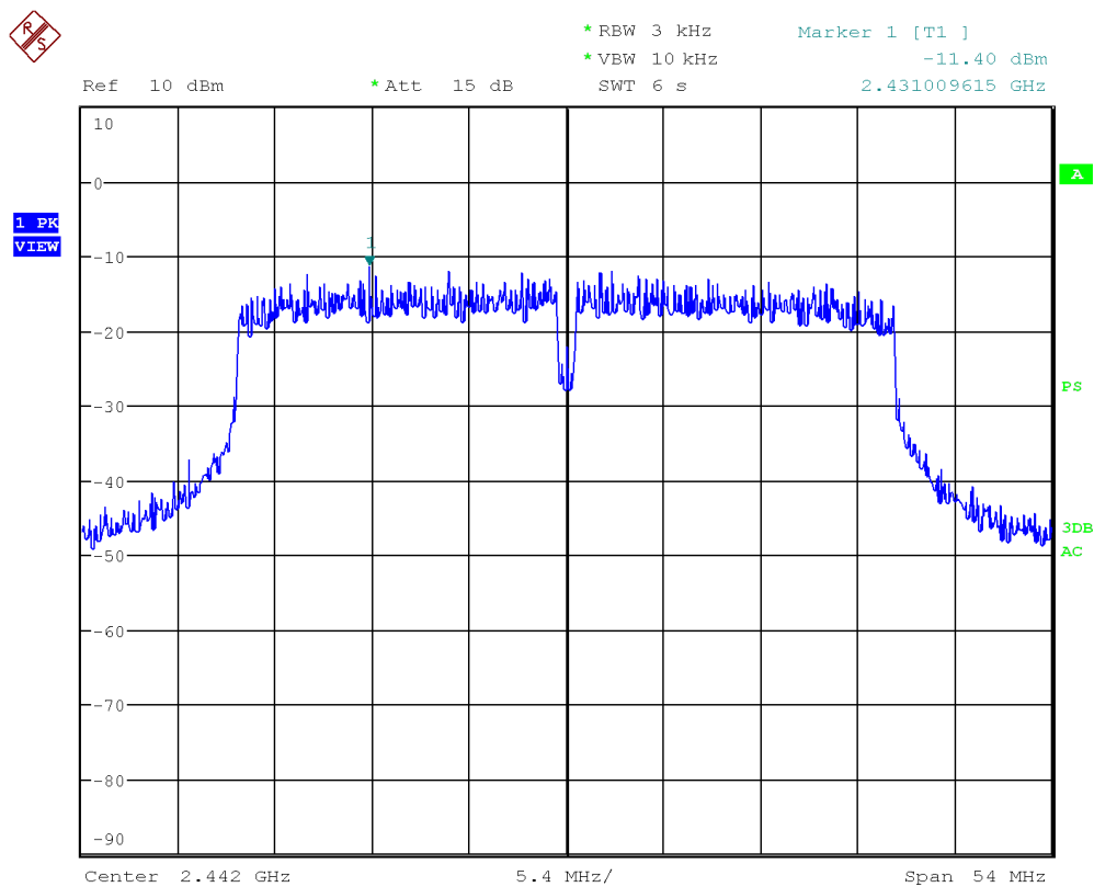
Figure 42: Chart of power spectral density on middle channel in modulation IEEE 802.11 n (HT40)
