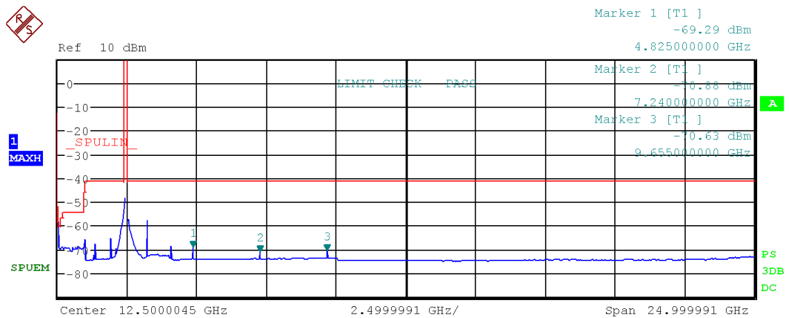
Figure 57: Chart of emissions test from 9 kHz to 25 GHz on lowest channel in modulation IEEE 802.11 b, RMS-detector
