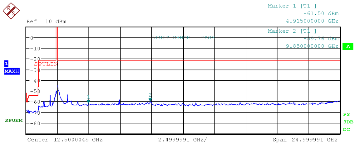
Figure 66: Chart of emissions test from 9 kHz to 25 GHz on highest channel in modulation IEEE 802.11 g, PK-detector
