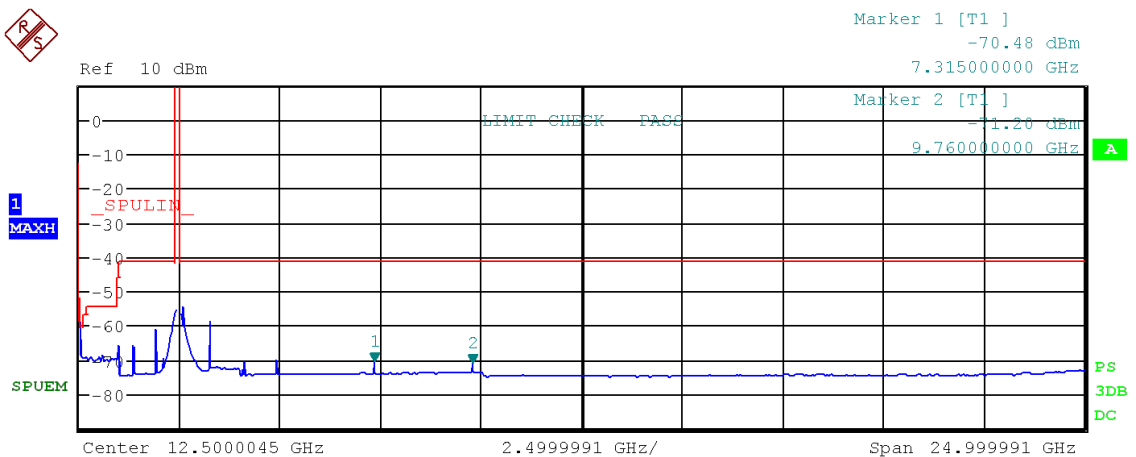
Figure 59: Chart of emissions test from 9 kHz to 25 GHz on middle channel in modulation IEEE 802.11 b, RMS-detector
