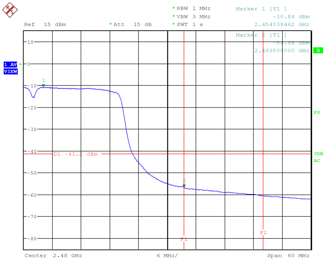
Figure 55: Chart of band-edge measurement on highest channel (AV) in modulation IEEE 802.11 n (HT40)
