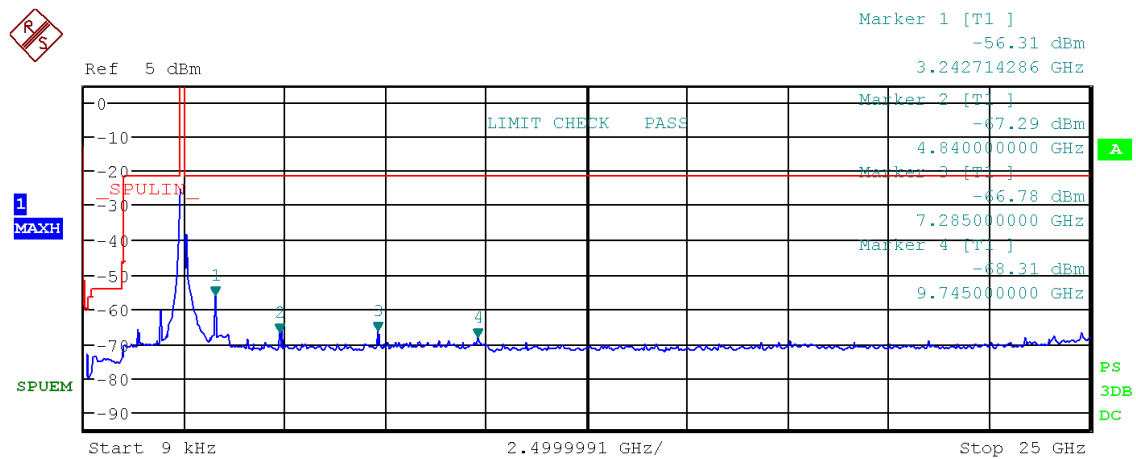
Figure 74: Chart of emissions test from 9 kHz to 25 GHz on lowest channel in modulation IEEE 802.11 n (HT40), PK-detector
