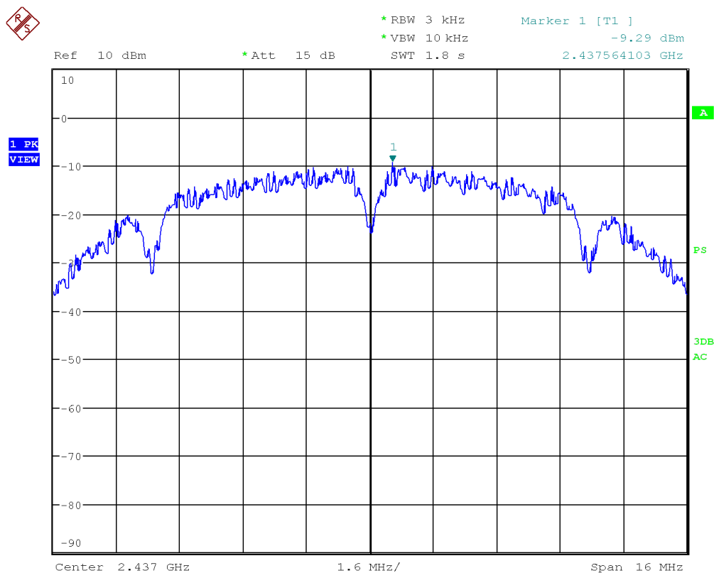
Figure 33: Chart of power spectral density on middle channel in modulation IEEE 802.11 b
