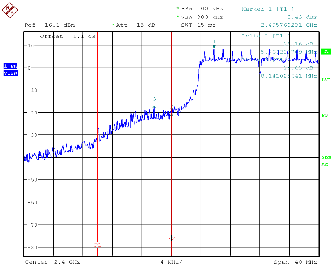
Figure 47: Chart of band-edge measurement on lowest channel in modulation IEEE 802.11 g
