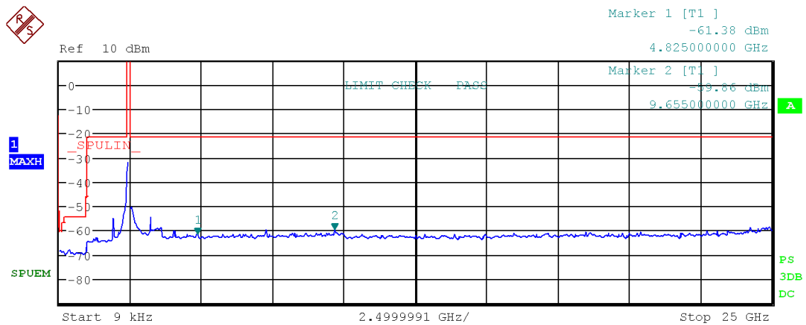
Figure 68: Chart of emissions test from 9 kHz to 25 GHz on lowest channel in modulation IEEE 802.11 n (HT20), PK-detector
