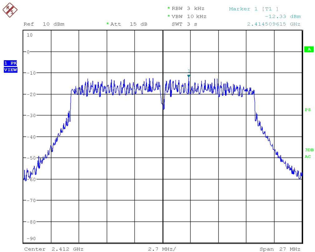
Figure 38: Chart of power spectral density on lowest channel in modulation IEEE 802.11 n (HT20)
