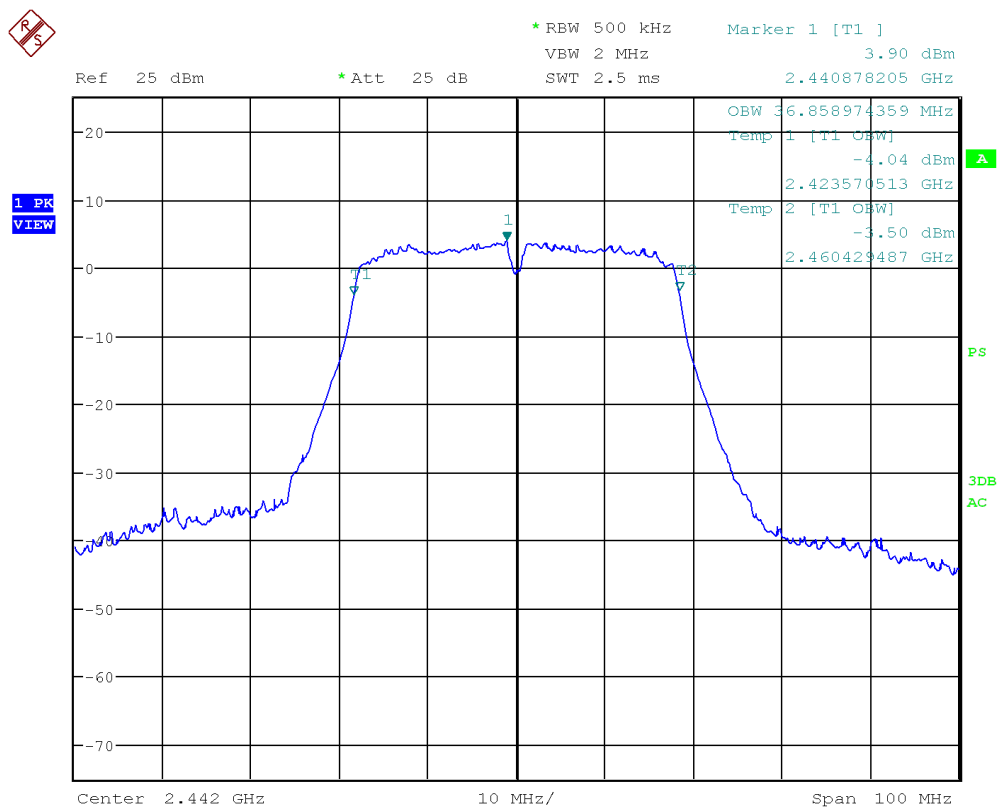
Figure 30: Chart of occupied bandwidth test on middle channel in modulation IEEE 802.11 n (HT40)
