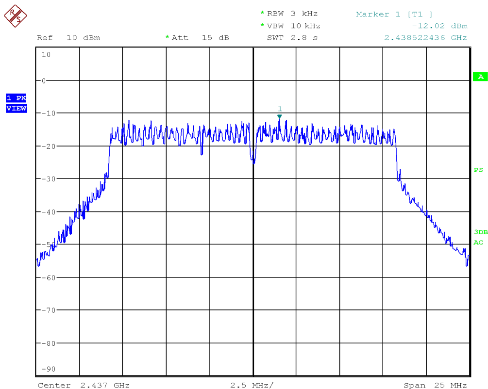
Figure 36: Chart of power spectral density on middle channel in modulation IEEE 802.11 g
