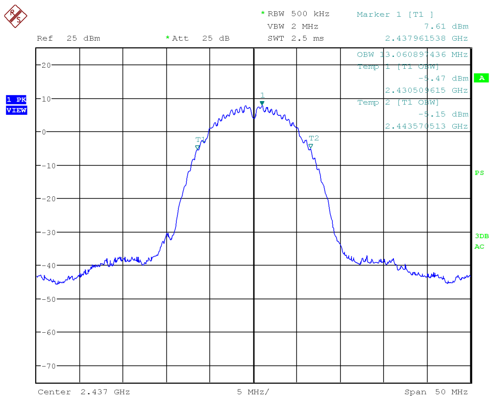
Figure 21: Chart of occupied bandwidth test on middle channel in modulation IEEE 802.11 b
