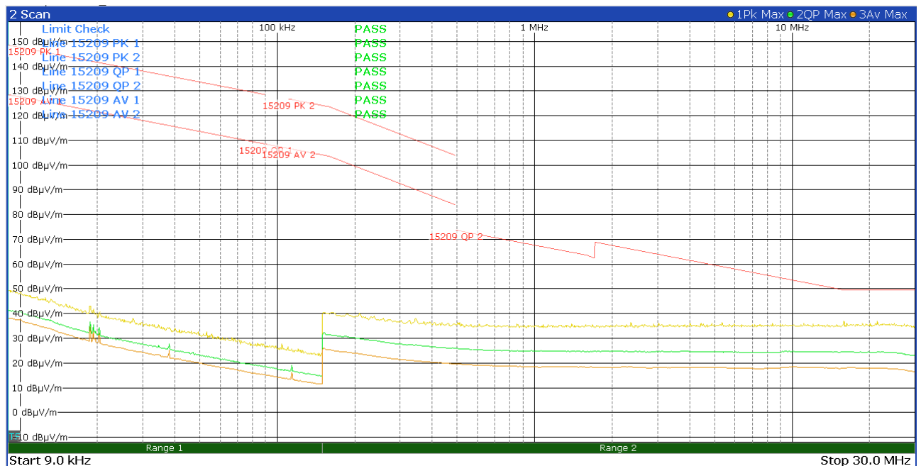
Figure 80: Chart of emissions test below 30 MHz on highest channel, EUT position Z, antenna parallel to the EUT
