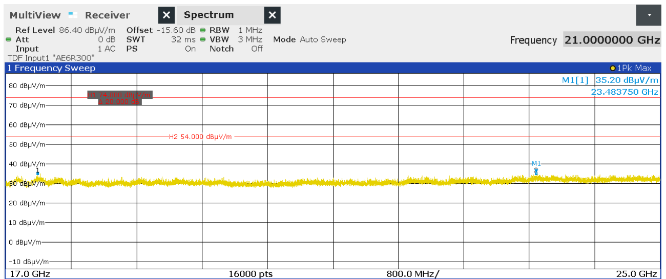
Figure 87: Chart of exploratory emission test from 17 GHz to 25 GHz on highest channel at 0.5 m
