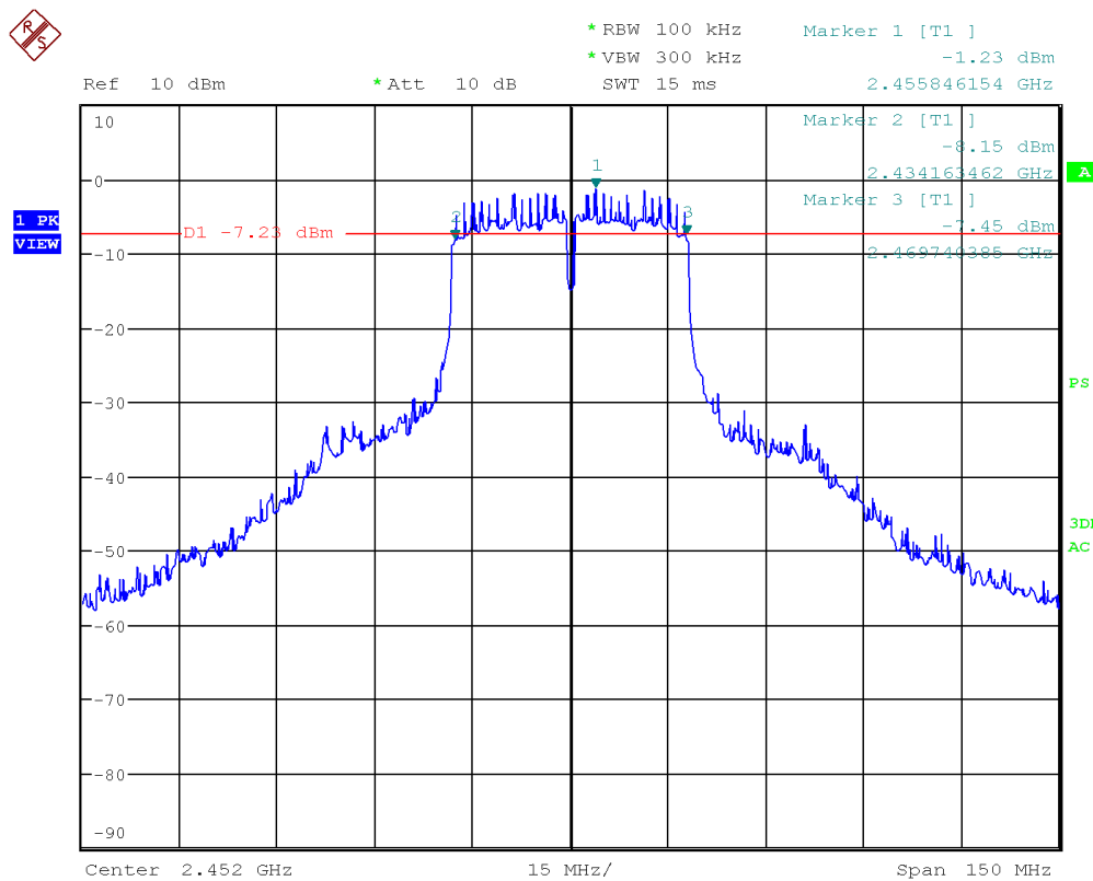
Figure 19: Chart of 6 dB bandwidth test on highest channel in modulation IEEE 802.11 n (HT40)
