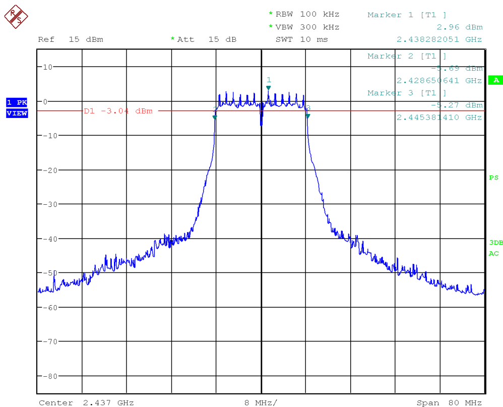
Figure 12: Chart of 6 dB bandwidth test on middle channel in modulation IEEE 802.11 g
