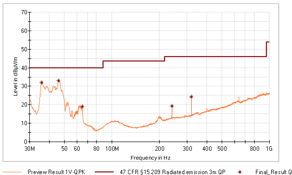
Figure 81: Chart of emissions test from 30 MHz to 1 GHz on lowest channel, EUT position Z, antenna polarization vertical
