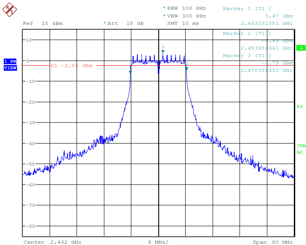
Figure 13: Chart of 6 dB bandwidth test on highest channel in modulation IEEE 802.11 g
