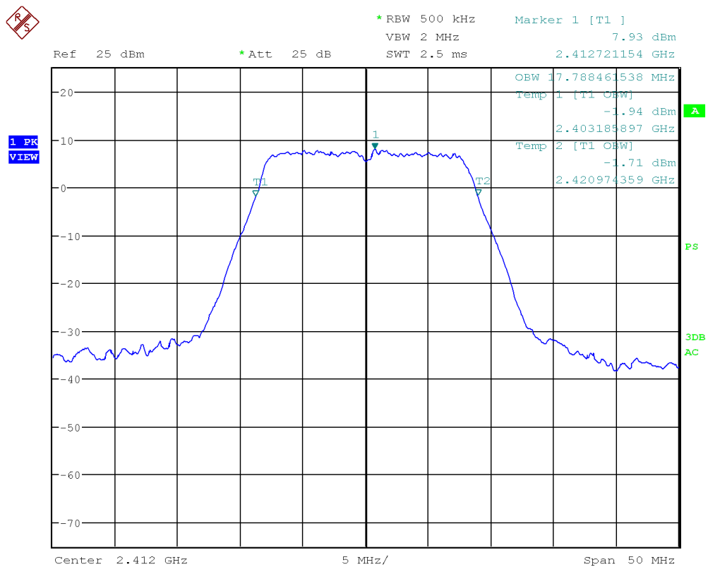
Figure 23: Chart of occupied bandwidth test on lowest channel in modulation IEEE 802.11 g
