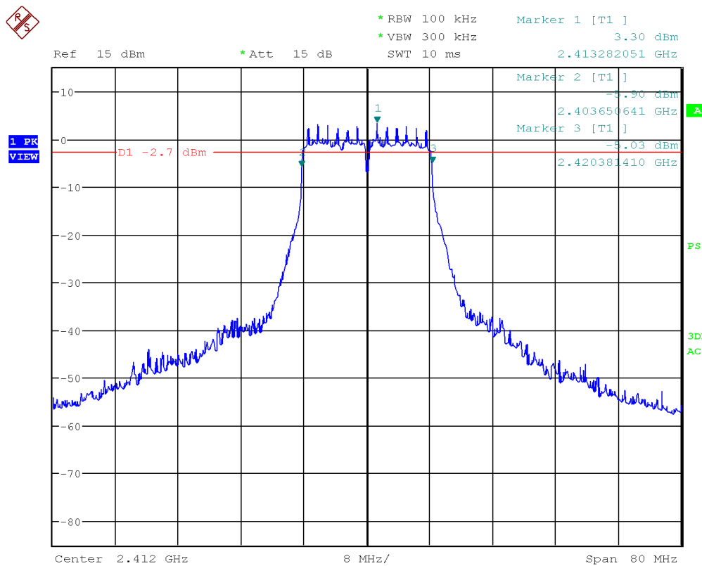
Figure 11: Chart of 6 dB bandwidth test on lowest channel in modulation IEEE 802.11 g
