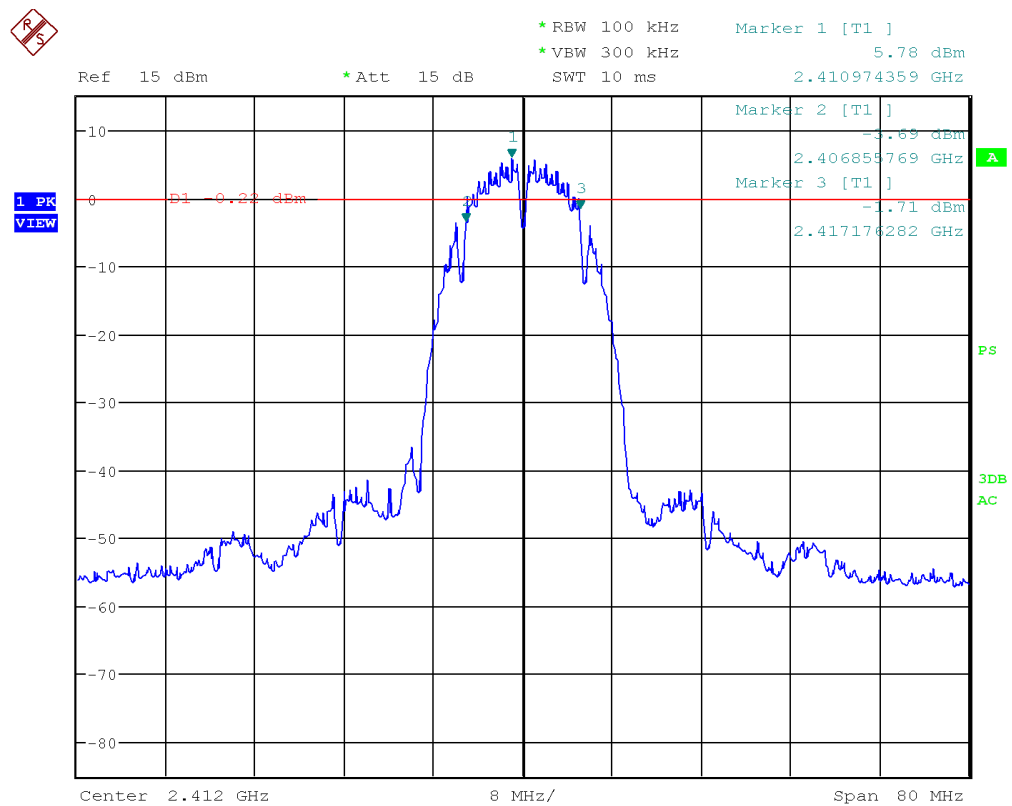
Figure 8: Chart of 6 dB bandwidth test on lowest channel in modulation IEEE 802.11 b
