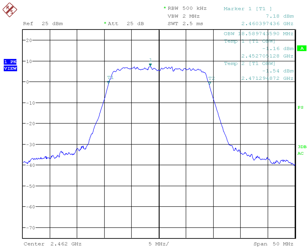
Figure 28: Chart of occupied bandwidth test on highest channel in modulation IEEE 802.11 n (HT20)
