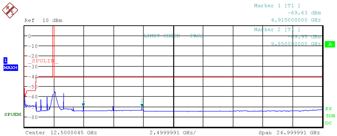
Figure 61: Chart of emissions test from 9 kHz to 25 GHz on highest channel in modulation IEEE 802.11 b, RMS-detector
