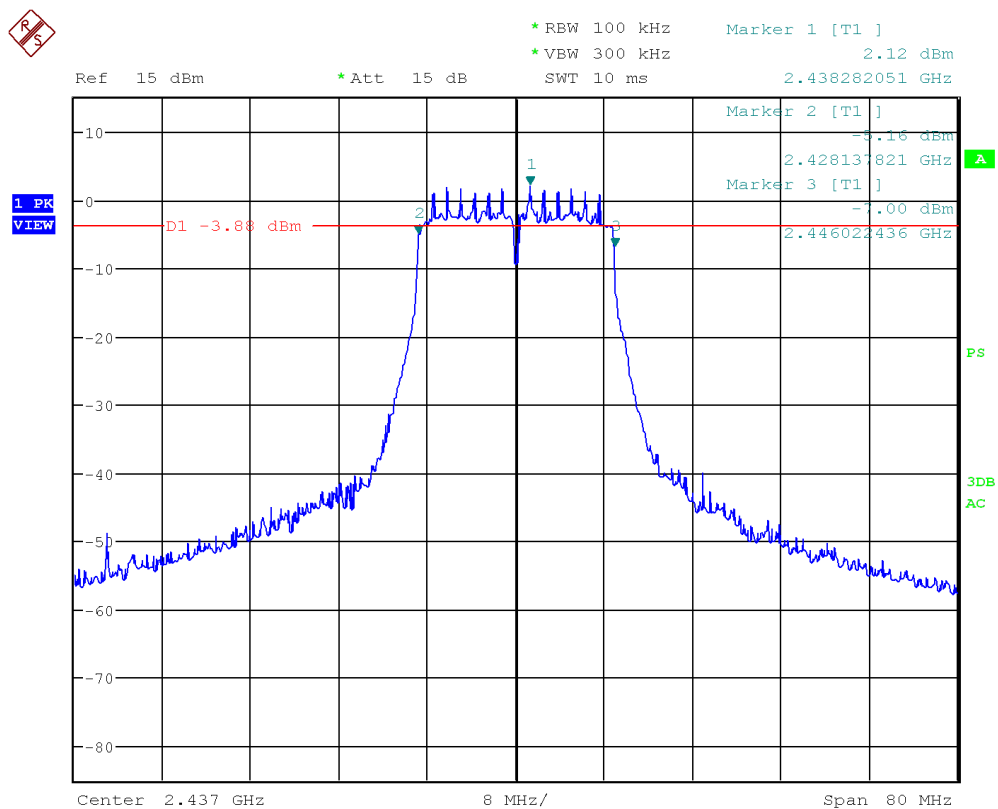
Figure 15: Chart of 6 dB bandwidth test on middle channel in modulation IEEE 802.11 n (HT20)
