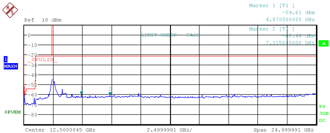
Figure 58: Chart of emissions test from 9 kHz to 25 GHz on middle channel in modulation IEEE 802.11 b, PK-detector
