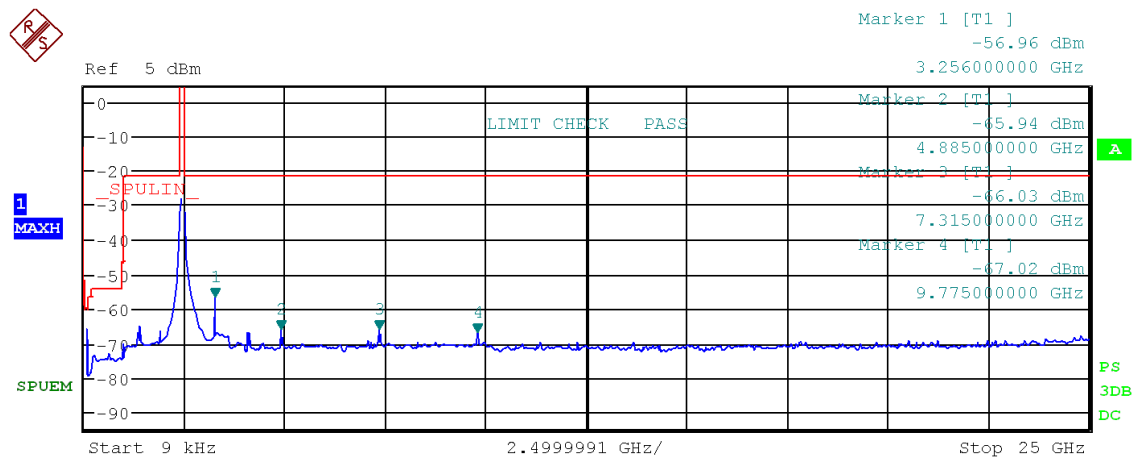
Figure 76: Chart of emissions test from 9 kHz to 25 GHz on middle channel in modulation IEEE 802.11 n (HT40), PK-detector
