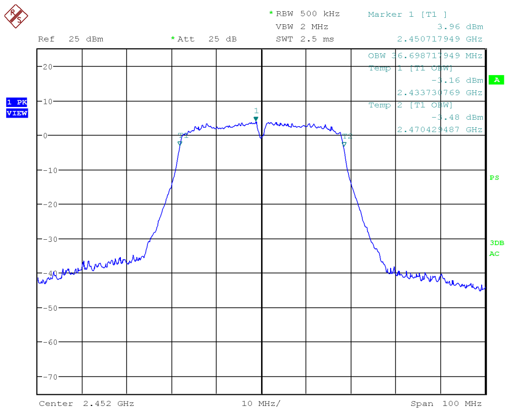
Figure 31: Chart of occupied bandwidth test on highest channel in modulation IEEE 802.11 n (HT40)
