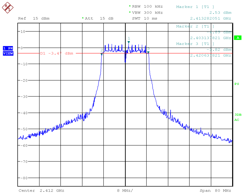
Figure 14: Chart of 6 dB bandwidth test on lowest channel in modulation IEEE 802.11 n (HT20)
