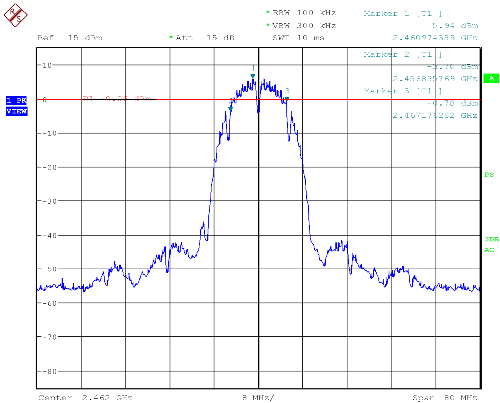
Figure 10: Chart of 6 dB bandwidth test on highest channel in modulation IEEE 802.11 b
