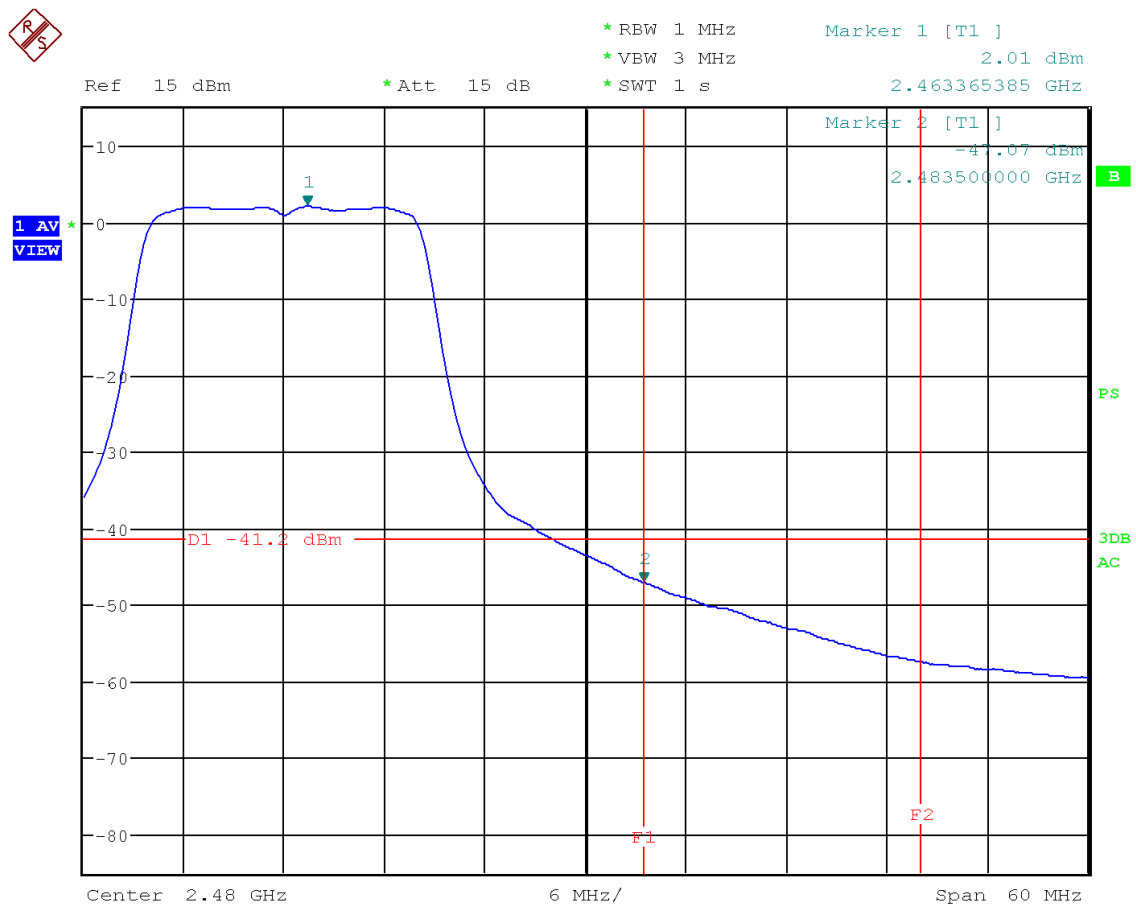
Figure 49: Chart of band-edge measurement on highest channel (AV) in modulation IEEE 802.11 g
