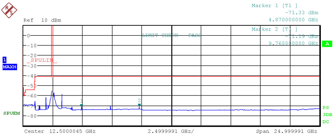
Figure 65: Chart of emissions test from 9 kHz to 25 GHz on middle channel in modulation IEEE 802.11 g, RMS-detector
