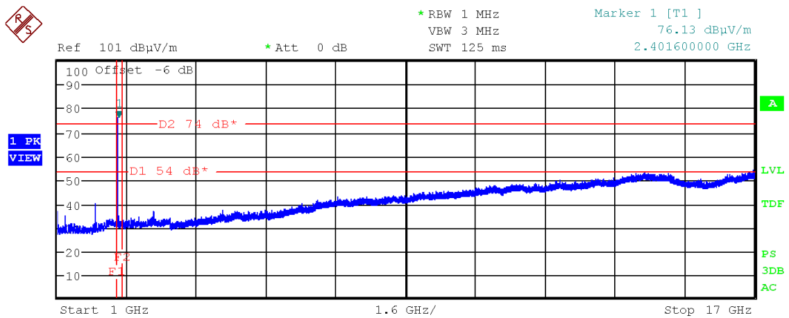
Figure 82: Chart of radiated emissions pre-measurement from 1 GHz to 17 GHz on lowest channel, 1 Mbps, EUT position Y, antenna polarization horizontal
