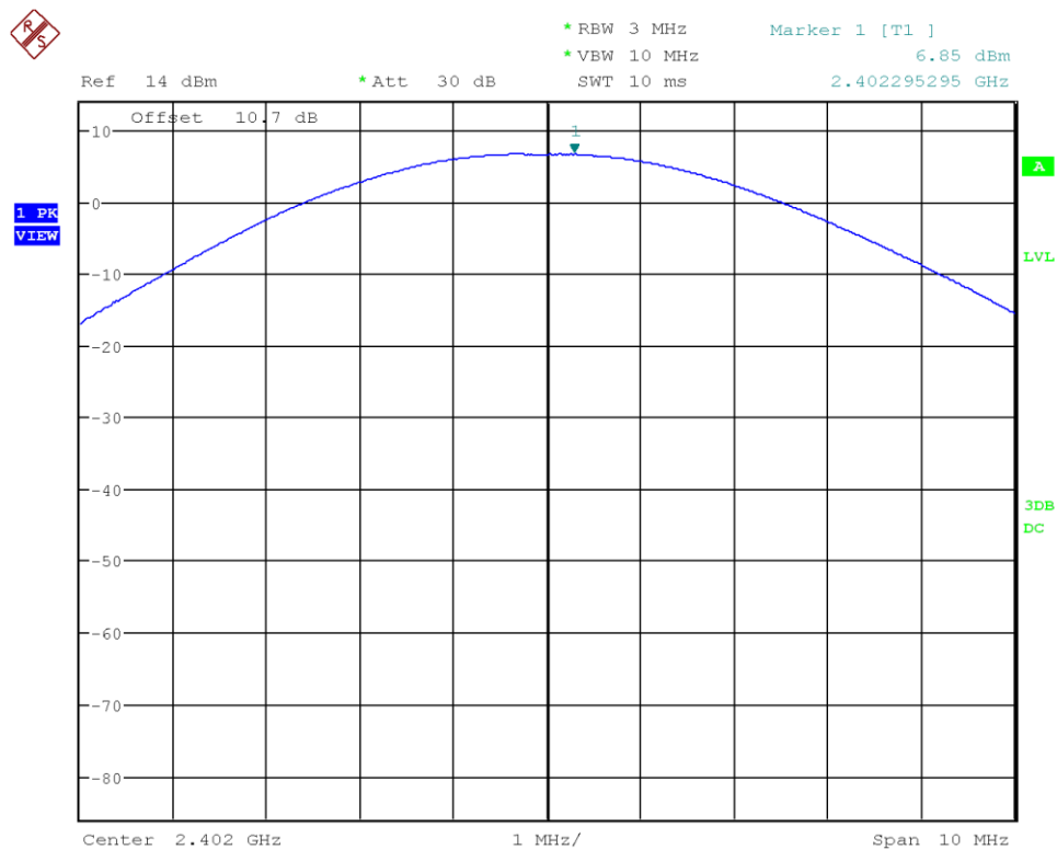
Figure 35: Chart of conducted output power on lowest channel, 500 kbps
