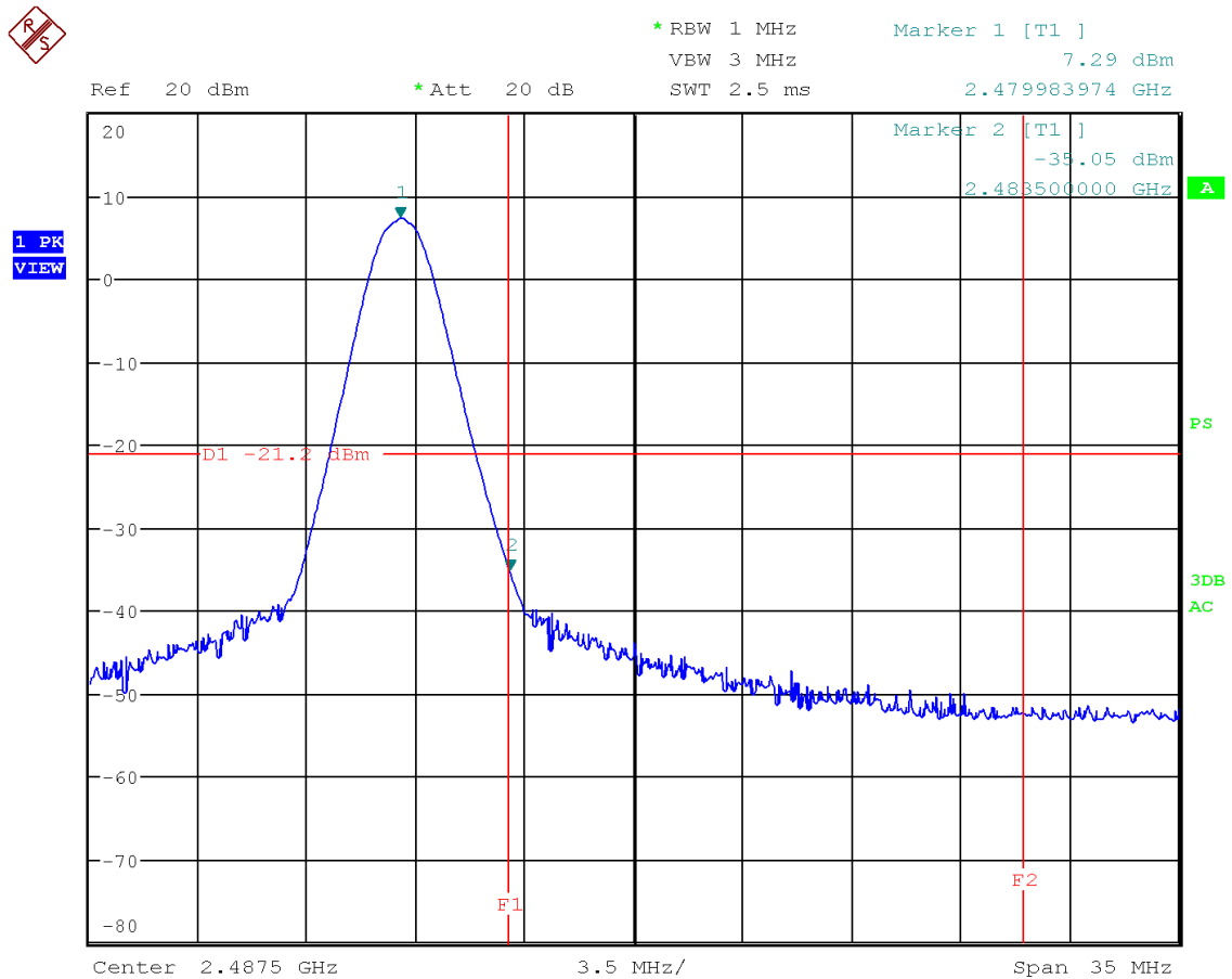
Figure 60: Chart of band-edge measurement on highest channel (PK), 500 kbps
