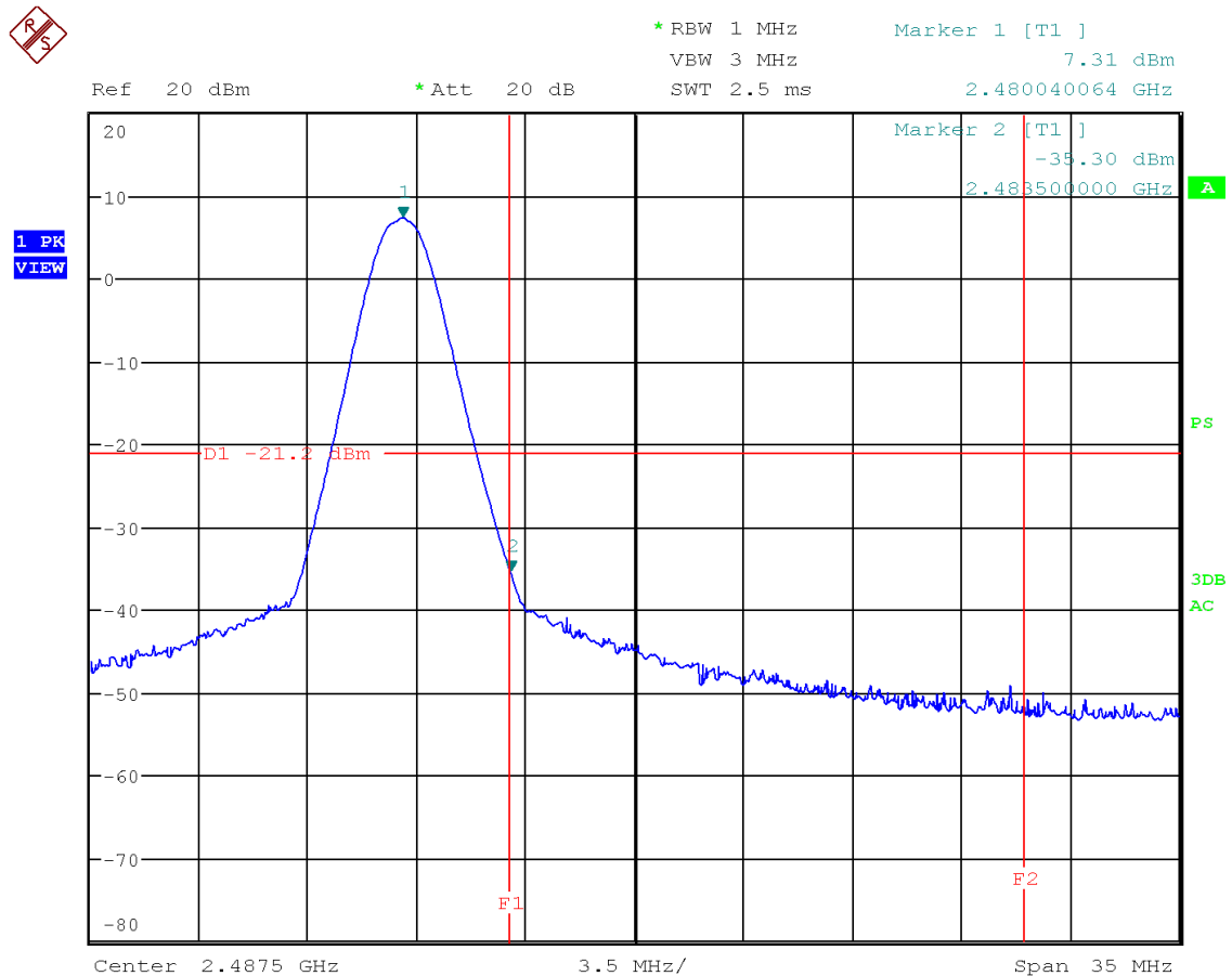
Figure 63: Chart of band-edge measurement on highest channel (PK), 1 Mbps
