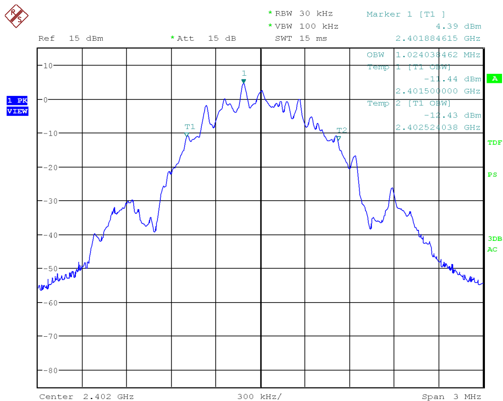
Figure 20: Chart of occupied bandwidth test on lowest channel, 125 kbps
