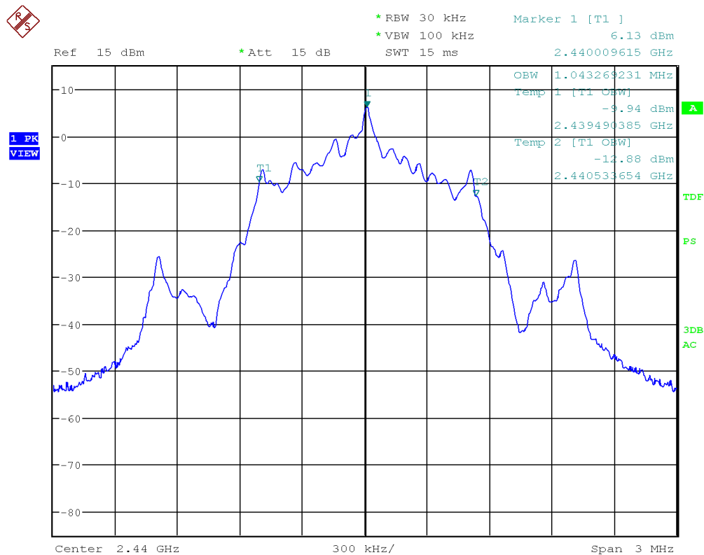
Figure 27: Chart of occupied bandwidth test on middle channel, 1 Mbps
