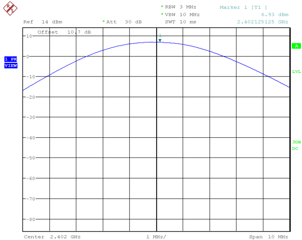
Figure 32: Chart of conducted output power on lowest channel, 125 kbps
