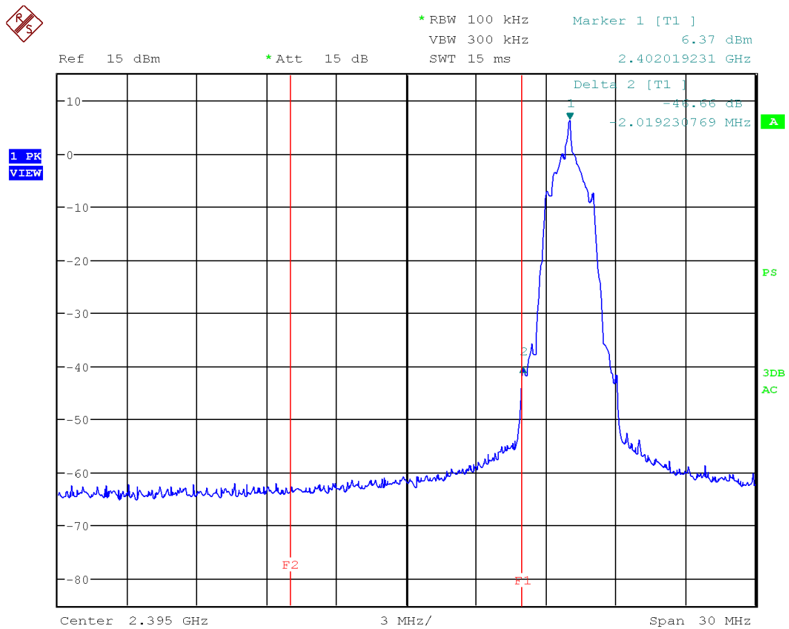
Figure 65: Chart of band-edge measurement on lowest channel, 2 Mbps
