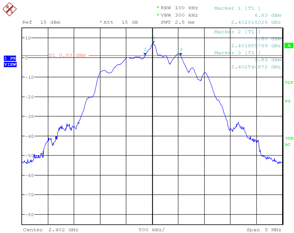
Figure 17: Chart of 6 dB bandwidth test on lowest channel, 2 Mbps
