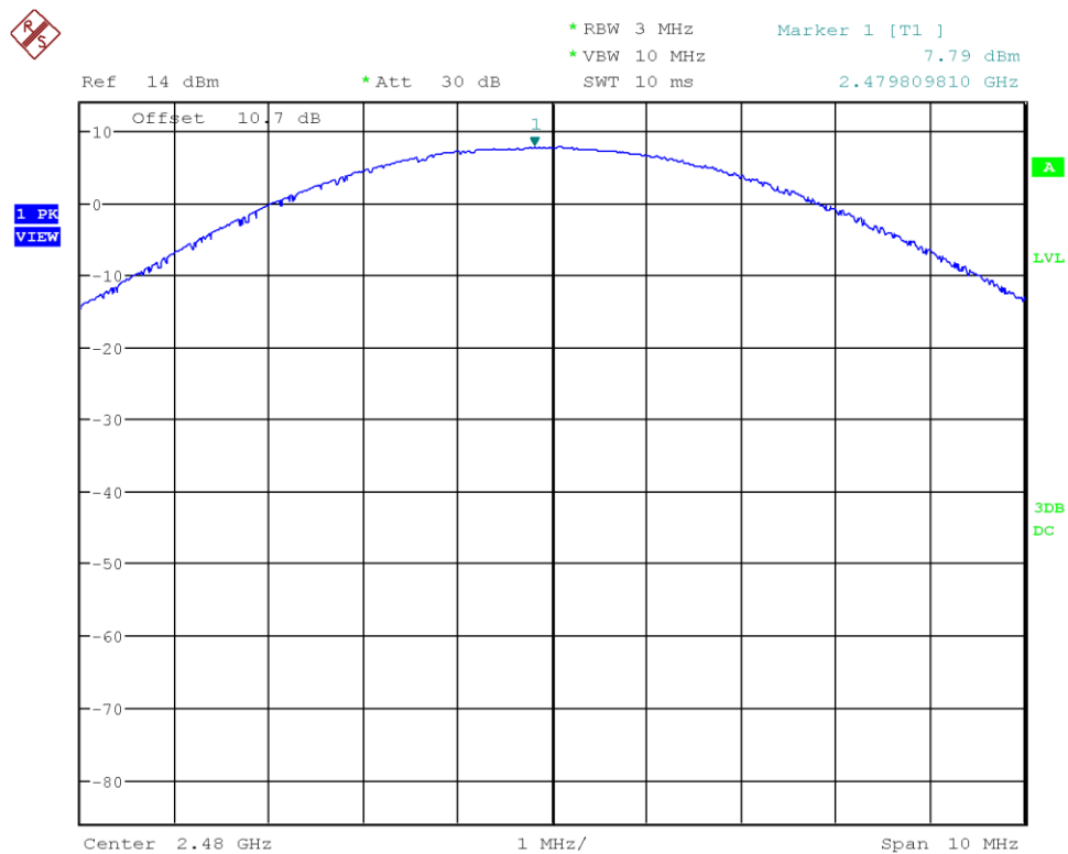
Figure 43: Chart of conducted output power on highest channel, 2 Mbps
