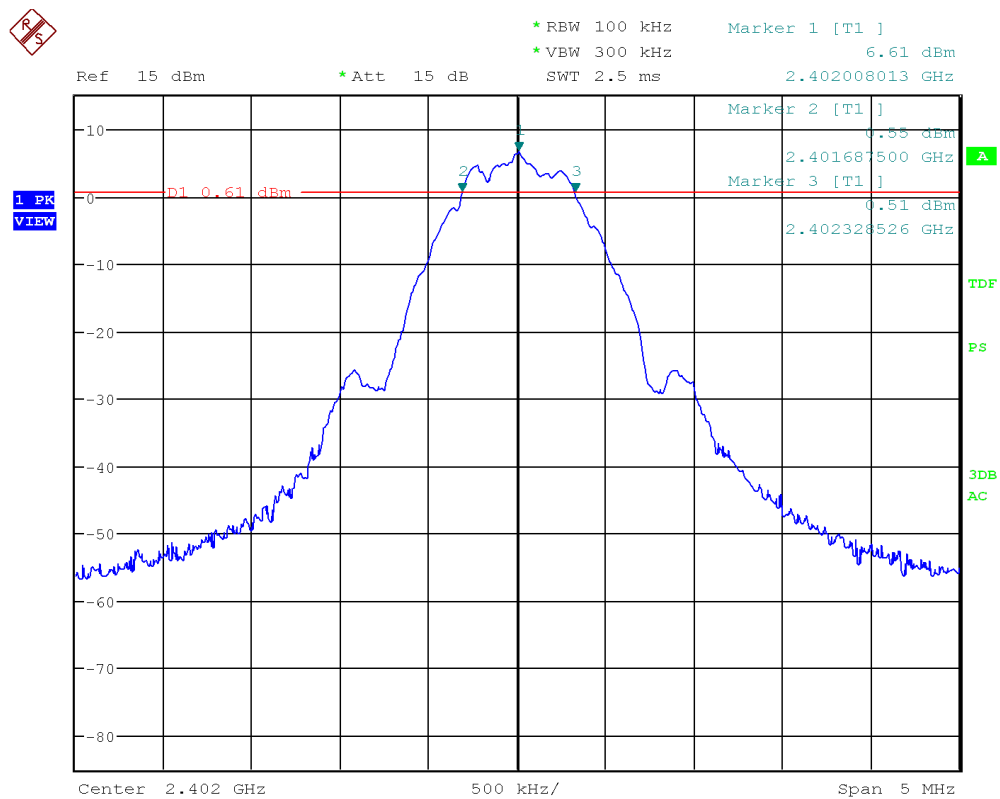
Figure 8: Chart of 6 dB bandwidth test on lowest channel, 125 kbps
