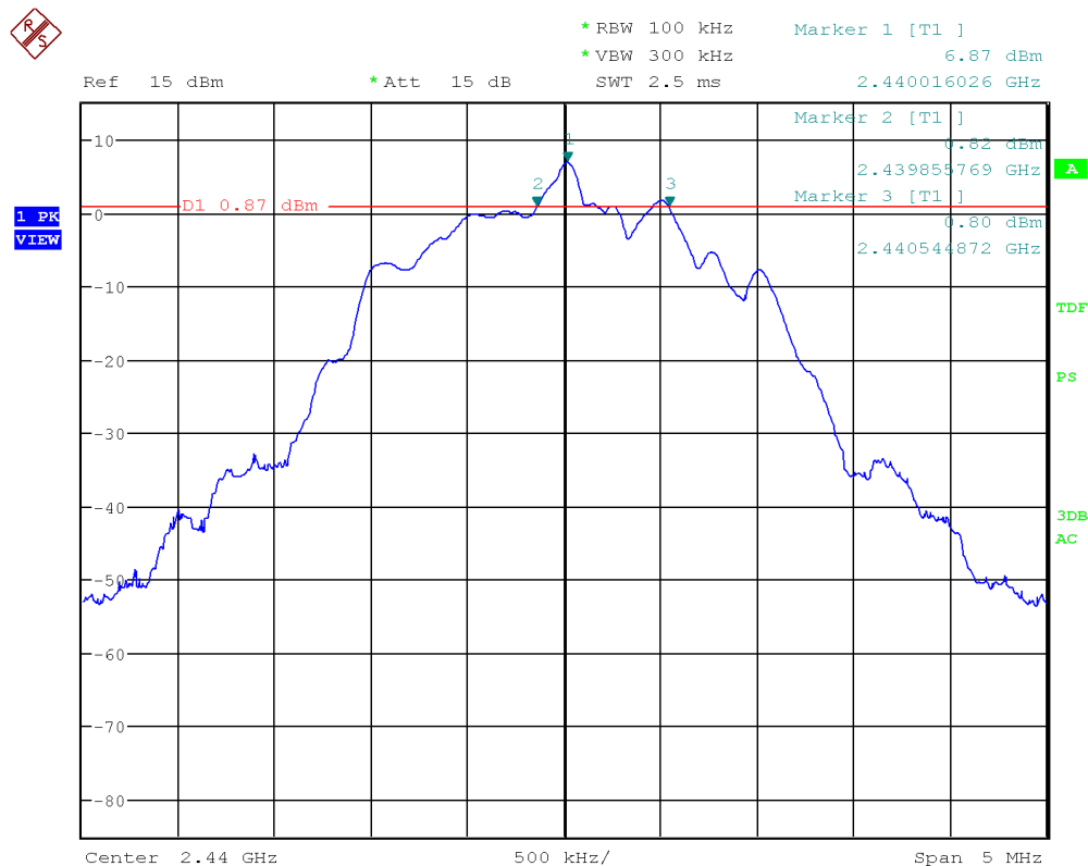
Figure 18: Chart of 6 dB bandwidth test on middle channel, 2 Mbps
