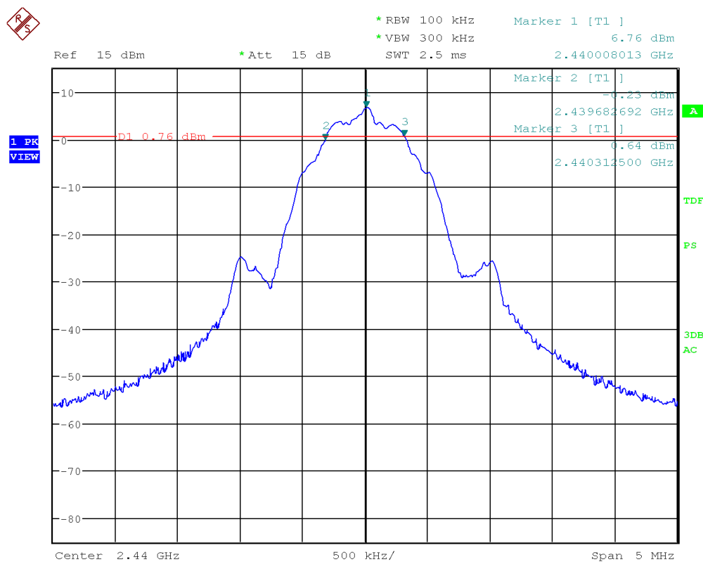
Figure 15: Chart of 6 dB bandwidth test on middle channel, 1 Mbps
