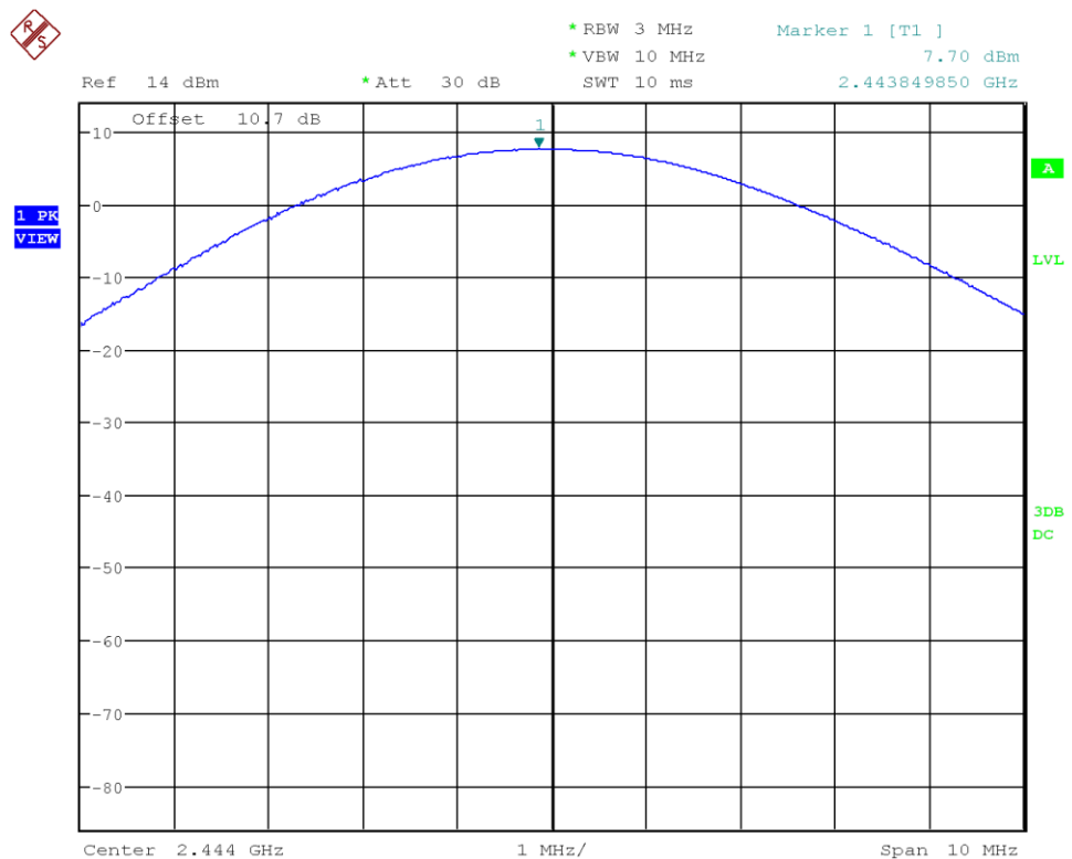
Figure 39: Chart of conducted output power on middle channel, 1 Mbps
