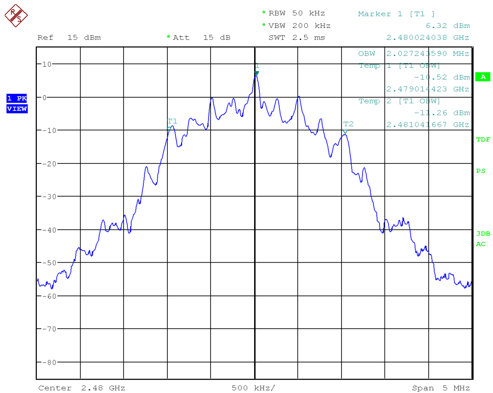
Figure 31: Chart of occupied bandwidth test on highest channel, 2 Mbps
