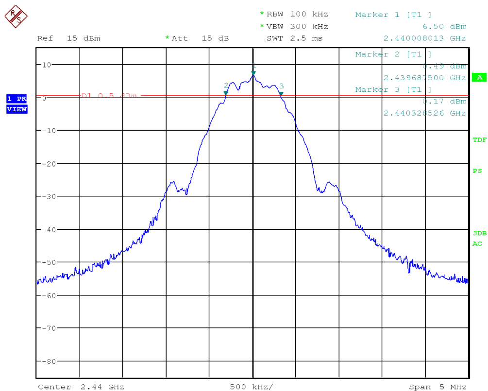
Figure 9: Chart of 6 dB bandwidth test on middle channel, 125 kbps
