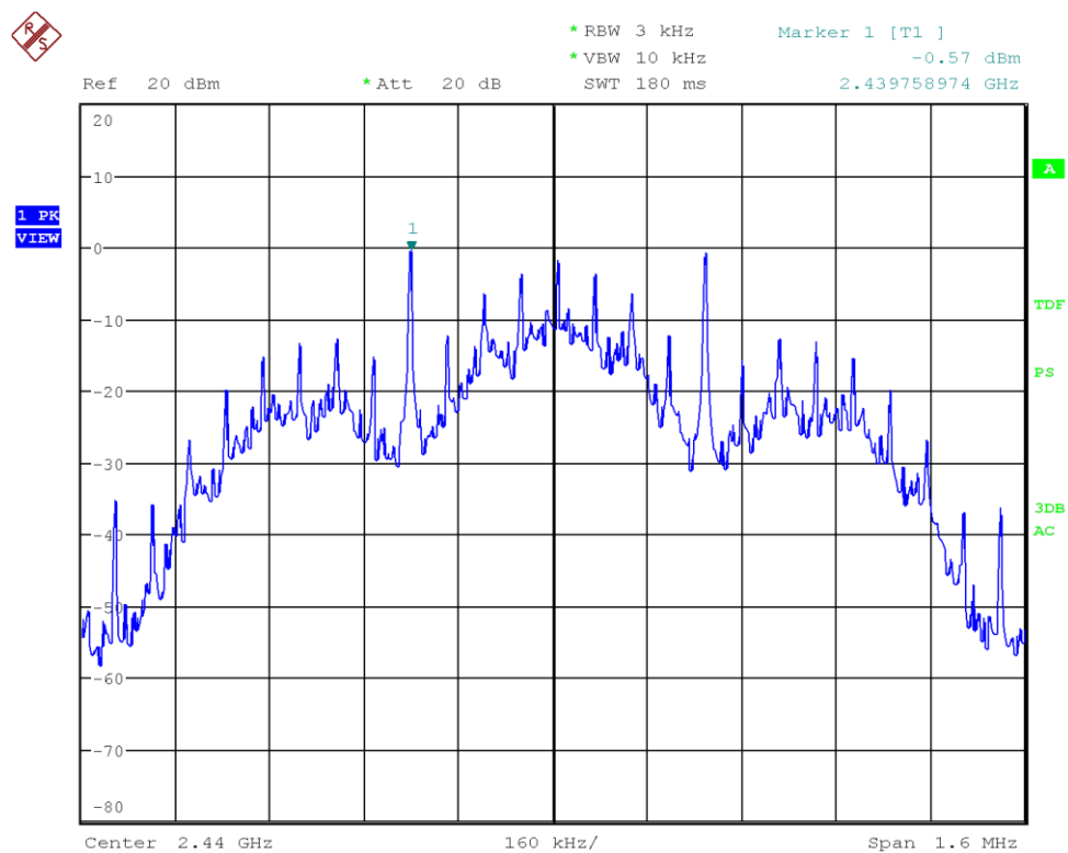
Figure 48: Chart of power spectral density on middle channel, 500 kbps
