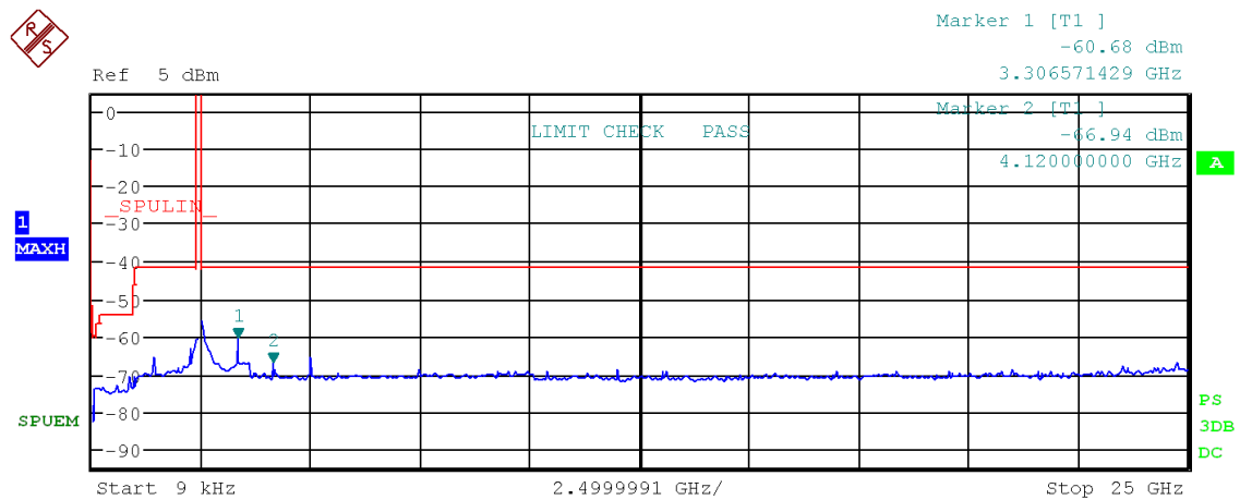
Figure 76: Chart of emissions test from 9 kHz to 25 GHz on highest channel, 1 Mbps, PK-detector
