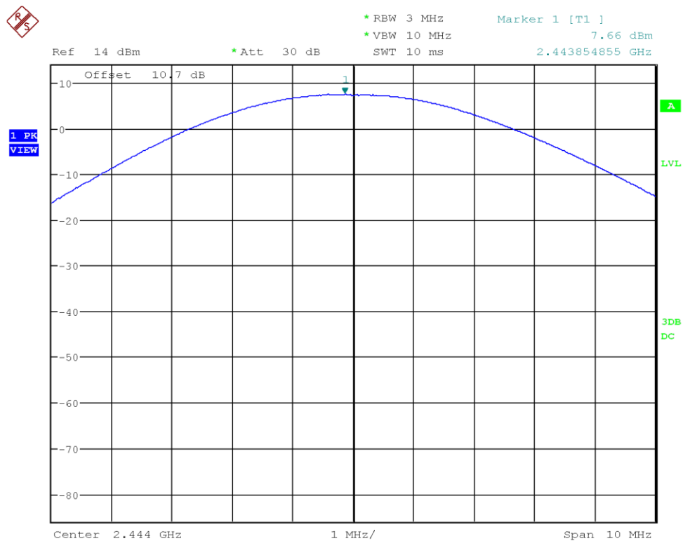
Figure 36: Chart of conducted output power on middle channel, 500 kbps
