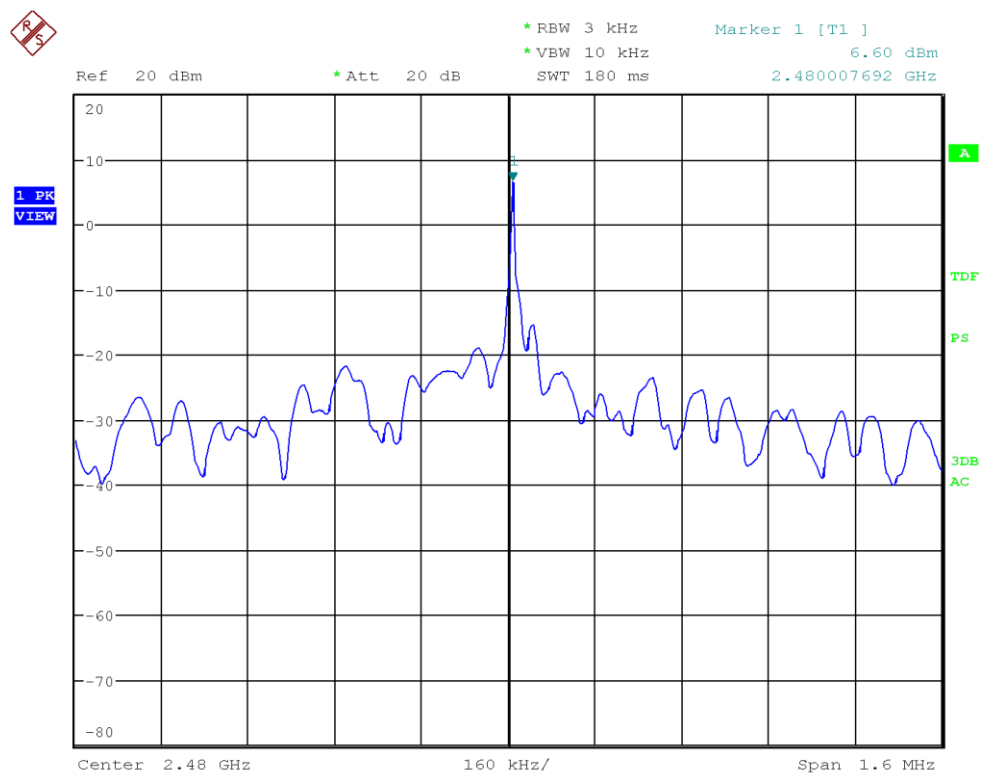
Figure 55: Chart of power spectral density on highest channel, 2 Mbps
