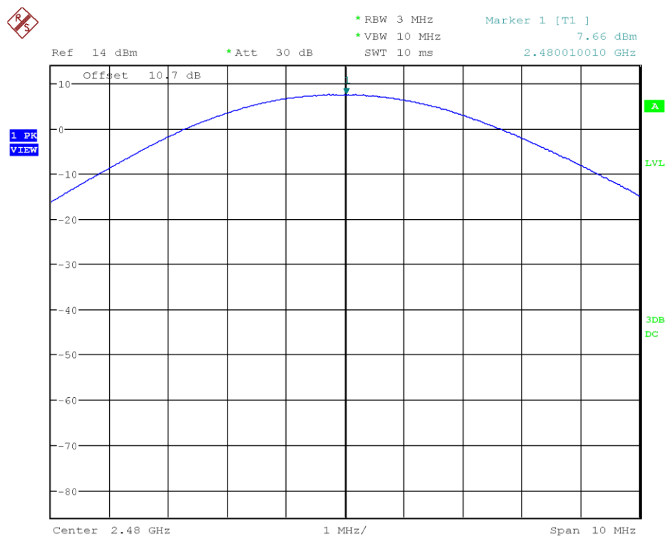
Figure 34: Chart of conducted output power on highest channel, 125 kbps
