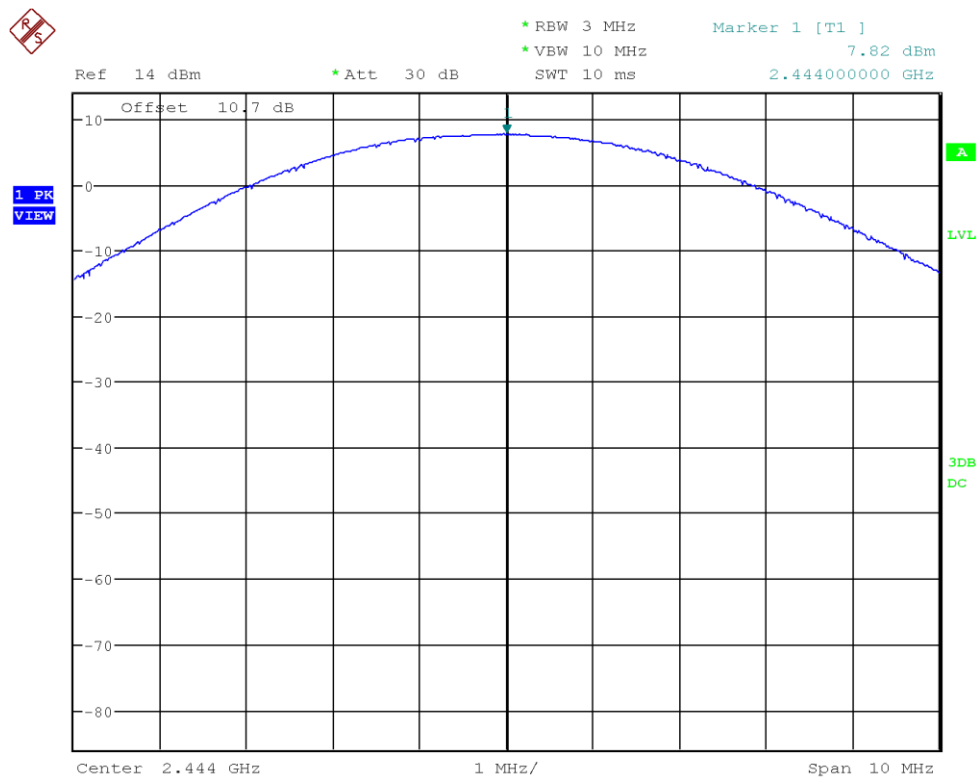
Figure 42: Chart of conducted output power on middle channel, 2 Mbps
