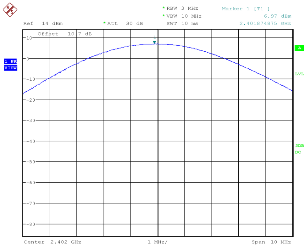
Figure 38: Chart of conducted output power on lowest channel, 1 Mbps
