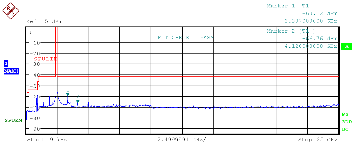
Figure 73: Chart of emissions test from 9 kHz to 25 GHz on highest channel, 500 kbps, PK-detector
