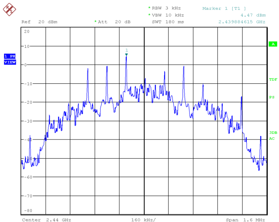
Figure 45: Chart of power spectral density on middle channel, 125 kbps
