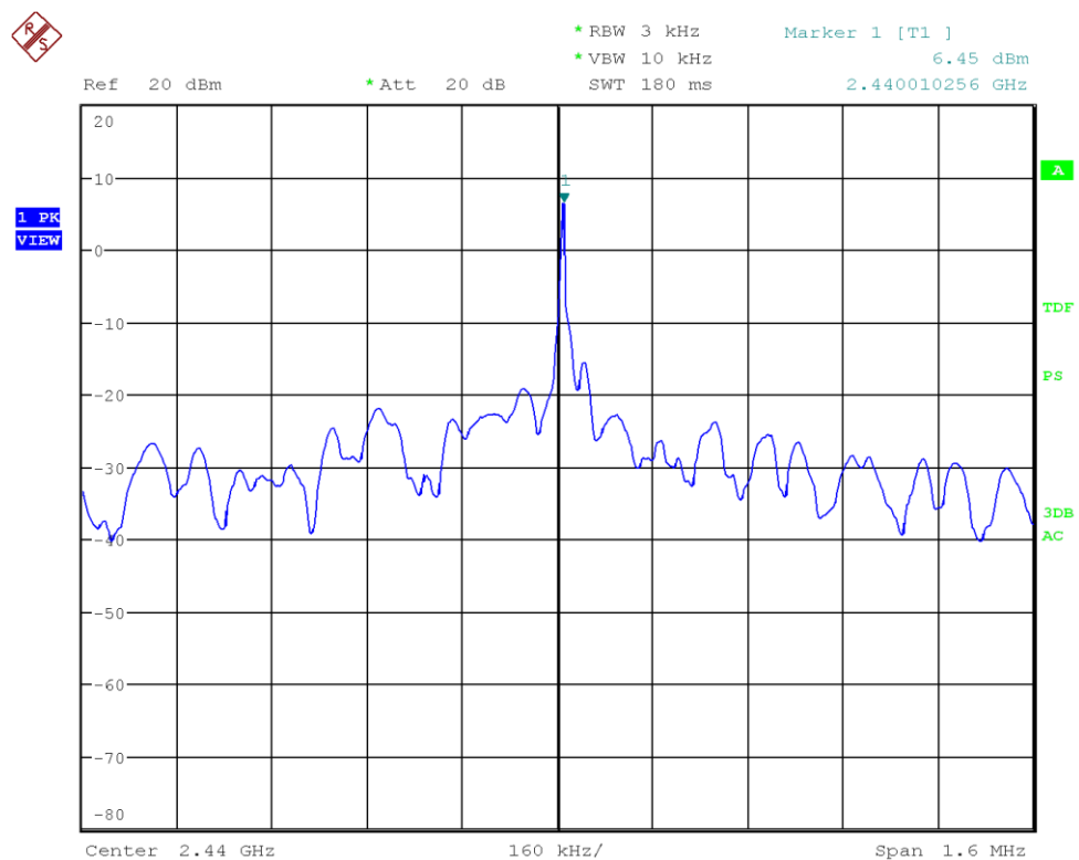
Figure 54: Chart of power spectral density on middle channel, 2 Mbps
