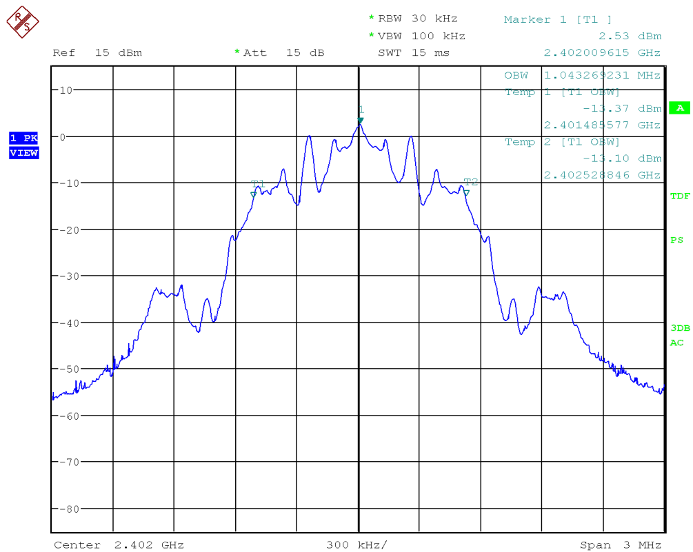
Figure 23: Chart of occupied bandwidth test on lowest channel, 500 kbps
