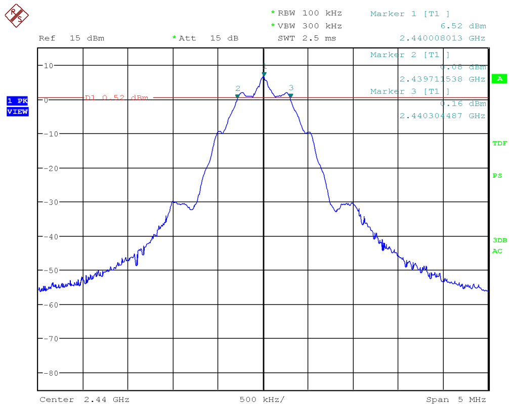
Figure 12: Chart of 6 dB bandwidth test on middle channel, 500 kbps
