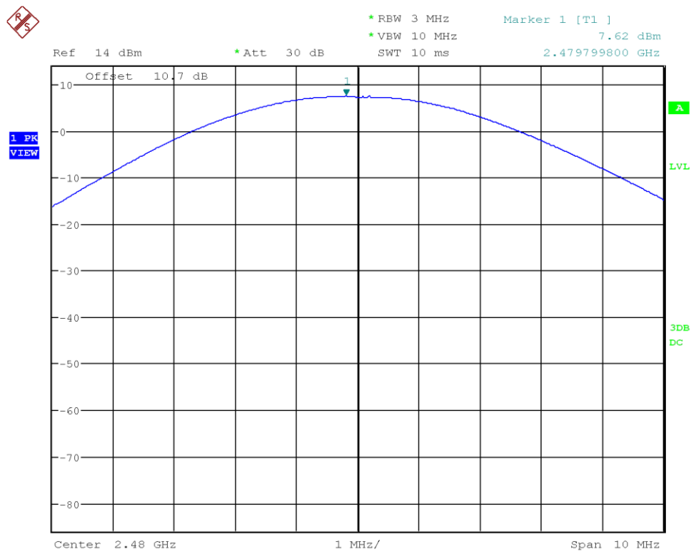
Figure 37: Chart of conducted output power on highest channel, 500 kbps
