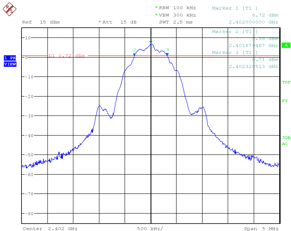
Figure 14: Chart of 6 dB bandwidth test on lowest channel, 1 Mbps
