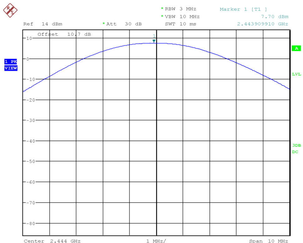
Figure 33: Chart of conducted output power on middle channel, 125 kbps
