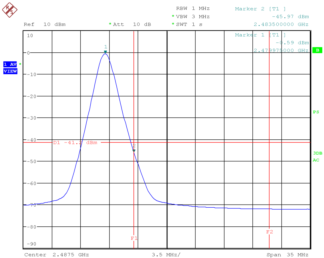
Figure 64: Chart of band-edge measurement on highest channel (AV), 1 Mbps
