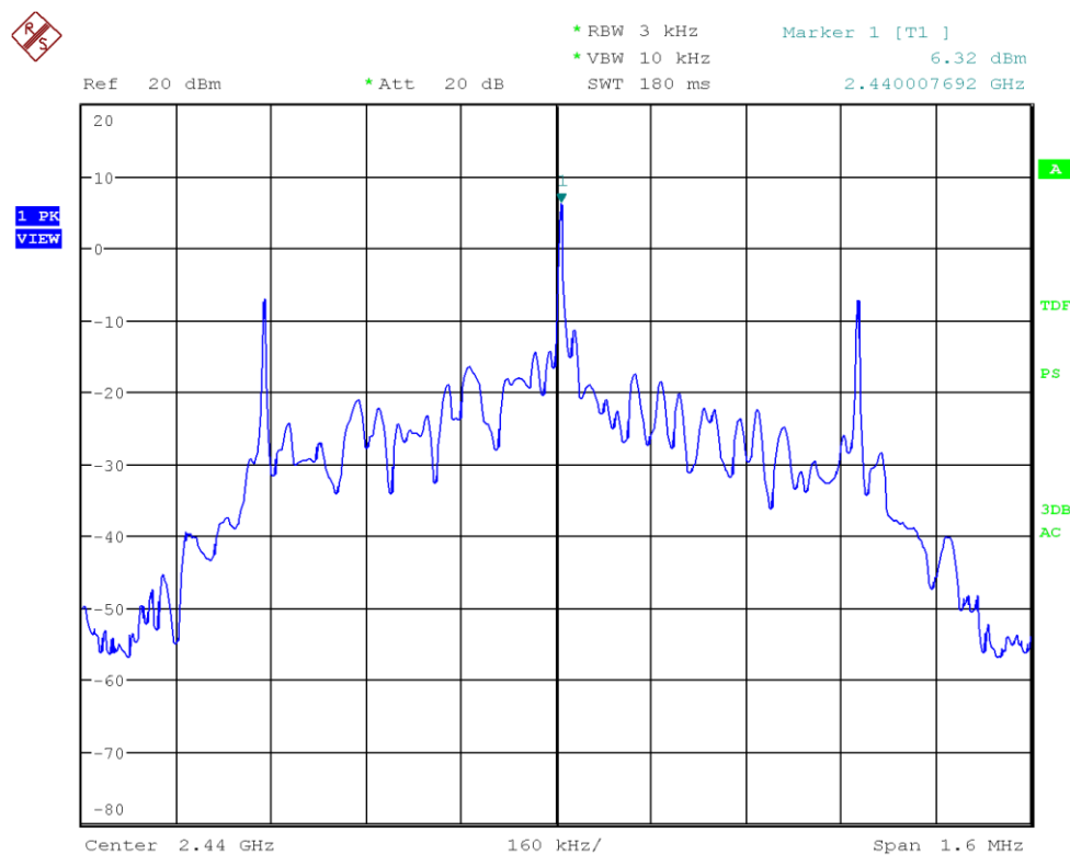
Figure 51: Chart of power spectral density on middle channel, 1 Mbps
