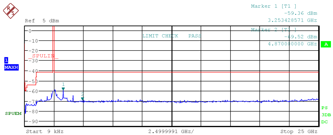
Figure 78: Chart of emissions test from 9 kHz to 25 GHz on middle channel, 2 Mbps, PK-detector
