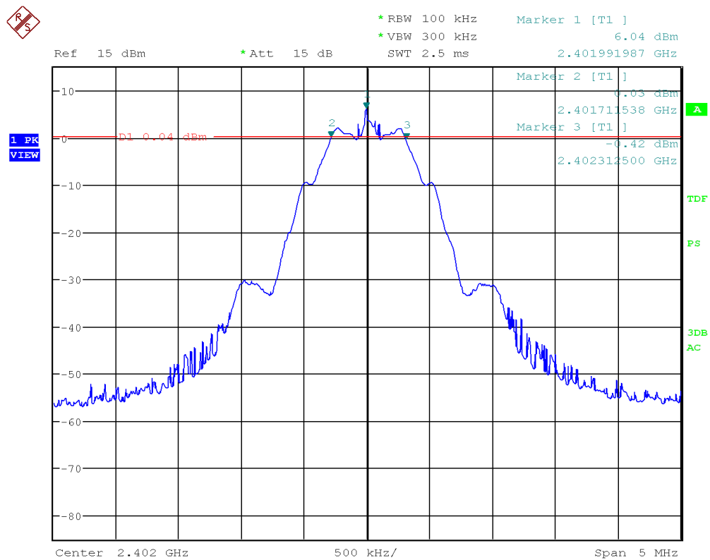
Figure 11: Chart of 6 dB bandwidth test on lowest channel, 500 kbps
