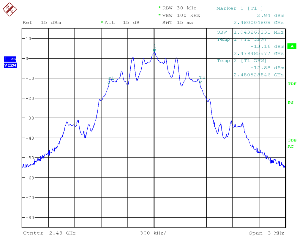
Figure 25: Chart of occupied bandwidth test on highest channel, 500 kbps
