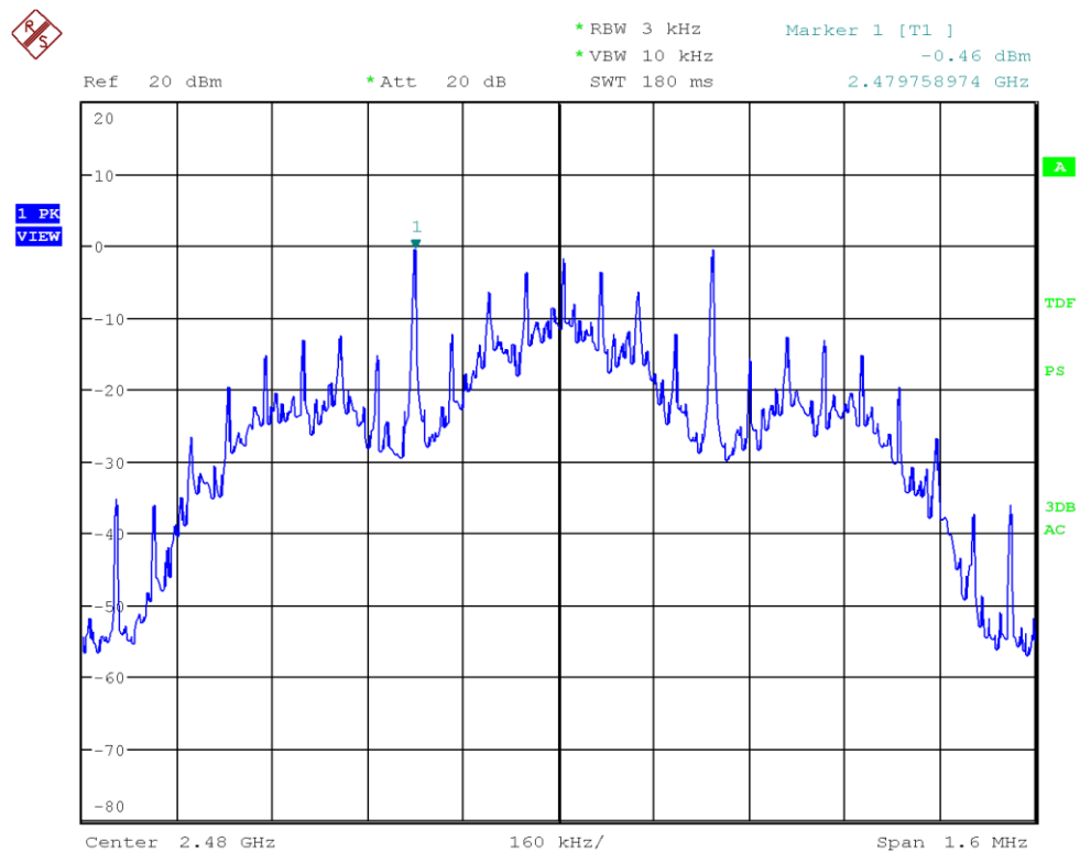
Figure 49: Chart of power spectral density on highest channel, 500 kbps
