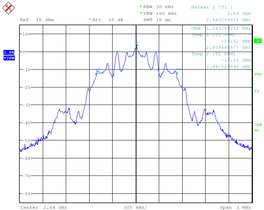
Figure 24: Chart of occupied bandwidth test on middle channel, 500 kbps
