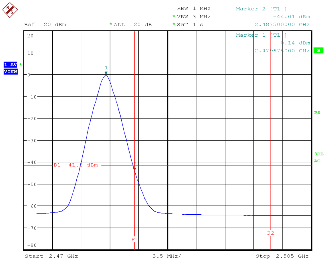
Figure 67: Chart of band-edge measurement on highest channel (AV), 2 Mbps
