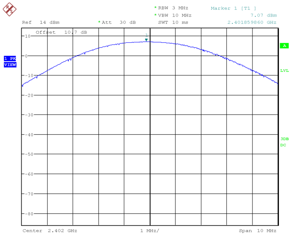
Figure 41: Chart of conducted output power on lowest channel, 2 Mbps
