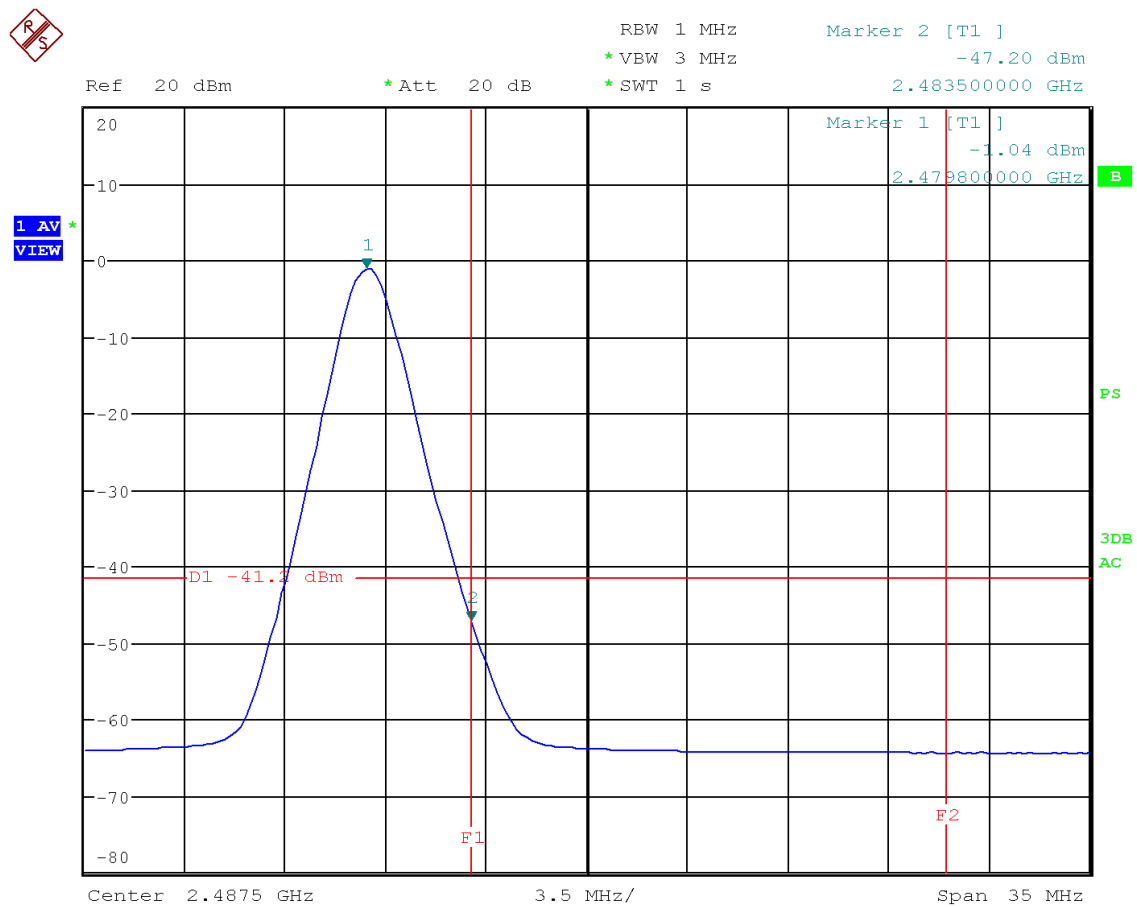
Figure 58: Chart of band-edge measurement on highest channel (AV), 125 kbps
