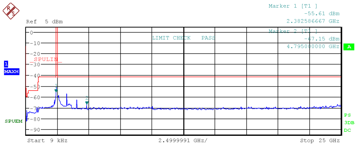
Figure 74: Chart of emissions test from 9 kHz to 25 GHz on lowest channel, 1 Mbps, PK-detector
