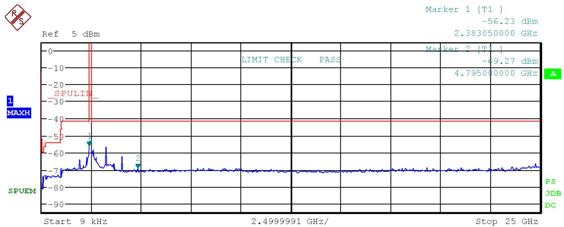
Figure 77: Chart of emissions test from 9 kHz to 25 GHz on lowest channel, 2 Mbps, PK-detector
