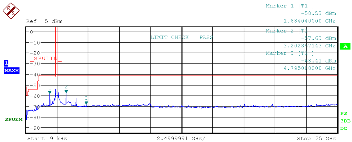
Figure 71: Chart of emissions test from 9 kHz to 25 GHz on lowest channel, 500 kbps, PK-detector
