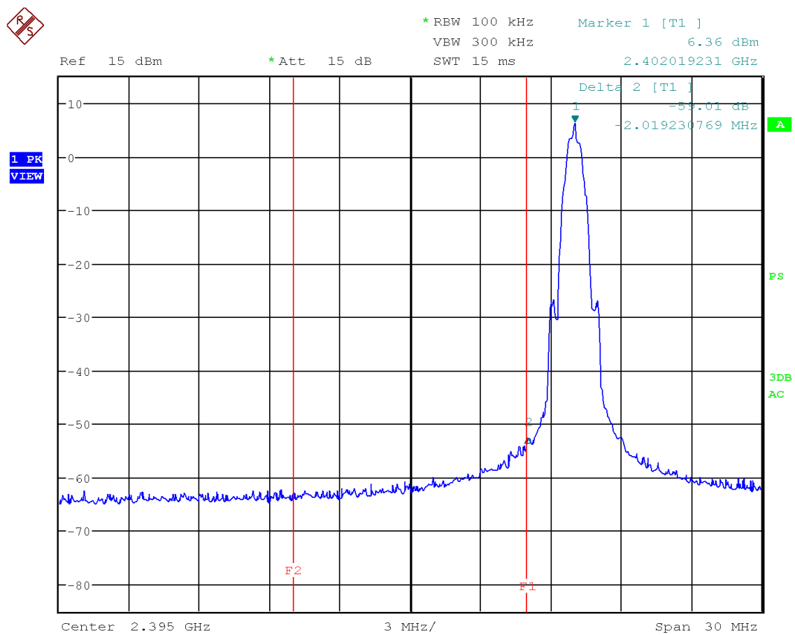
Figure 62: Chart of band-edge measurement on lowest channel, 1 Mbps
