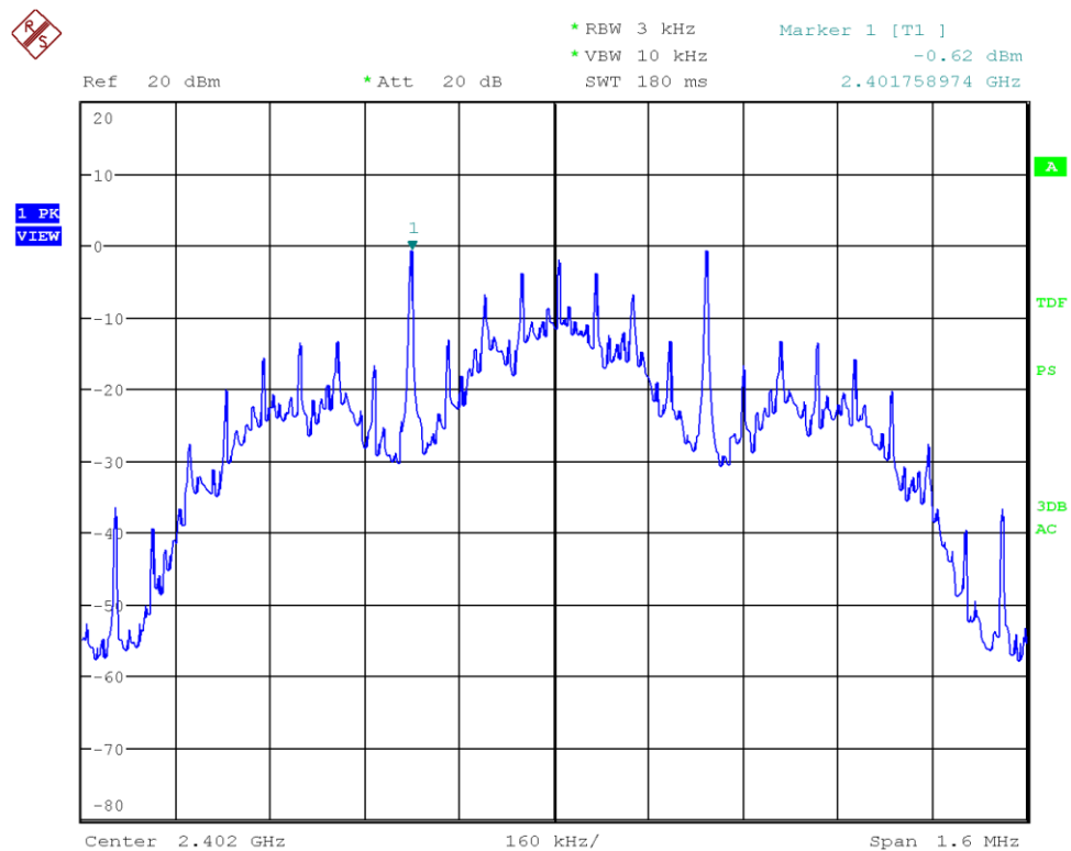
Figure 47: Chart of power spectral density on lowest channel, 500 kbps
