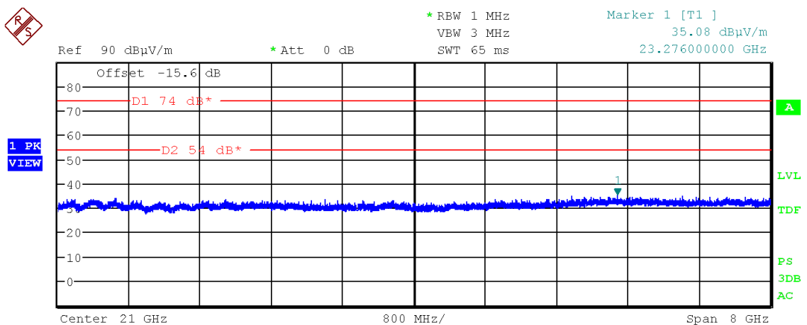
Figure 87: Chart of exploratory emission test from 17 GHz to 25 GHz on highest channel, 1 Mbps, at 0.5 m
