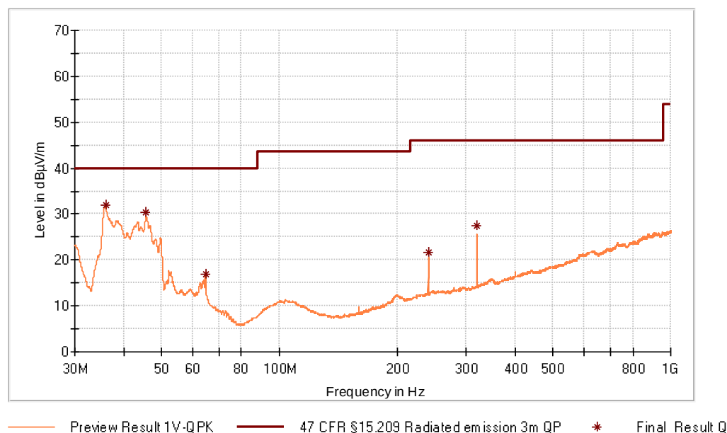
Figure 81: Chart of emissions test from 30 MHz to 1 GHz on lowest channel, 1 Mbps, EUT position X, antenna polarization vertical
