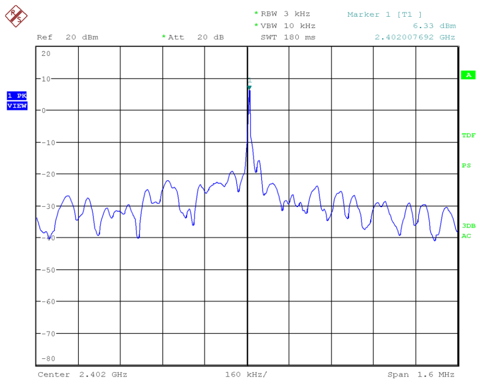
Figure 53: Chart of power spectral density on lowest channel, 2 Mbps
