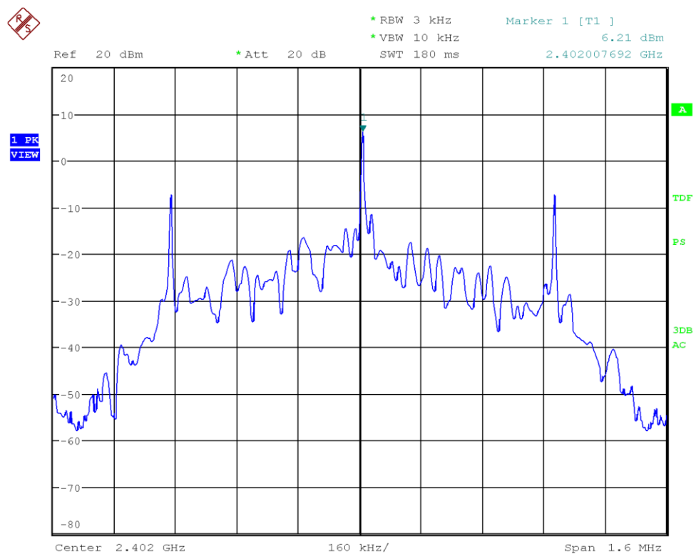
Figure 50: Chart of power spectral density on lowest channel, 1 Mbps
