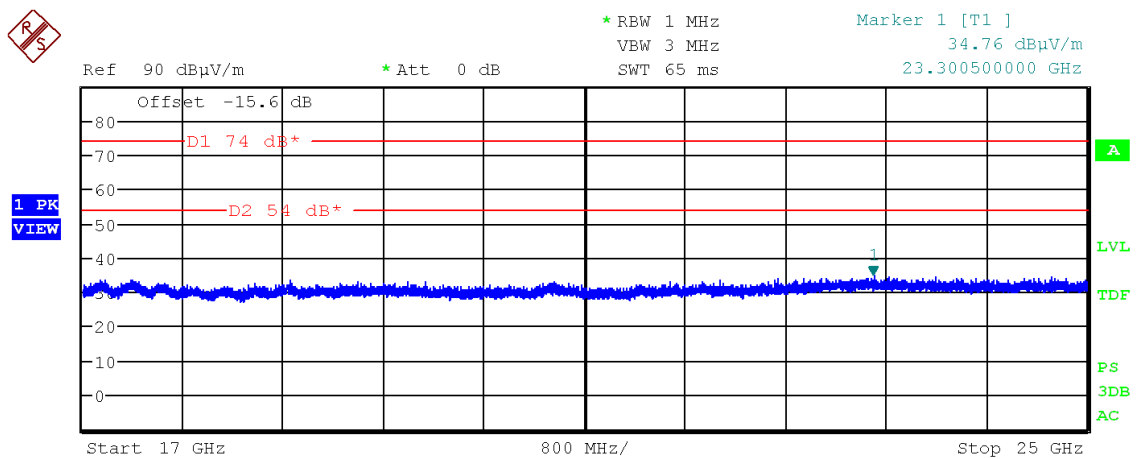
Figure 83: Chart of exploratory emissions measurement from 17 GHz to 25 GHz on lowest channel, 1 Mbps
