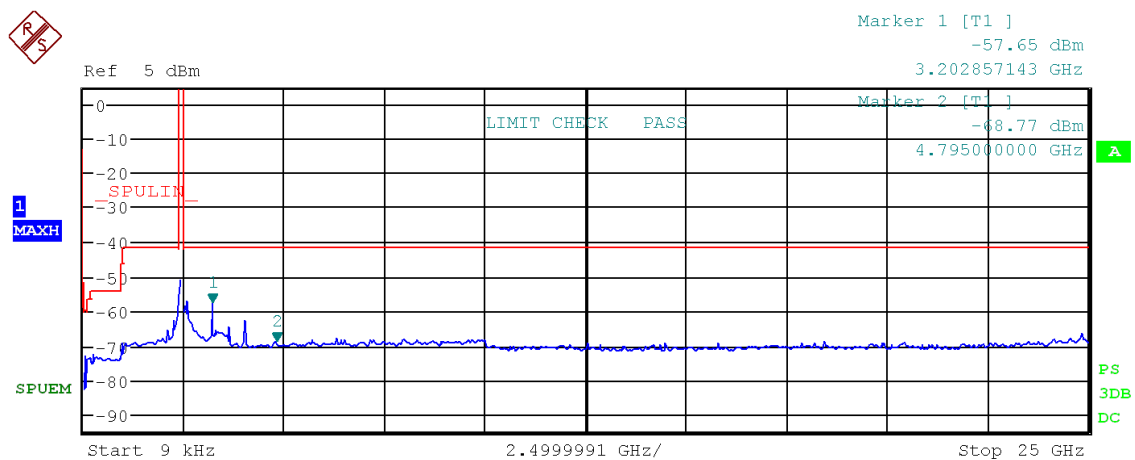
Figure 68: Chart of emissions test from 9 kHz to 25 GHz on lowest channel, 125 kbps, PK-detector
