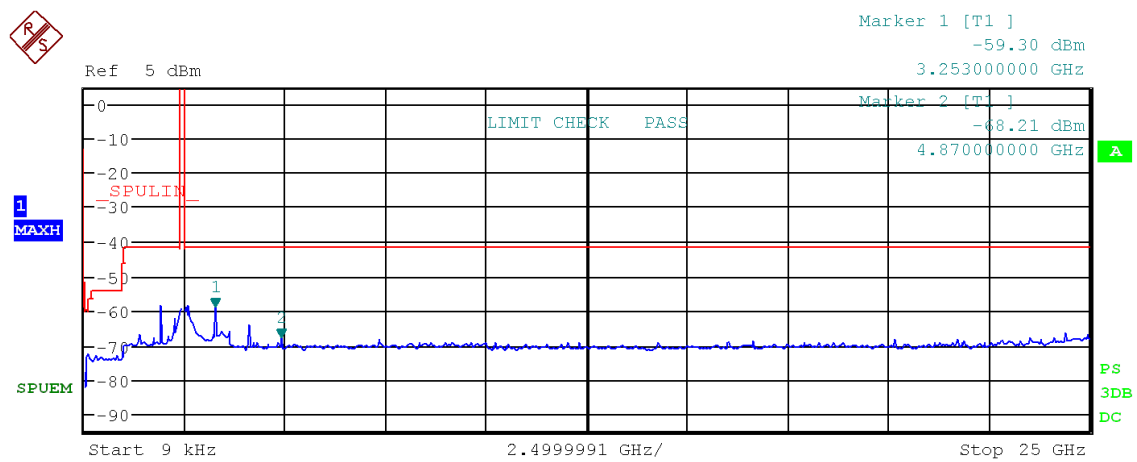
Figure 75: Chart of emissions test from 9 kHz to 25 GHz on middle channel, 1 Mbps, PK-detector
