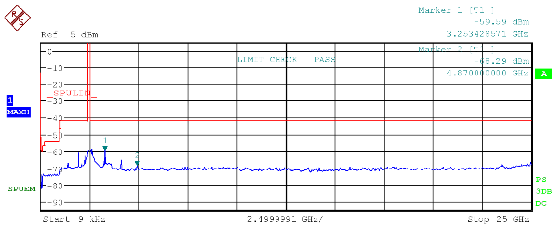
Figure 69: Chart of emissions test from 9 kHz to 25 GHz on middle channel, 125 kbps, PK-detector
