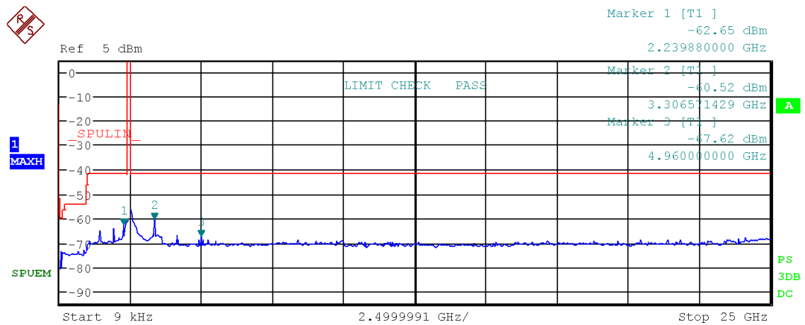
Figure 70: Chart of emissions test from 9 kHz to 25 GHz on highest channel, 125 kbps, PK-detector
