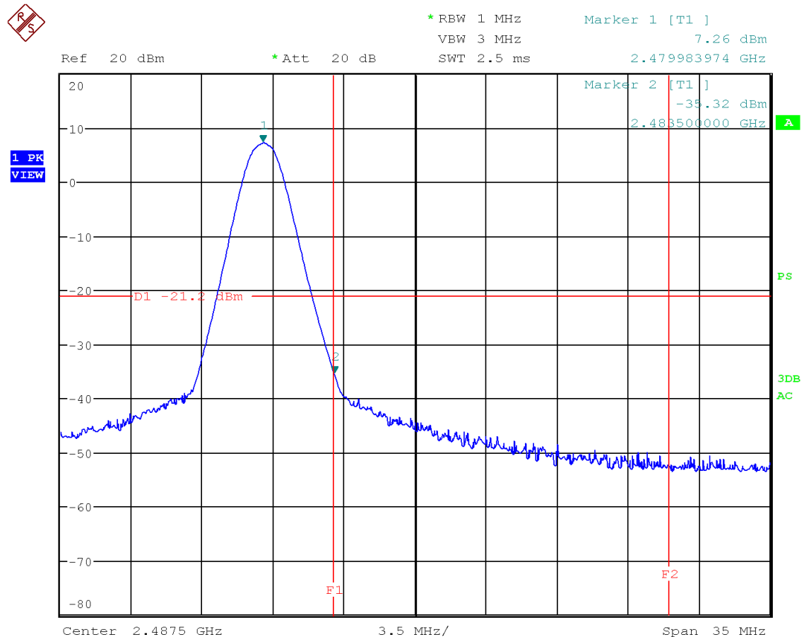
Figure 57: Chart of band-edge measurement on highest channel (PK), 125 kbps
