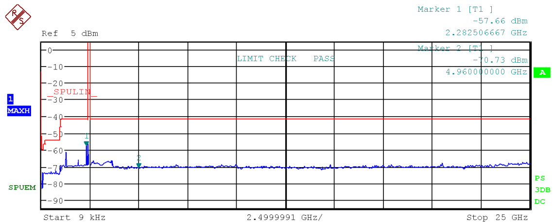
Figure 79: Chart of emissions test from 9 kHz to 25 GHz on highest channel, 2 Mbps, PK-detector
