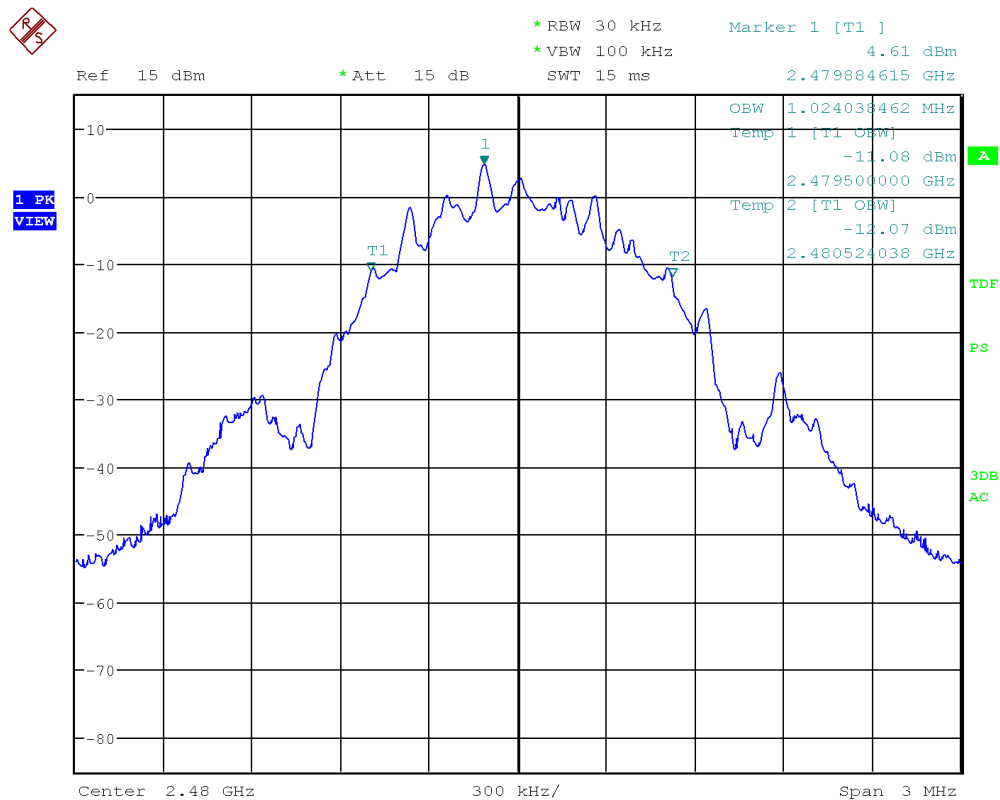
Figure 22: Chart of occupied bandwidth test on highest channel, 125 kbps
