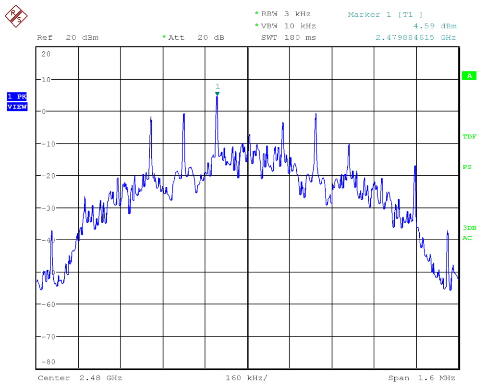
Figure 46: Chart of power spectral density on highest channel, 125 kbps
