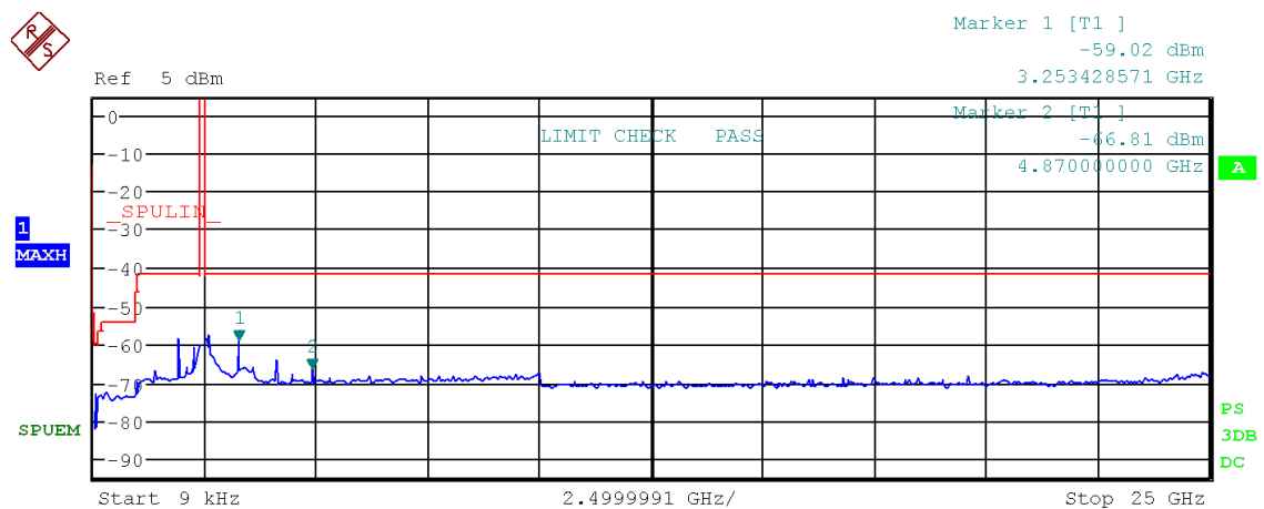
Figure 72: Chart of emissions test from 9 kHz to 25 GHz on middle channel, 500 kbps, PK-detector
