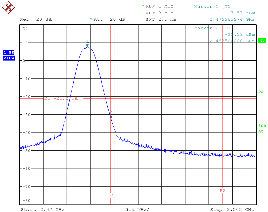
Figure 66: Chart of band-edge measurement on highest channel (PK), 2 Mbps
