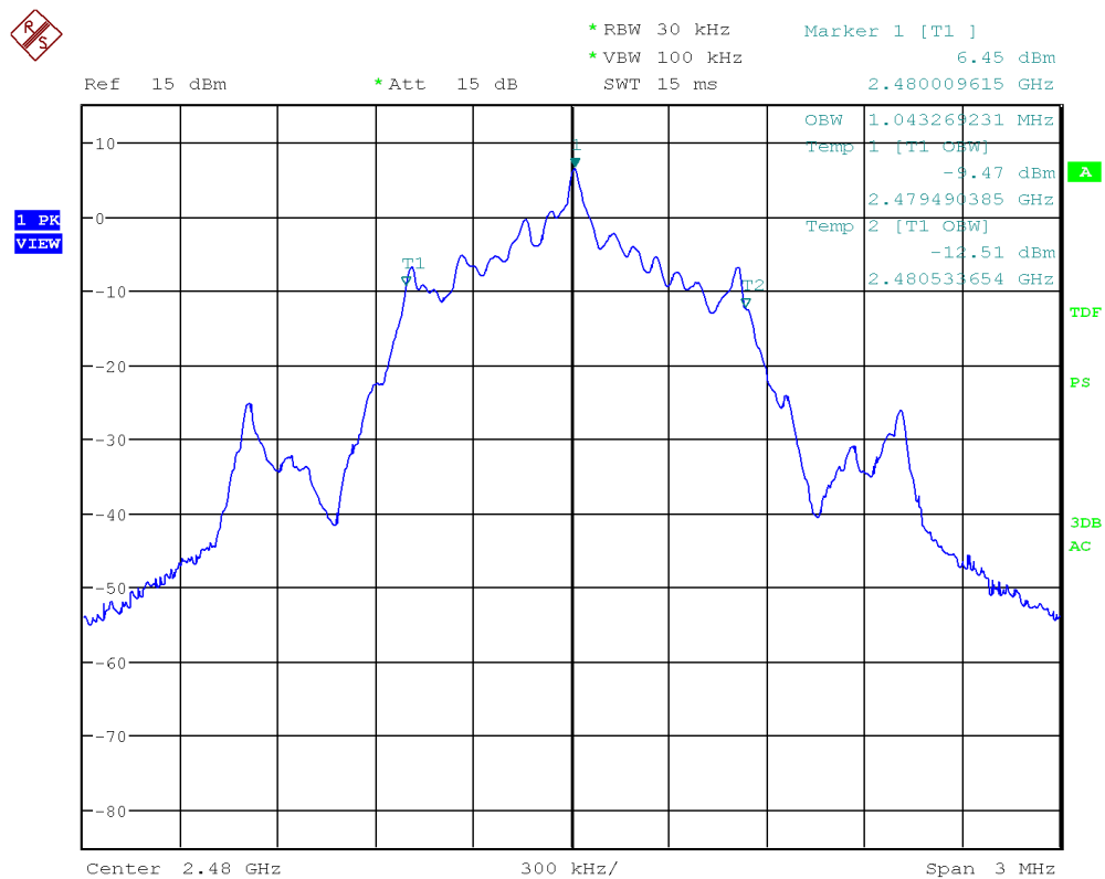
Figure 28: Chart of occupied bandwidth test on highest channel, 1 Mbps
