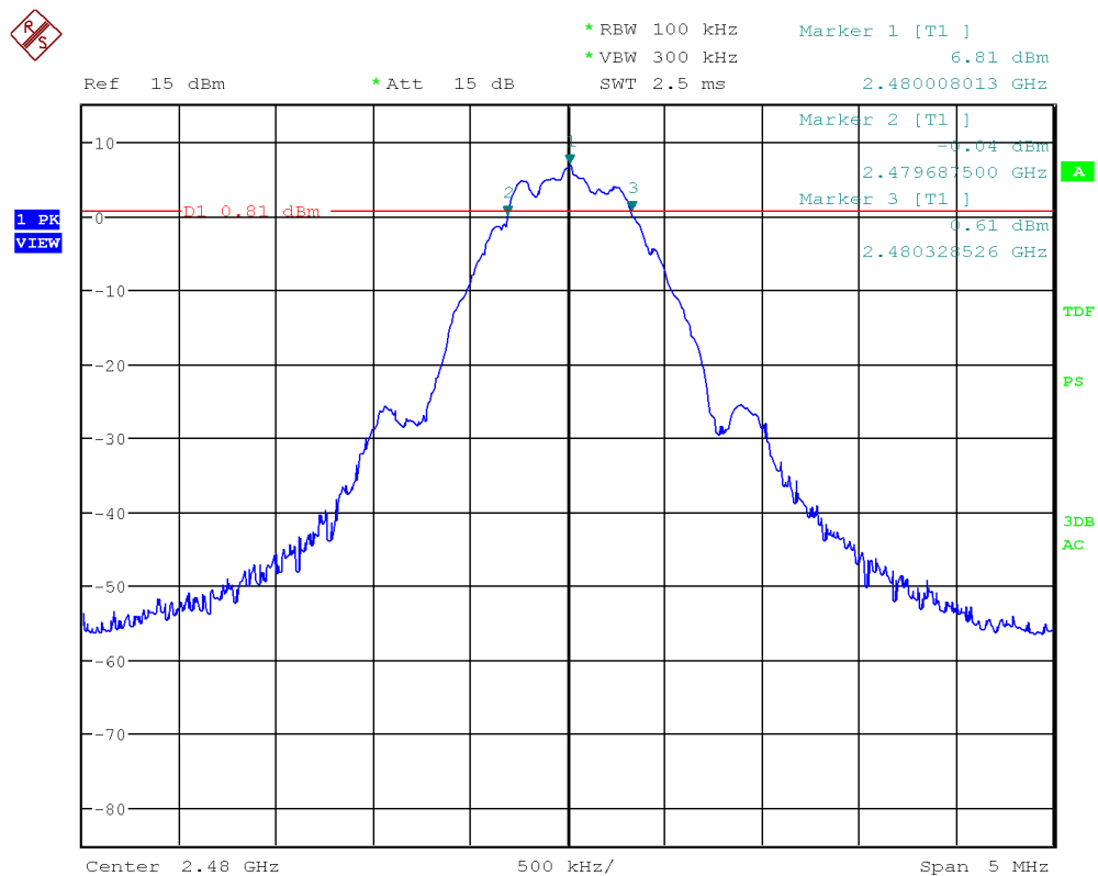
Figure 10: Chart of 6 dB bandwidth test on highest channel, 125 kbps
