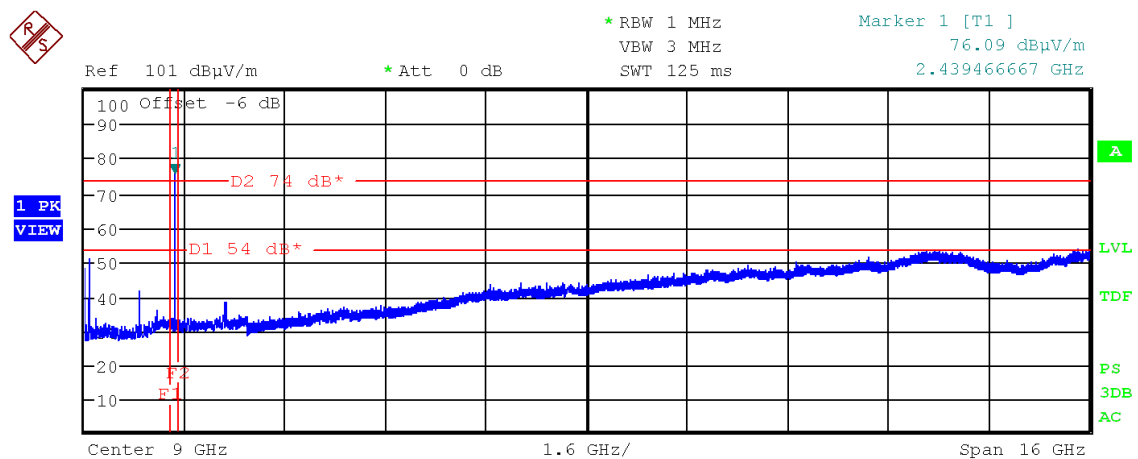
Figure 84: Chart of radiated emissions pre-measurement from 1 GHz to 17 GHz on middle channel, 1 Mbps, EUT position Y, antenna polarization horizontal
