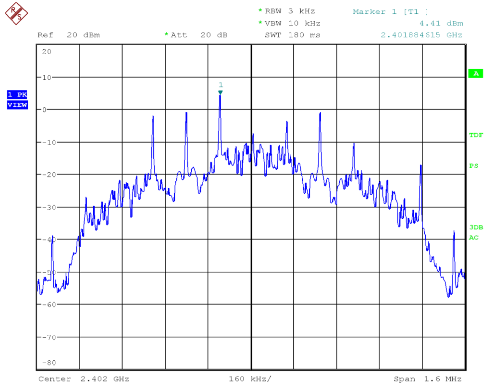
Figure 44: Chart of power spectral density on lowest channel, 125 kbps
