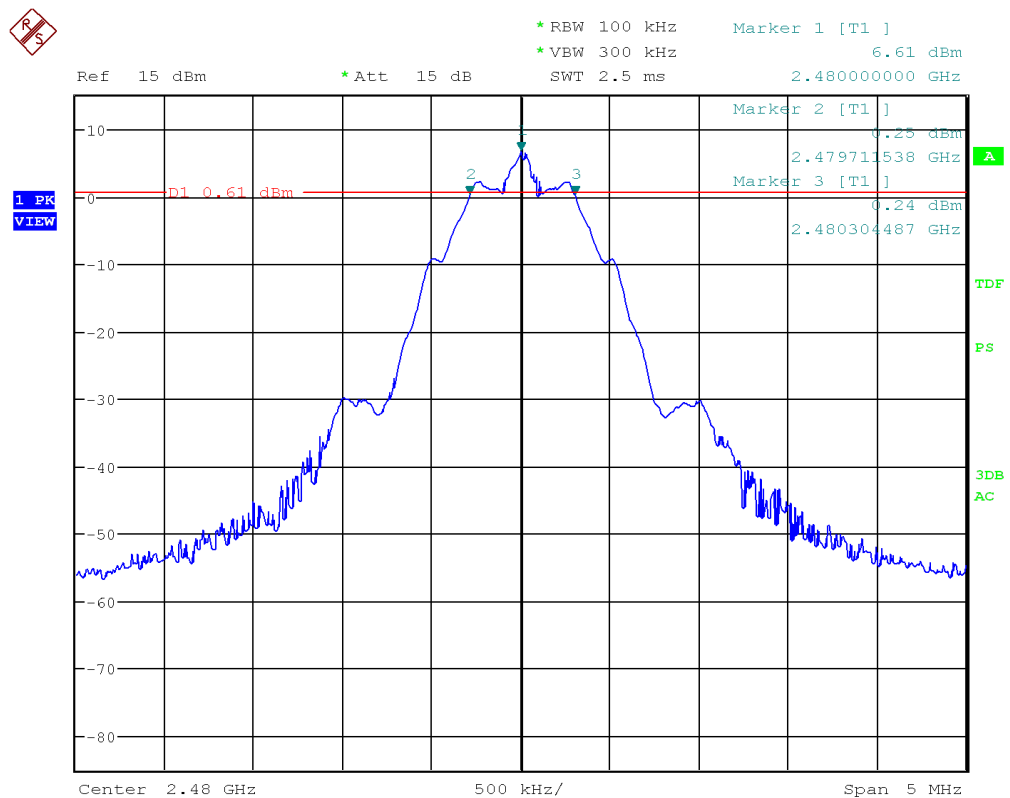
Figure 13: Chart of 6 dB bandwidth test on highest channel, 500 kbps
