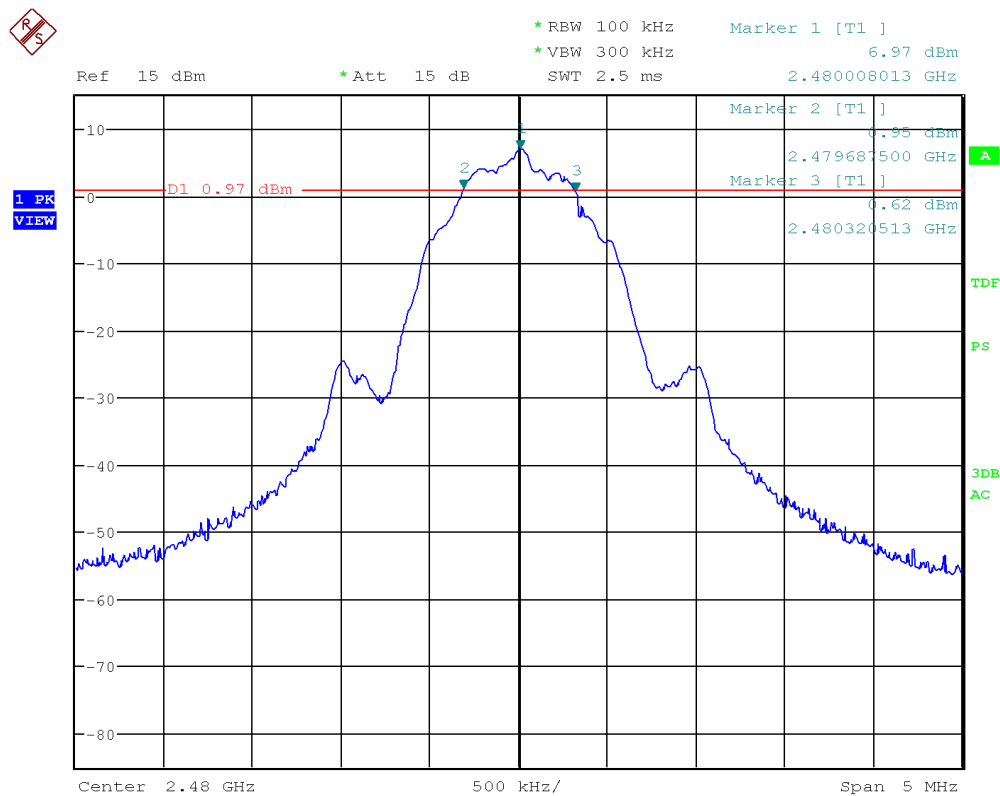
Figure 16: Chart of 6 dB bandwidth test on highest channel, 1 Mbps
