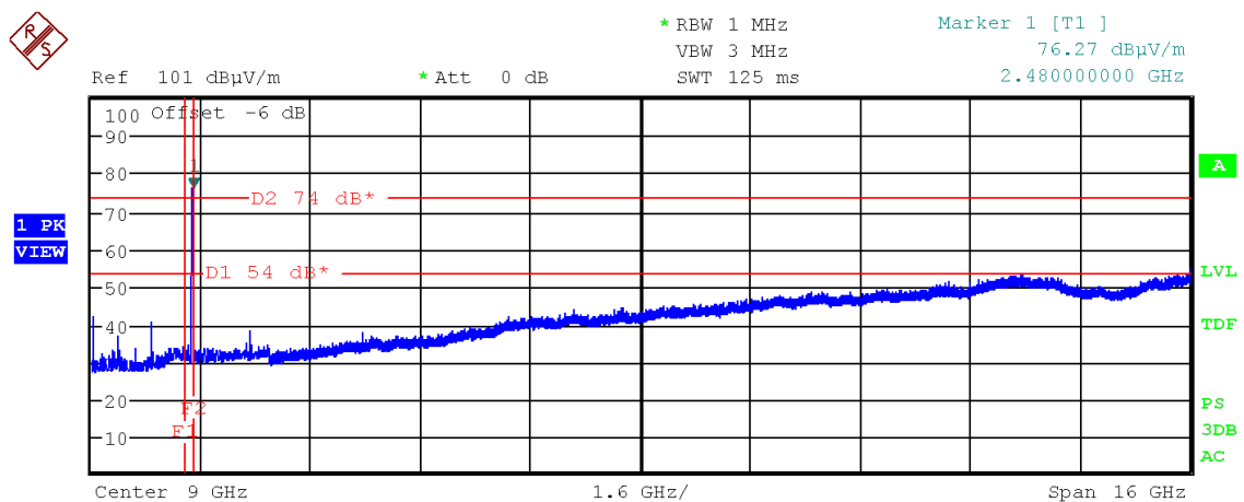
Figure 86: Chart of emissions test from 1 GHz to 17 GHz on highest channel, 1 Mbps, EUT position Y, antenna polarization horizontal
