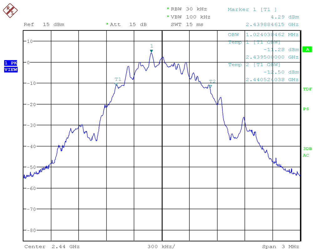
Figure 21: Chart of occupied bandwidth test on middle channel, 125 kbps
