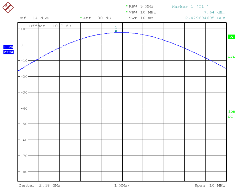
Figure 40: Chart of conducted output power on highest channel, 1 Mbps
