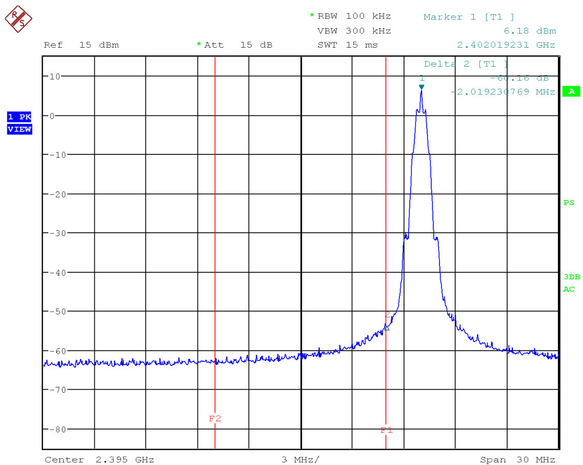
Figure 59: Chart of band-edge measurement on lowest channel, 500 kbps
