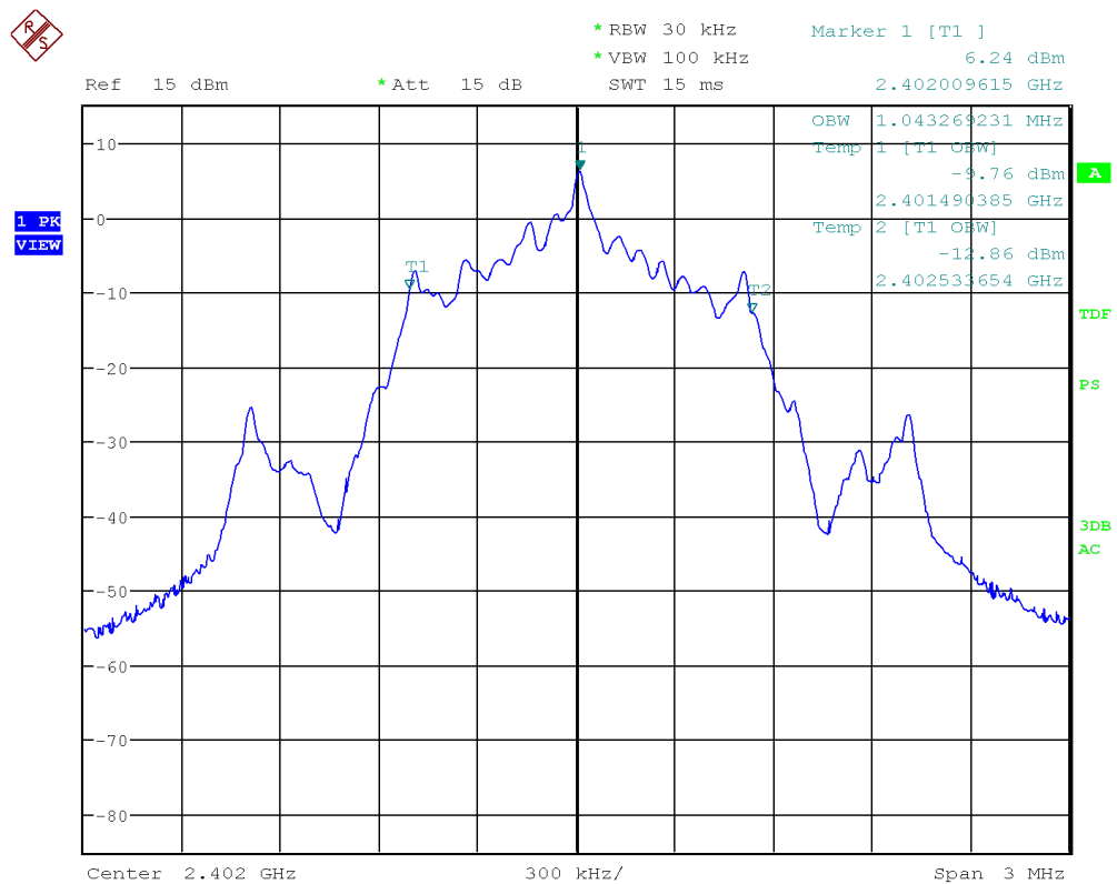
Figure 26: Chart of occupied bandwidth test on lowest channel, 1 Mbps
