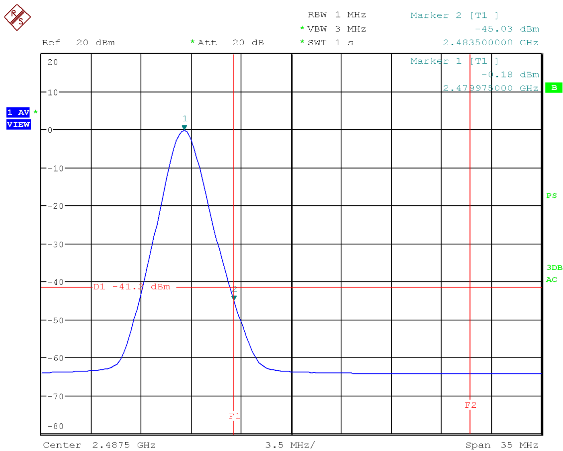
Figure 61: Chart of band-edge measurement on highest channel (AV), 500 kbps
