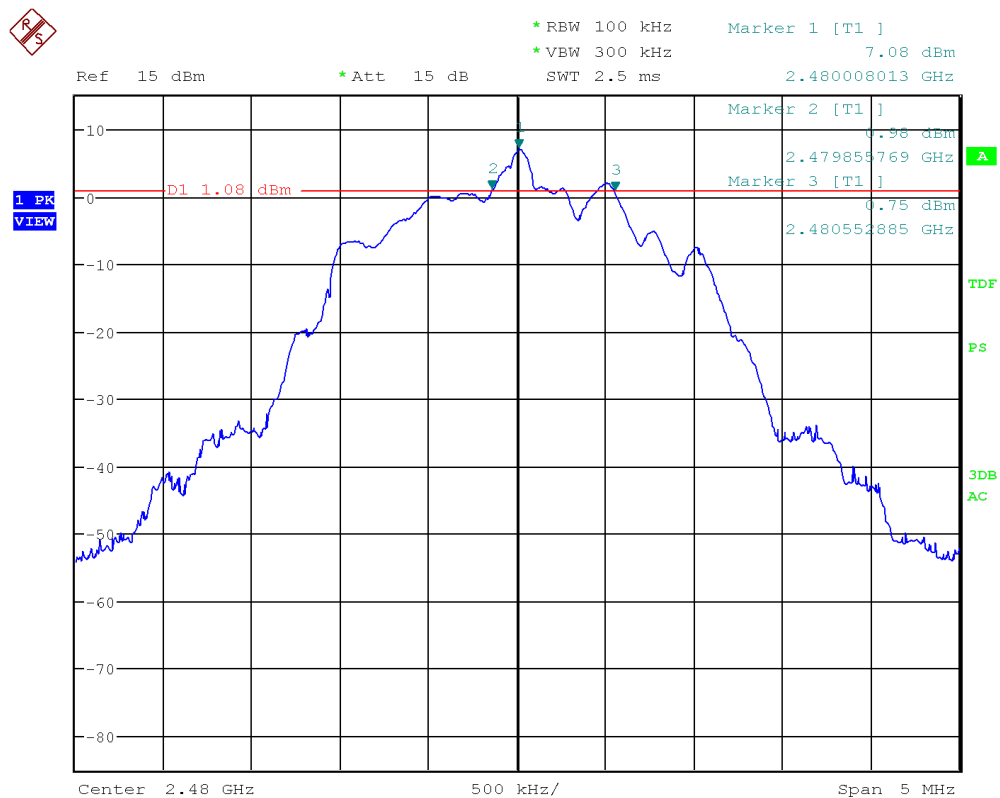
Figure 19: Chart of 6 dB bandwidth test on highest channel, 2 Mbps
