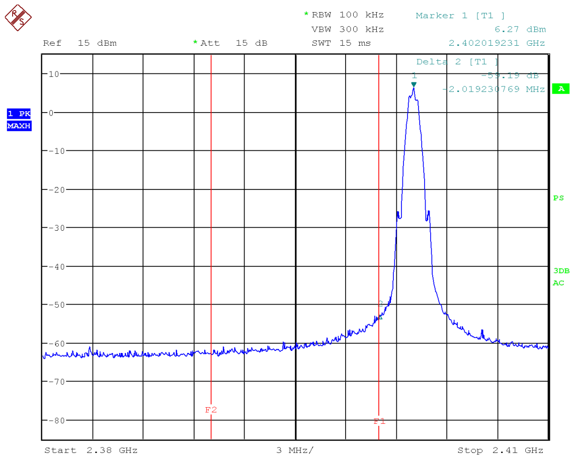
Figure 56: Chart of band-edge measurement on lowest channel, 125 kbps
