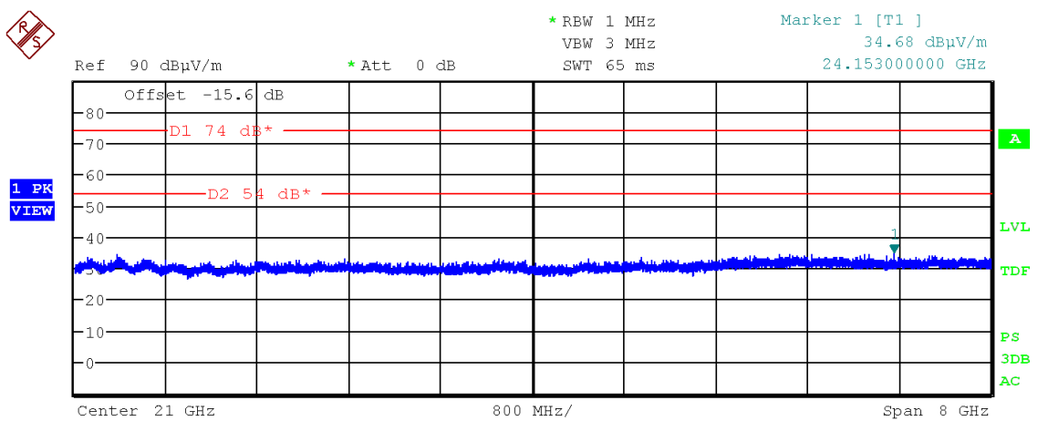
Figure 85: Chart of exploratory emissions measurement from 17 GHz to 25 GHz on middle channel, 1 Mbps
