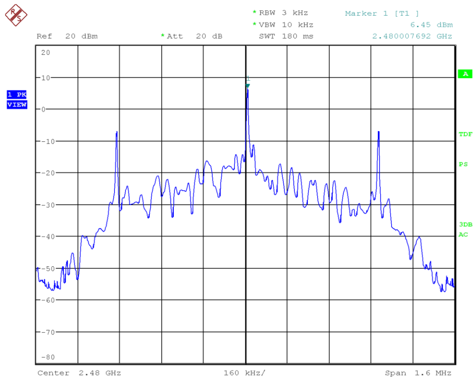
Figure 52: Chart of power spectral density on highest channel, 1 Mbps
