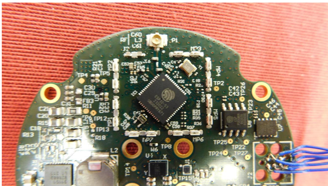
Picture 11: EUT without shielding – detailed view
