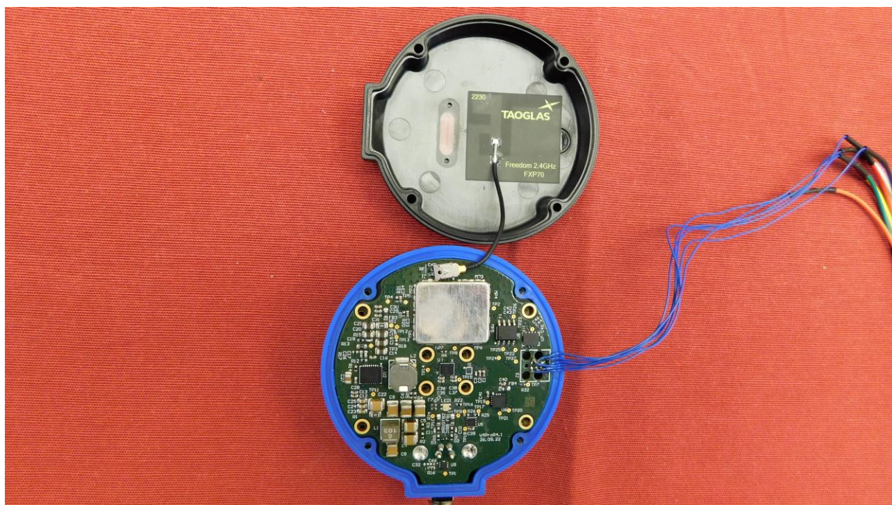
Picture 1: EUT without cover – top view
