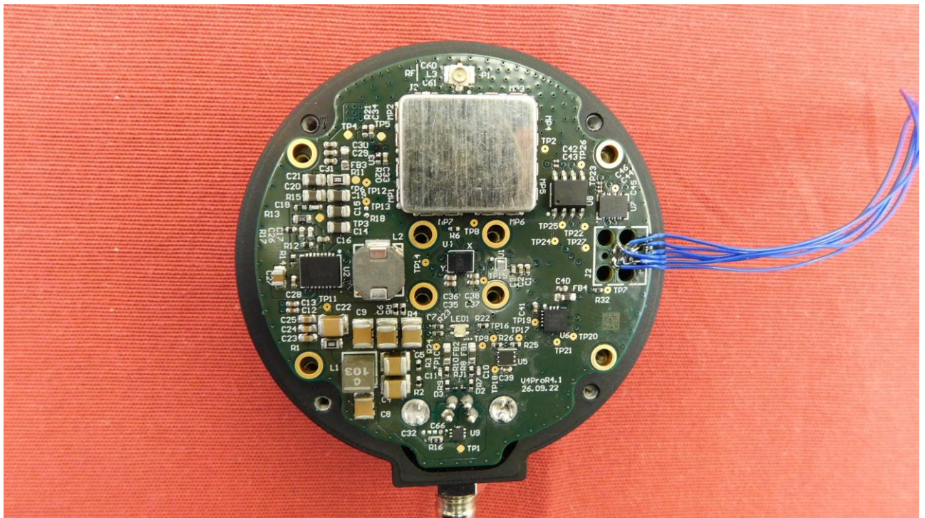
Picture 5: EUT without seal ring – top view
