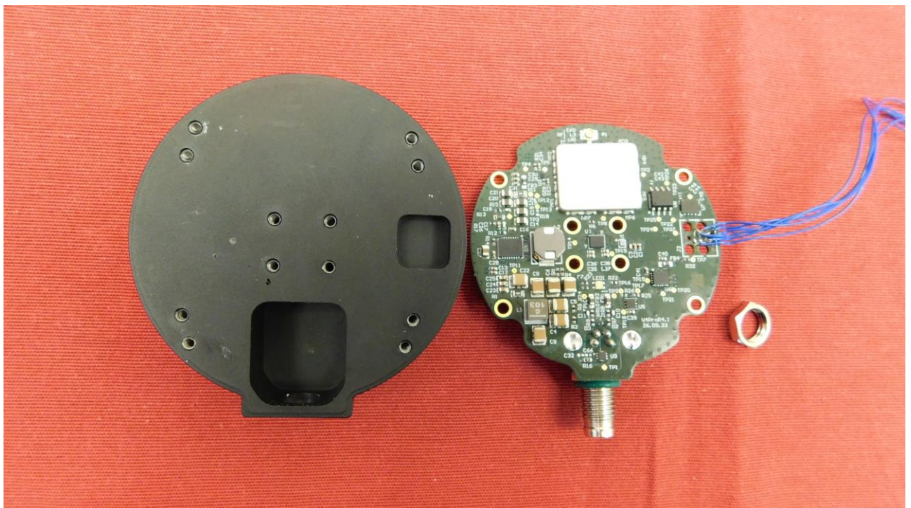
Picture 6: EUT without housing – top view
