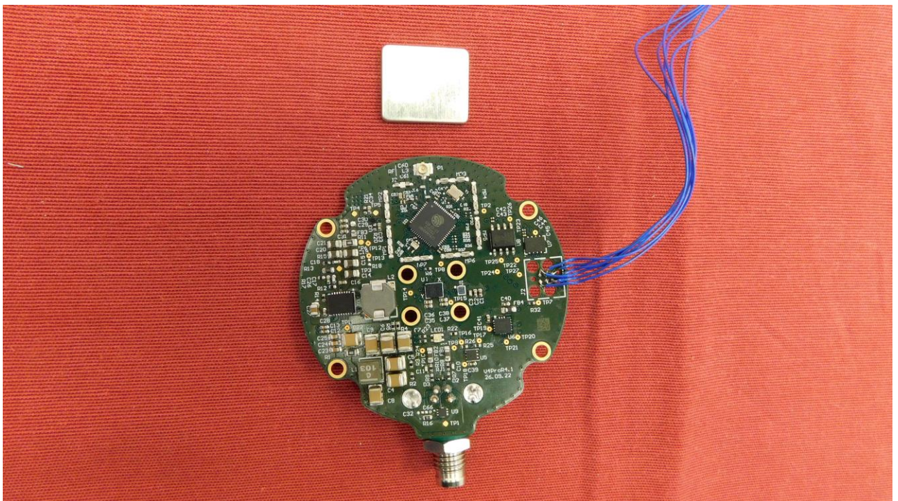
Picture 10: EUT without shielding– top view
