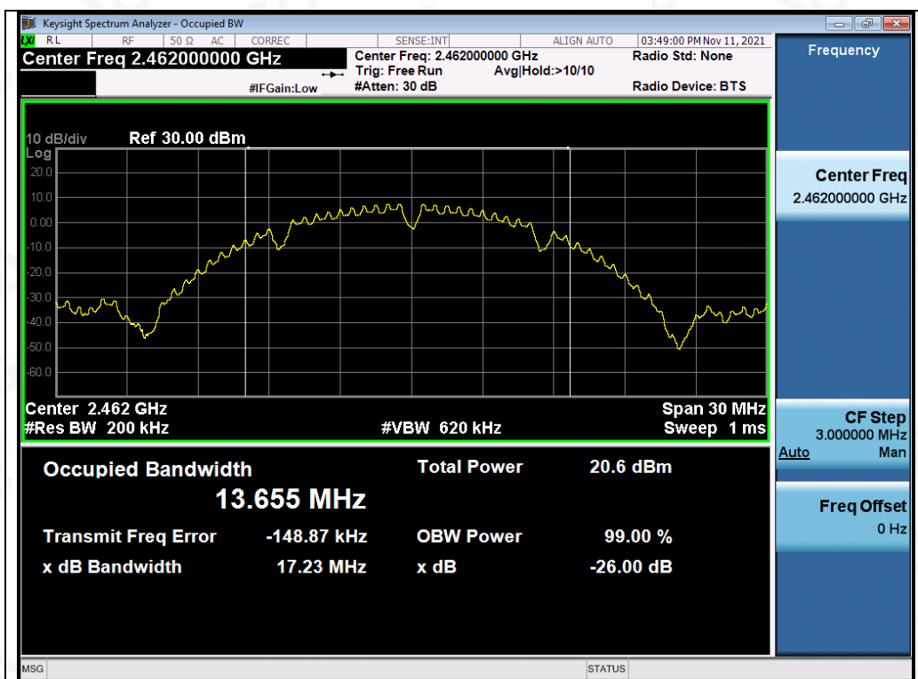
Test Graph 802.11b ANT1 2462 1Mbps OBW
