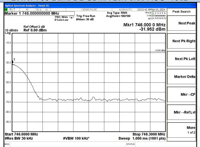
Lower 700 Band DL-CDMA Right Side AGC+10dB
