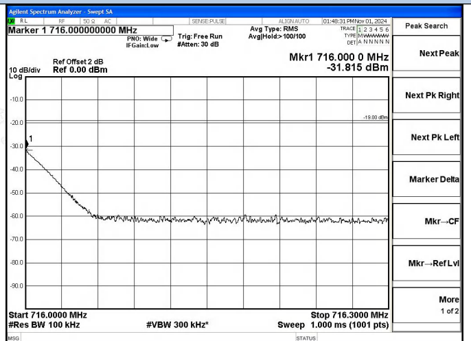
Lower 700 Band UL-LTE Right Side AGC+10dB
