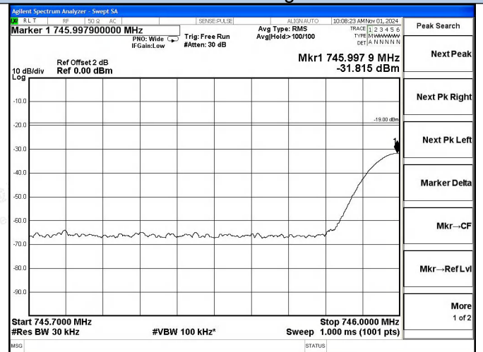
Upper 700 Band DL-CDMA Left Side AGC+10dB
