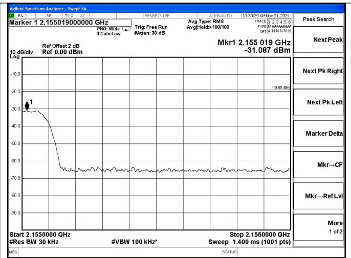
AWS Band DL-CDMA Right Side AGC+10dB
