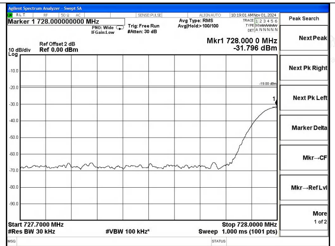
Lower 700 Band DL-CDMA Left Side AGC+10dB
