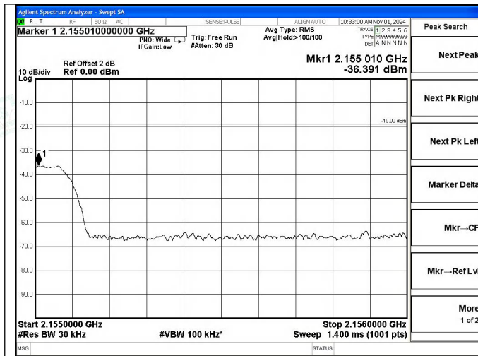
AWS Band DL-CDMA Right Side Pre AGC
