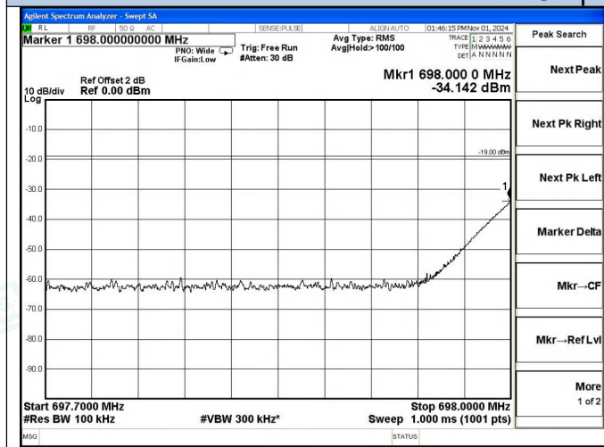
Lower 700 Band UL-LTE Left Side Pre AGC
