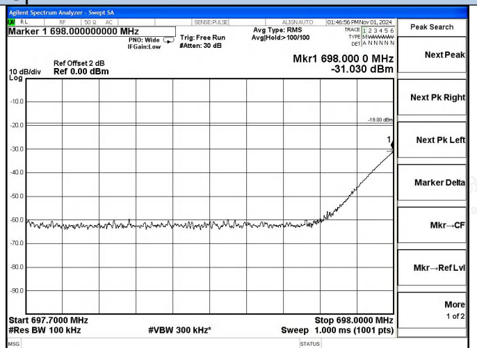
Lower 700 Band UL-LTE Left Side AGC+10dB
