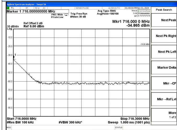
Lower 700 Band UL-LTE Right Side Pre AGC
