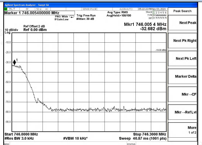
Lower 700 Band DL-GSM Right Side AGC+10dB
