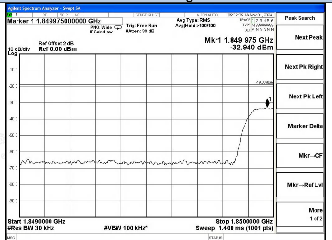
PCS Band UL-CDMA Left Side AGC+5.5dB
