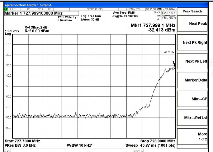
Lower 700 Band DL-GSM Left Side AGC+10dB
