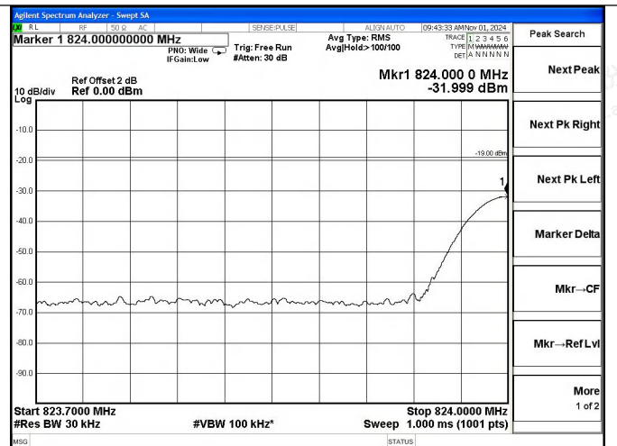
Cellular Band UL-CDMA Left Side AGC+10dB
