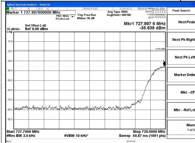
Lower 700 Band DL-GSM Left Side Pre AGC
