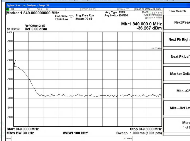
Cellular Band UL-CDMA Right Side Pre AGC
