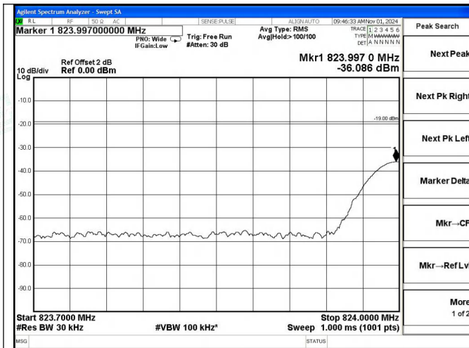
Cellular Band UL-CDMA Left Side Pre AGC
