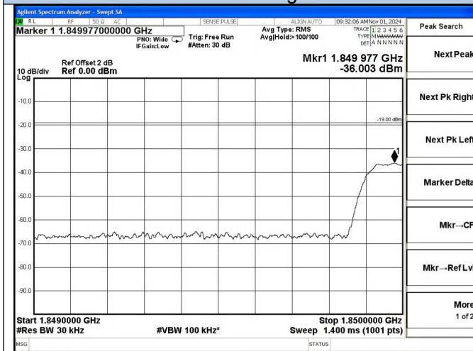
PCS Band UL-CDMA Left Side Pre AGC
