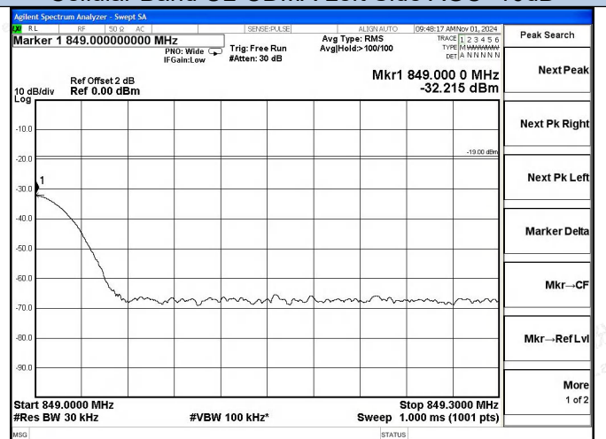
Cellular Band UL-CDMA Right Side AGC+10dB
