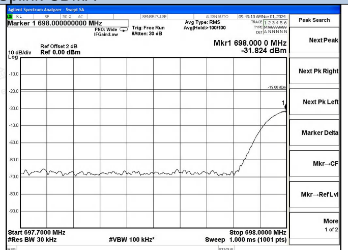
Lower 700 Band UL-CDMA Left Side AGC+10dB
