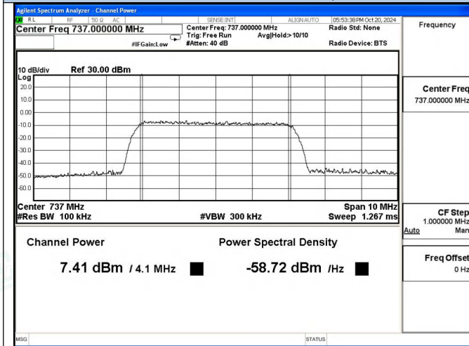
Lower 700 Band AWGN, DL
