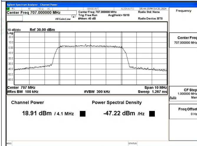
Lower 700 Band AWGN, UL
