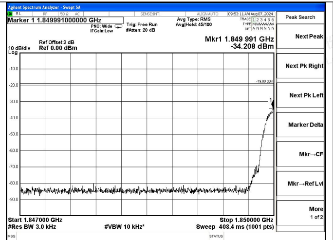
PCS Band UL-GSM Left Side AGC+5.5dB
