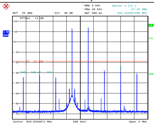
Cellular Band Uplink-Pre AGC
