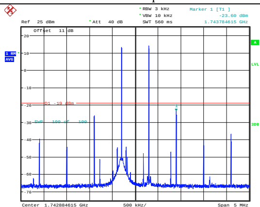
AWS-1 Band Uplink-Pre AGC
