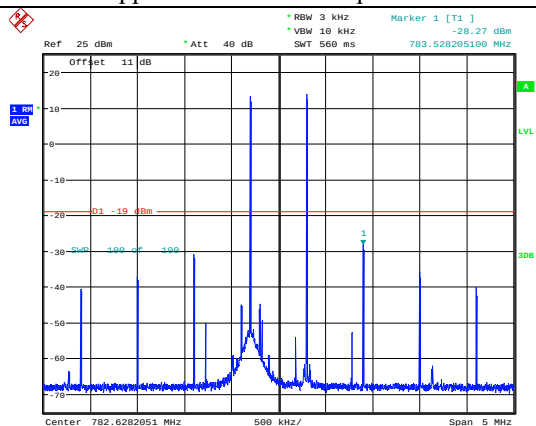
Upper 700MHz Band Uplink-Pre AGC
