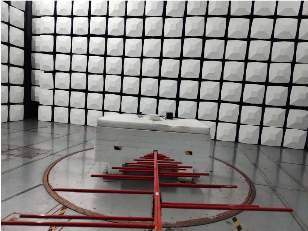
Model: SF006B Radiated Emission Below 1GHz View-Downlink
