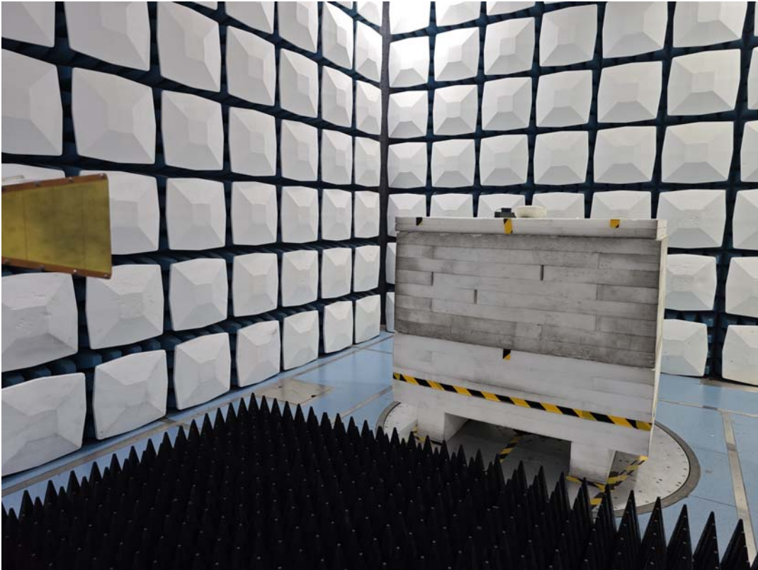
Model: SF006B Radiated Emission Above 1GHz View-Downlink
