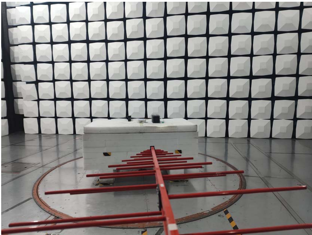
Model: SF006A Radiated Emission Below 1GHz View-Downlink
