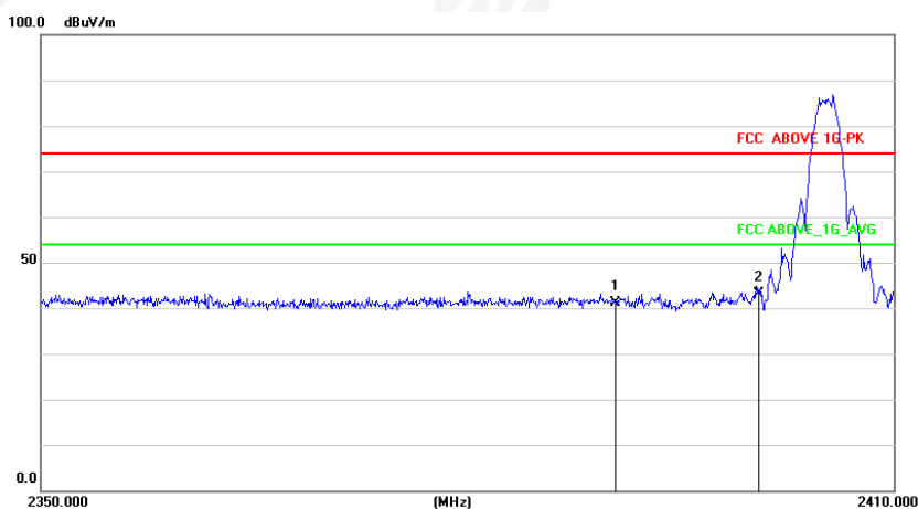
2402MHz Horizontal
