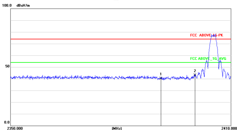
2402MHz Vertical
