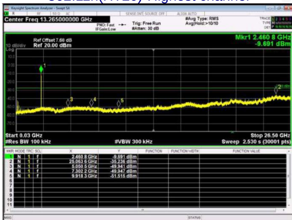
802.11n(HT20)-Highest channel
