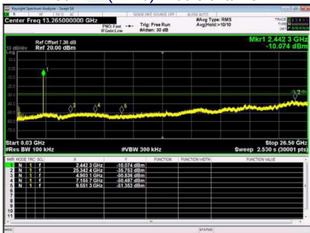
802.11n(HT20)-Middle channel
