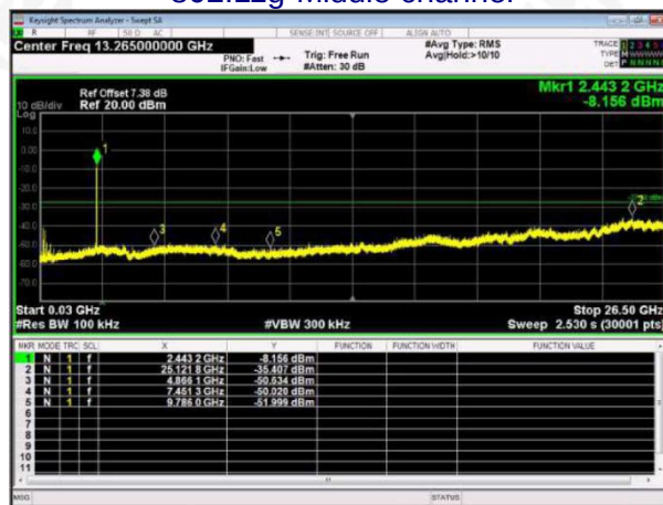
802.11g-Middle channel
