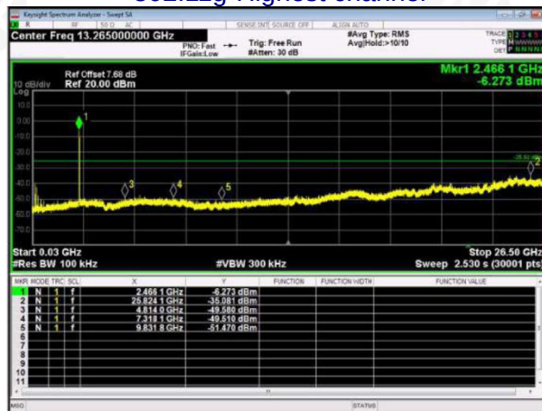
802.11g-Highest channel
