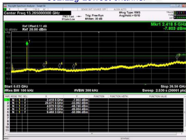
802.11g-Lowest channel
