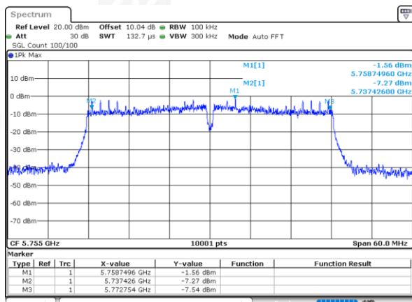
(802.11n40)6DB Bandwidth plot on channel 151
