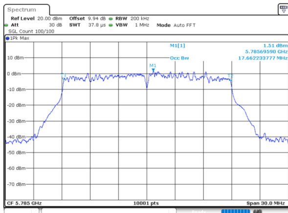
(802.11n20)99% Bandwidth plot on channel 157
