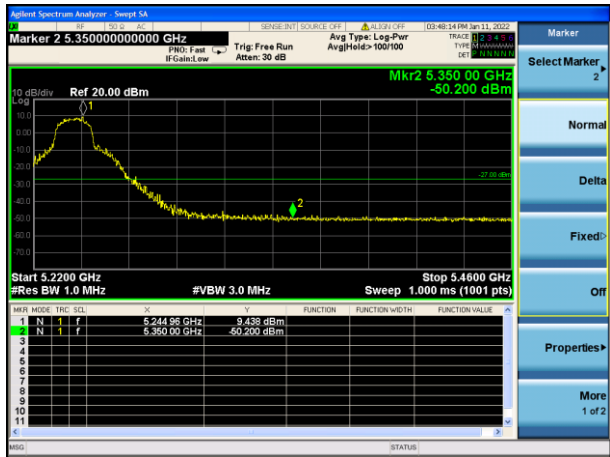
Right bandedge
