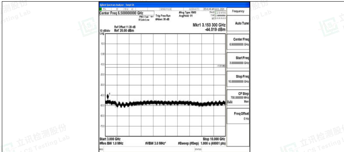
Band71_5MHz_16QAM_133447_1RB#0_3000~10000_3000~10000
