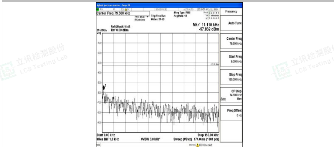
Band71_15MHz_QPSK_133297_1RB#0_0.009~0.15_0.009~0.15
