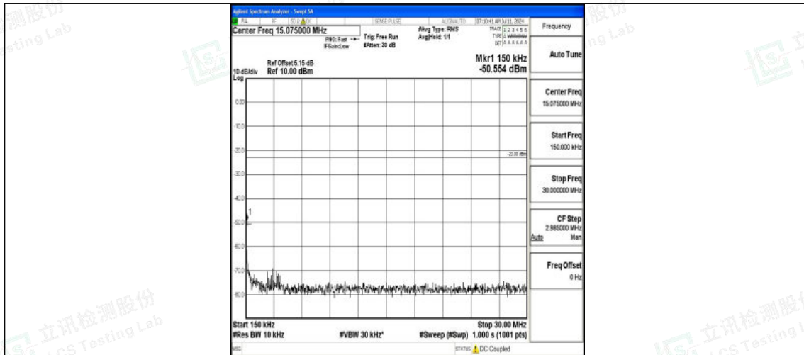
Band71_20MHz_QPSK_133322_1RB#0_0.15~30_0.15~30
