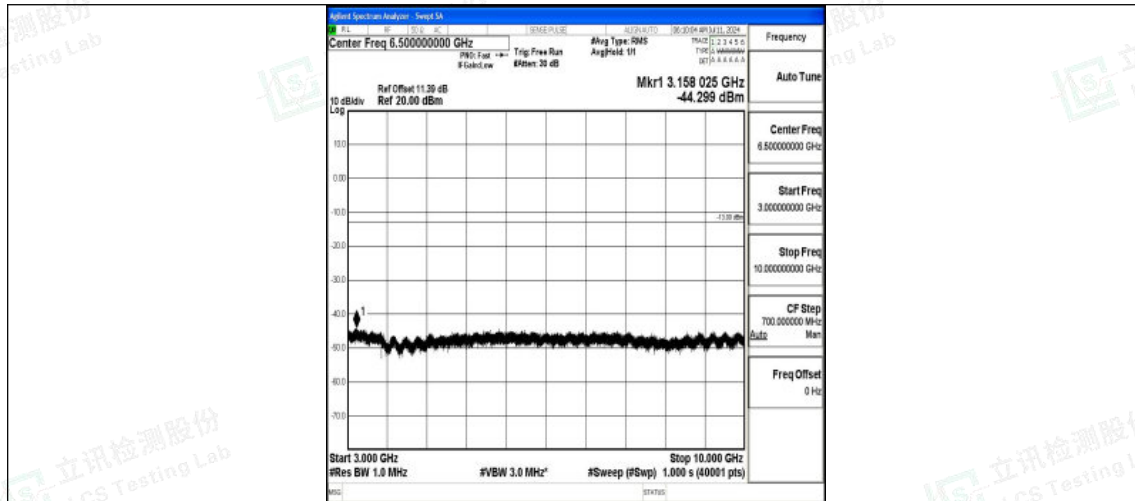
Band71_10MHz_QPSK_133297_1RB#0_3000~10000_3000~10000
