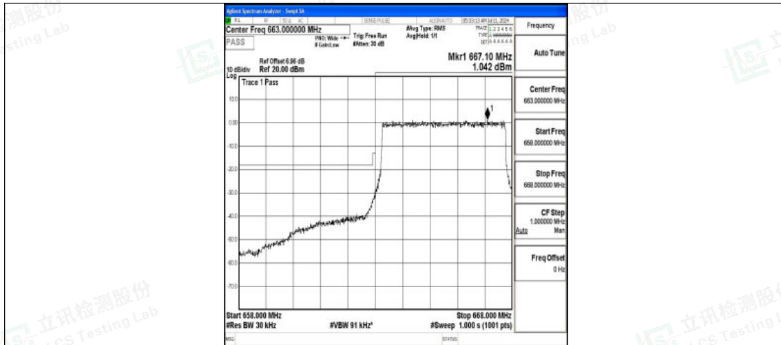
Band71_5MHz_16QAM_133147_25RB#0
