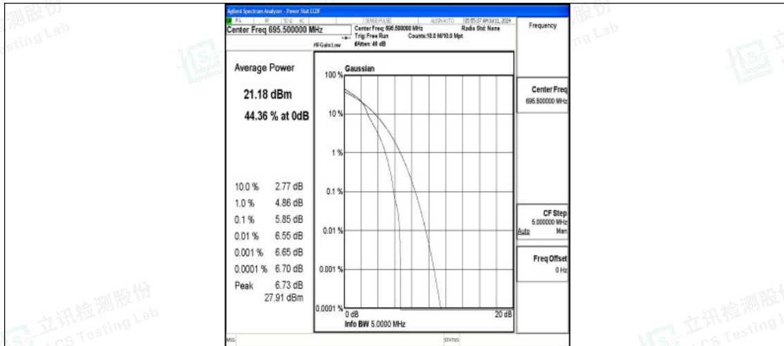
Band71-5MHz-16QAM-133447-1RB#0-PASS
