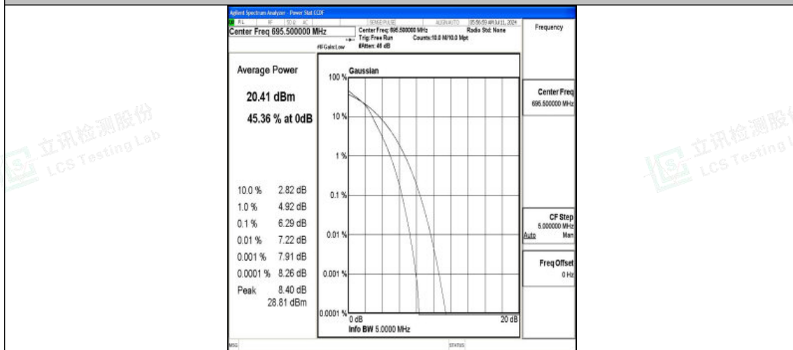
Band71-5MHz-16QAM-133447-25RB#0-PASS
