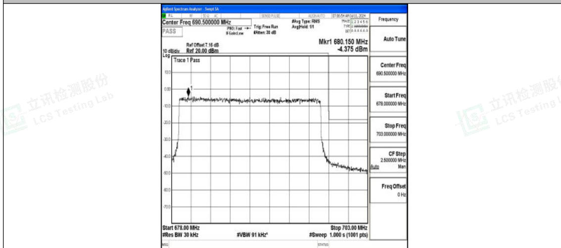
Band71_20MHz_16QAM_133372_100RB#0
