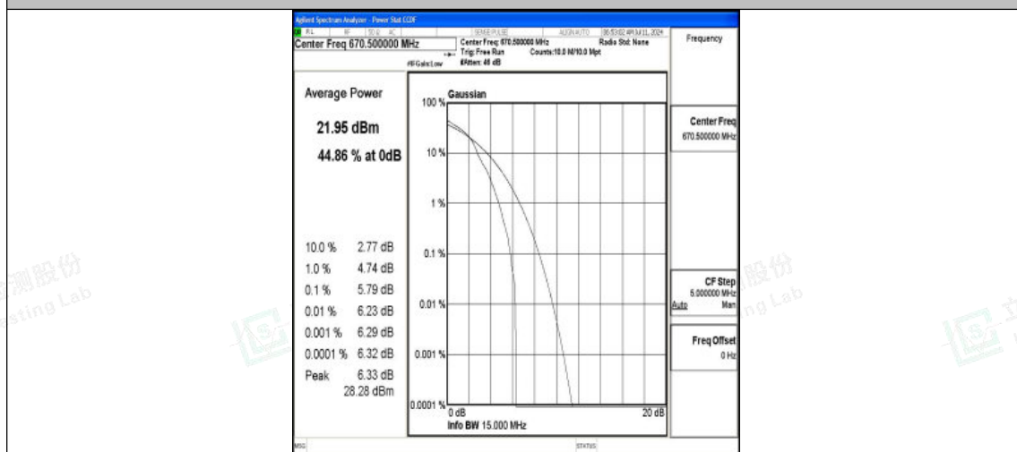
Band71-15MHz-16QAM-133197-1RB#0-PASS
