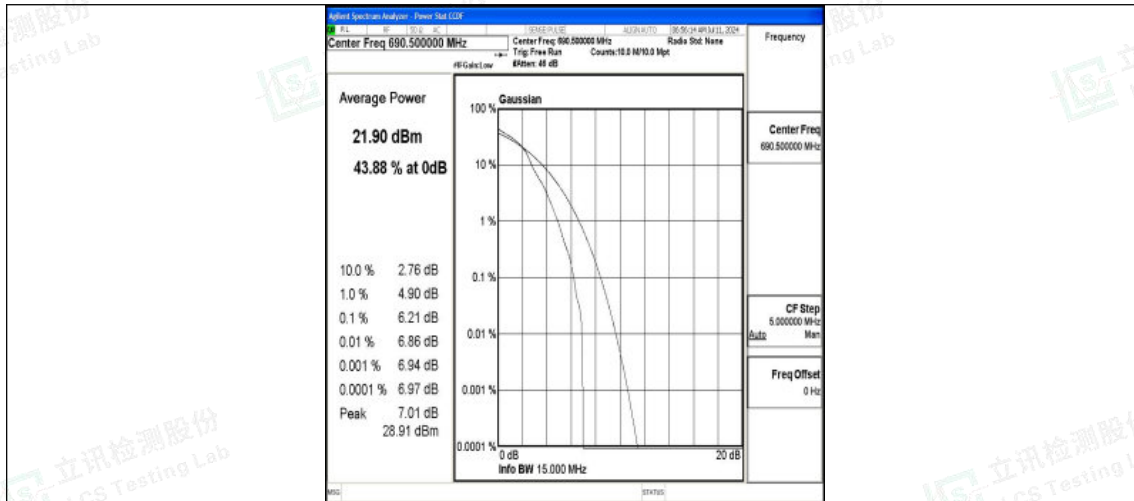
Band71-15MHz-16QAM-133397-1RB#0-PASS
