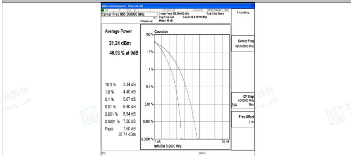
Band71-5MHz-QPSK-133447-25RB#0-PASS
