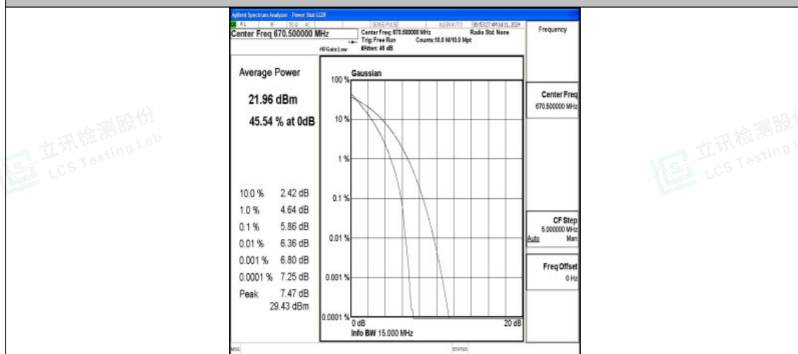
Band71-15MHz-QPSK-133197-75RB#0-PASS
