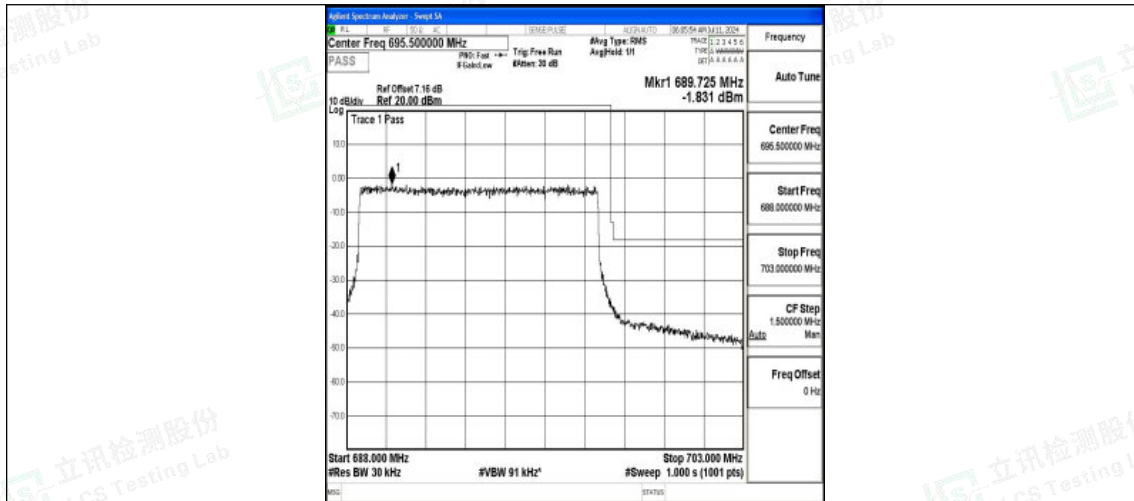
Band71_10MHz_16QAM_133422_50RB#0
