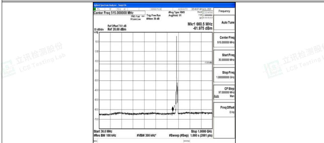
Band71_5MHz_QPSK_133447_1RB#0_30~1000_30~1000
