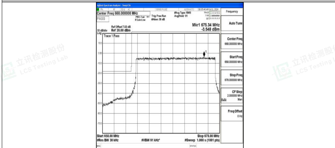
Band71_15MHz_16QAM_133197_75RB#0
