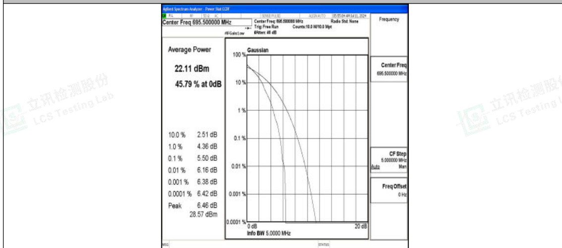
Band71-5MHz-QPSK-133447-1RB#0-PASS
