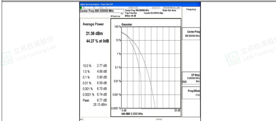
Band71-5MHz-16QAM-133297-1RB#0-PASS
