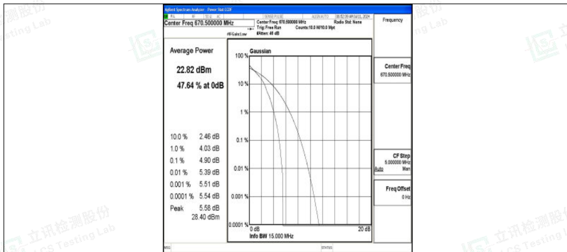
Band71-15MHz-QPSK-133197-1RB#0-PASS
