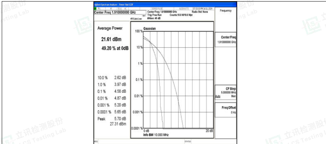
Band25-10MHz-16QAM-26640-1RB#0-PASS
