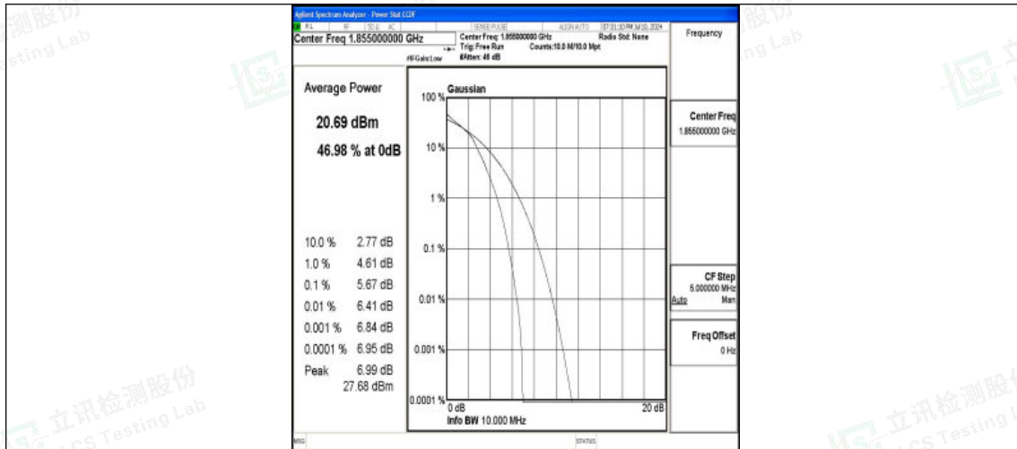
Band25-10MHz-16QAM-26090-50RB#0-PASS
