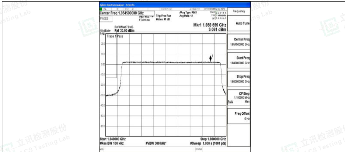
Band25_10MHz_QPSK_26090_50RB#0
