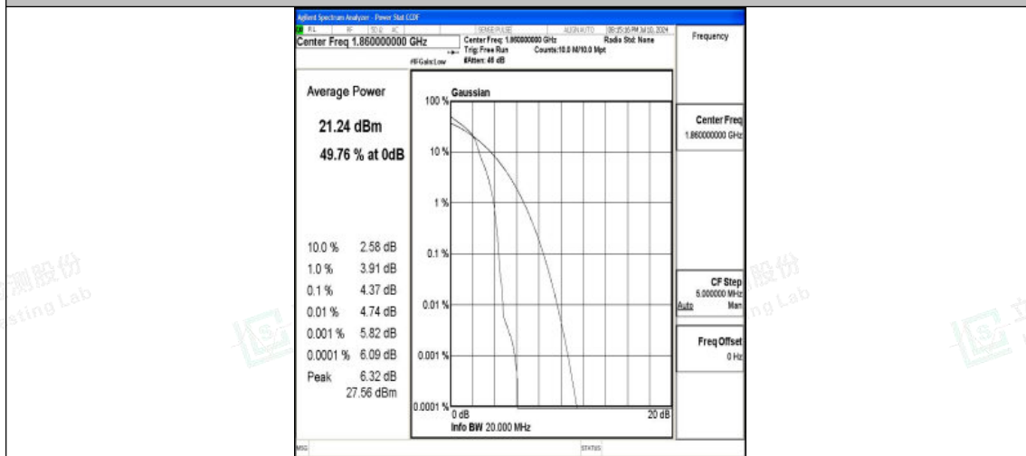
Band25-20MHz-16QAM-26140-1RB#0-PASS
