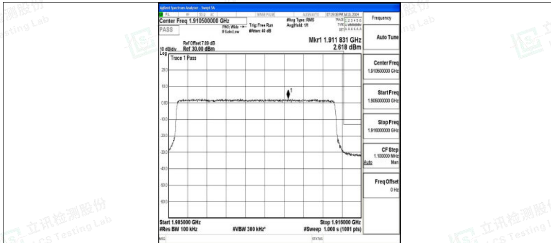
Band25_10MHz_16QAM_26640_50RB#0
