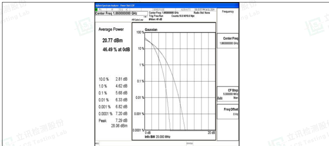
Band25-20MHz-16QAM-26140-100RB#0-PASS
