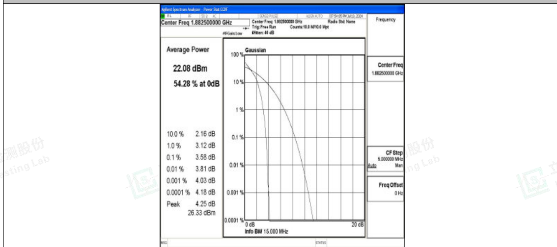
Band25-15MHz-QPSK-26365-1RB#0-PASS
