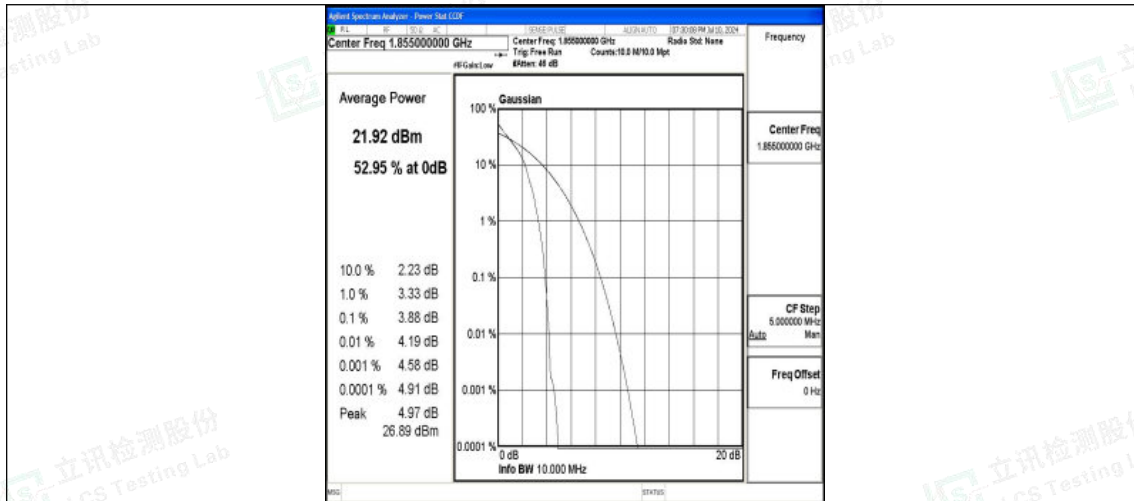
Band25-10MHz-QPSK-26090-1RB#0-PASS
