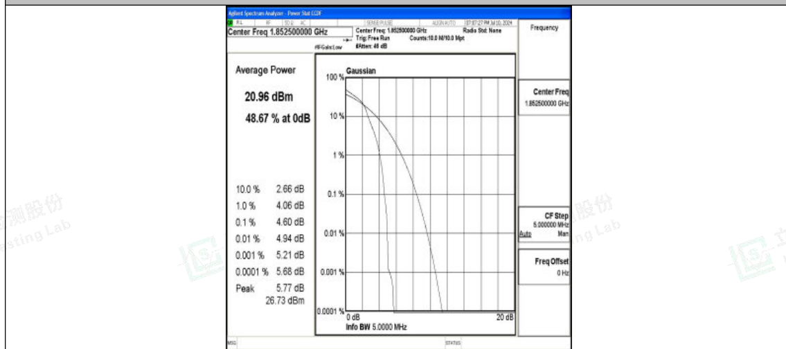
Band25-5MHz-16QAM-26065-1RB#0-PASS
