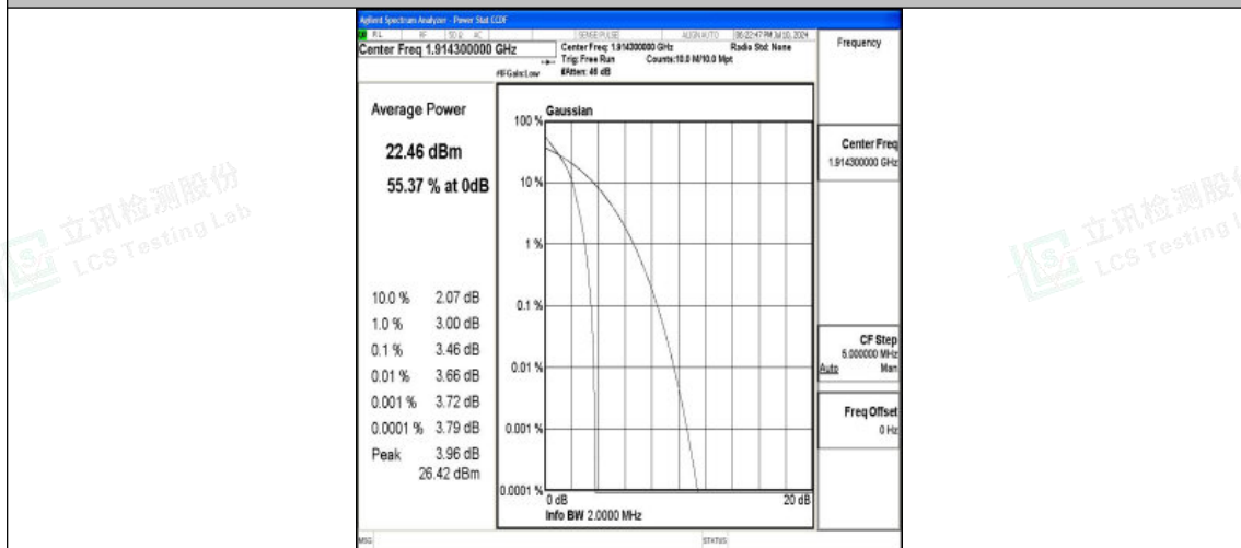
Band25-1.4MHz-QPSK-26683-1RB#0-PASS
