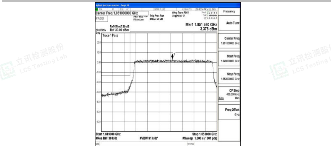
Band25_3MHz_16QAM_26055_15RB#0
