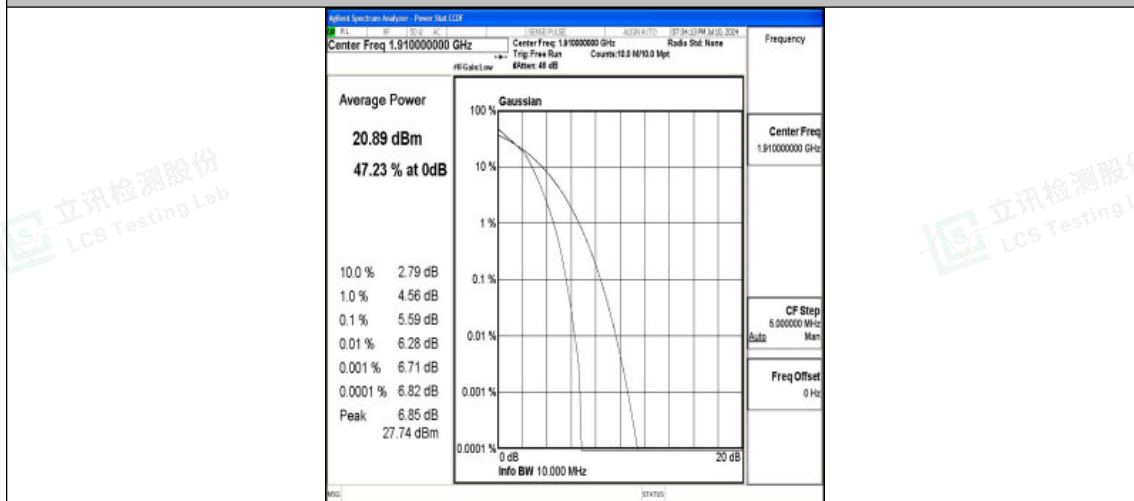
Band25-10MHz-16QAM-26640-50RB#0-PASS
