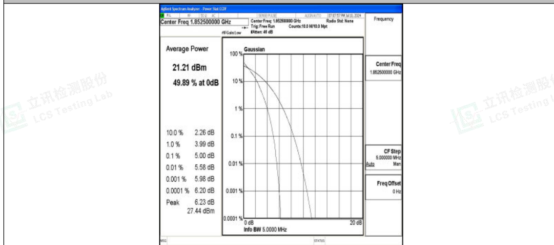
Band25-5MHz-QPSK-26065-25RB#0-PASS
