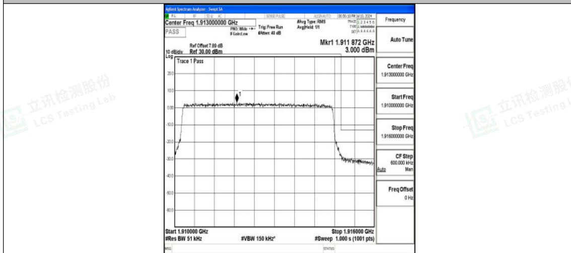
Band25_5MHz_16QAM_26665_25RB#0
