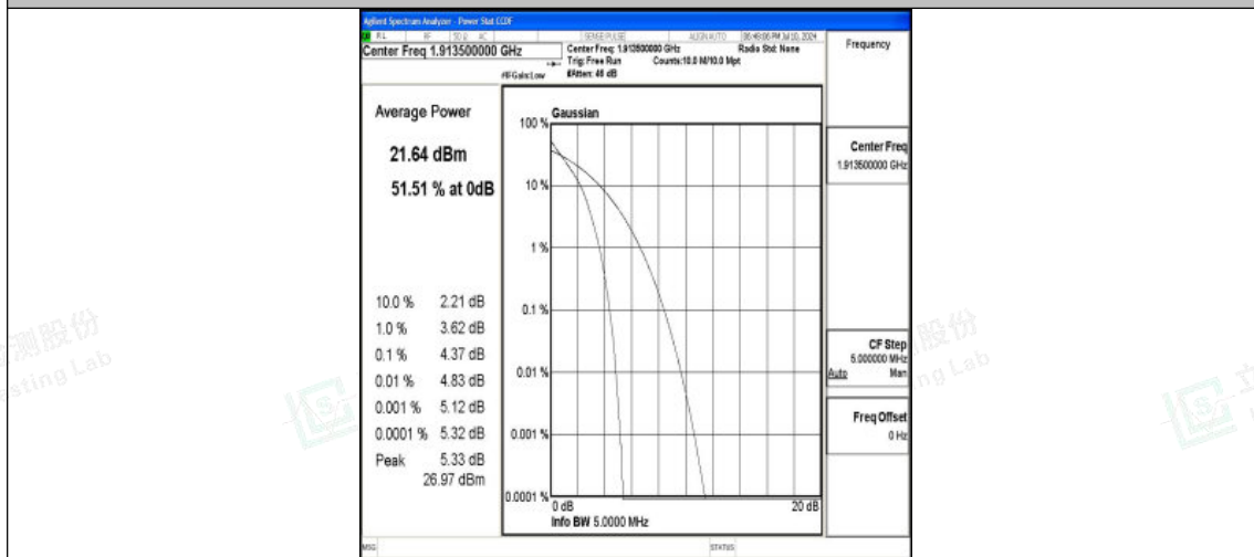
Band25-3MHz-QPSK-26675-15RB#0-PASS
