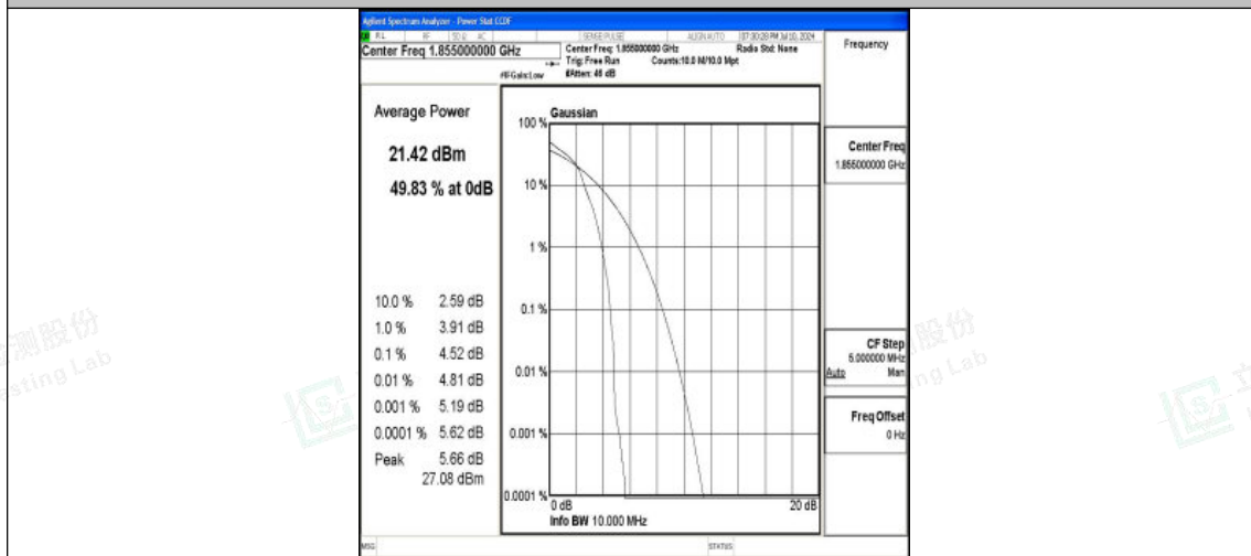
Band25-10MHz-16QAM-26090-1RB#0-PASS
