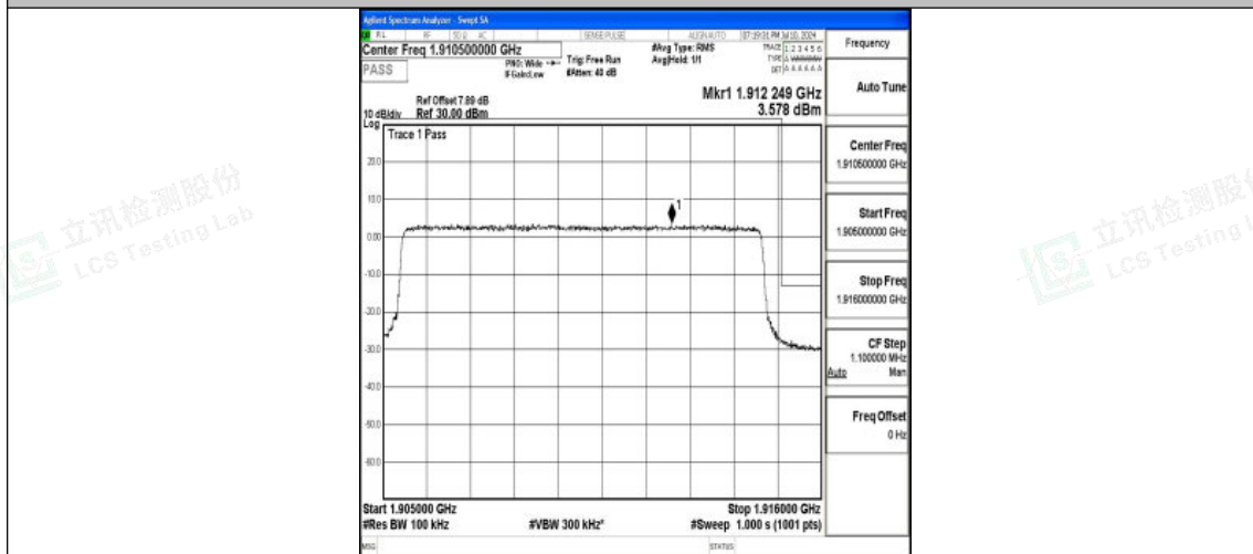
Band25_10MHz_QPSK_26640_50RB#0
