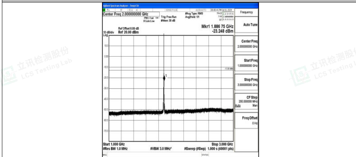
Band25_1.4MHz_16QAM_26365_1RB#0_1000~3000_1000~3000
