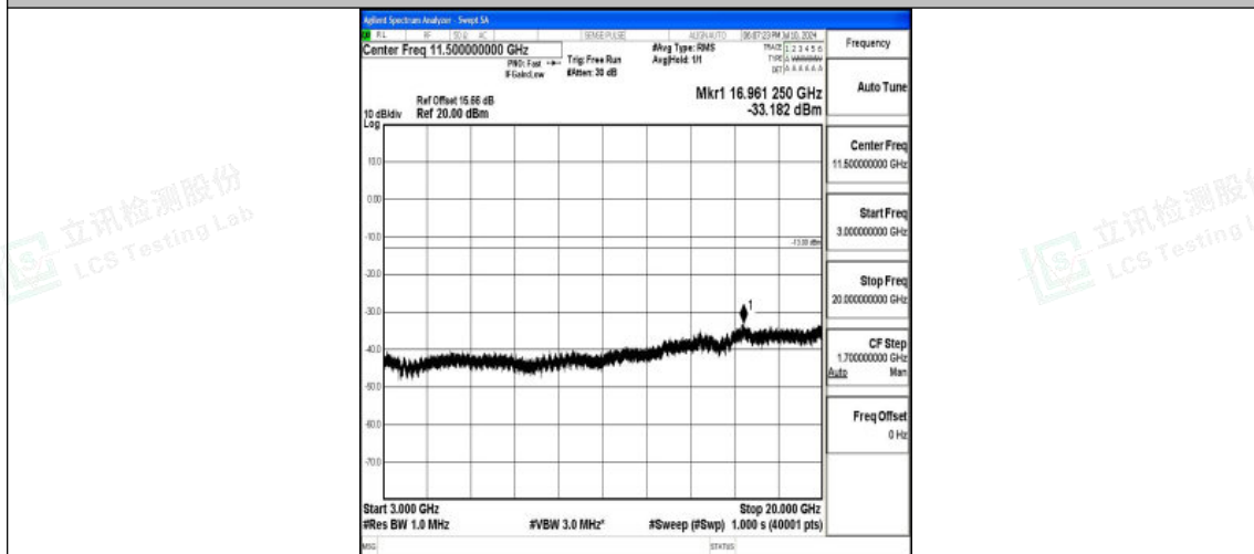
Band25_1.4MHz_QPSK_26683_1RB#0_3000~20000_3000~20000
