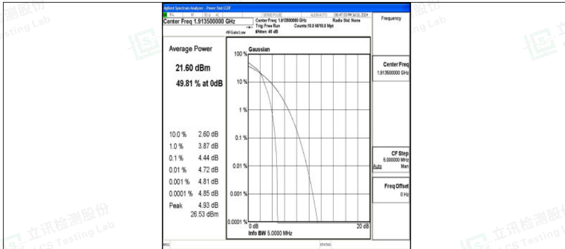
Band25-3MHz-16QAM-26675-1RB#0-PASS
