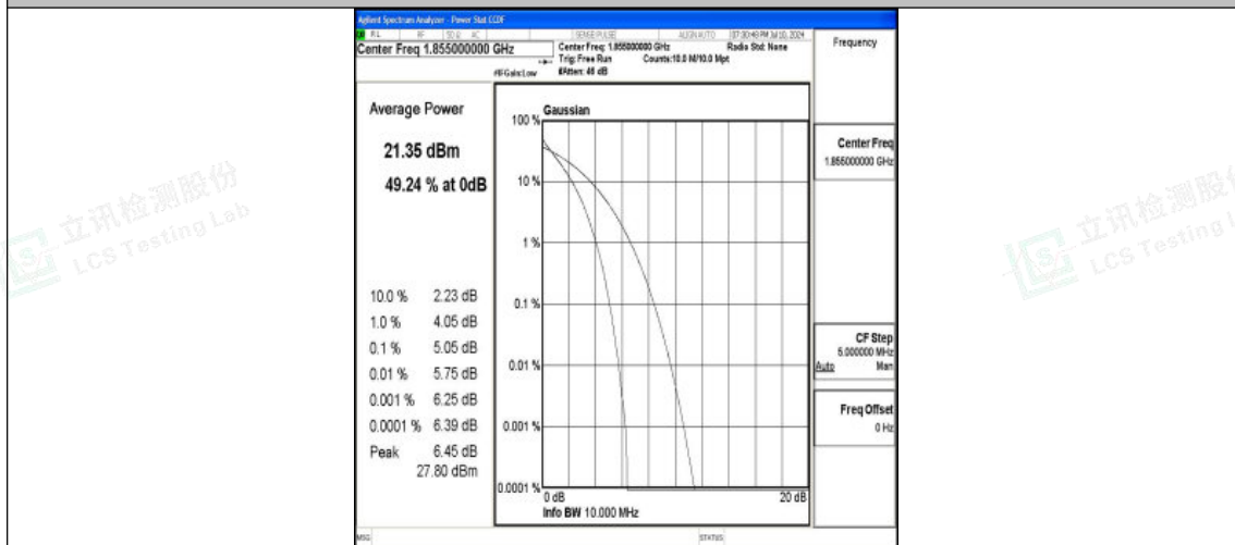
Band25-10MHz-QPSK-26090-50RB#0-PASS
