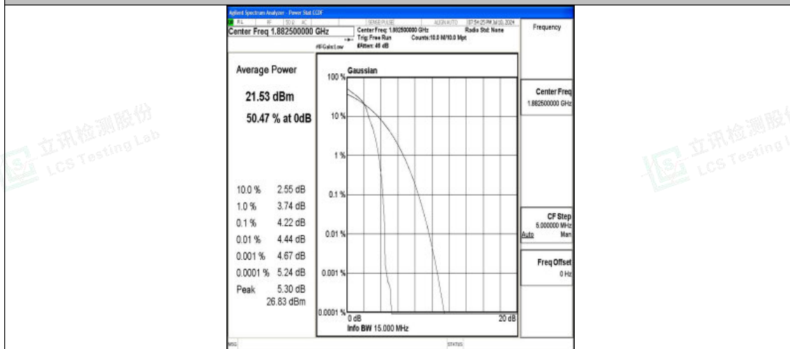
Band25-15MHz-16QAM-26365-1RB#0-PASS
