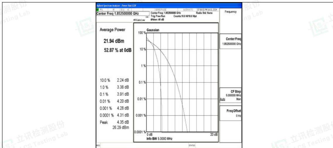
Band25-5MHz-QPSK-26065-1RB#0-PASS
