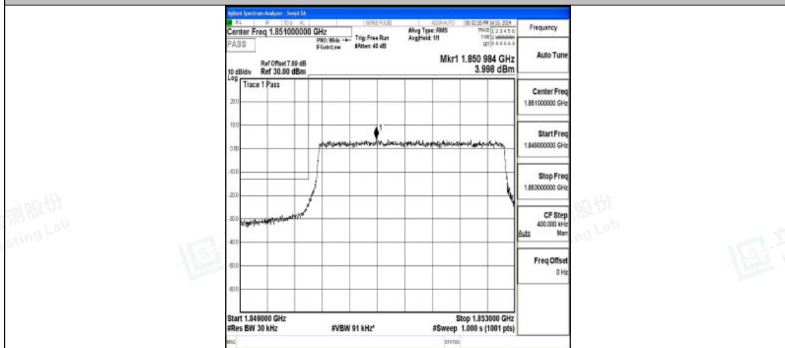
Band25_3MHz_QPSK_26055_15RB#0
