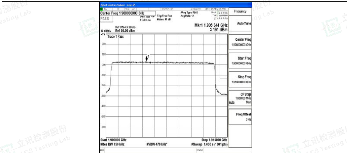
Band25_15MHz_QPSK_26615_75RB#0
