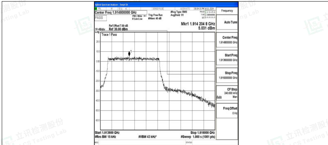
Band25_1.4MHz_16QAM_26683_6RB#0
