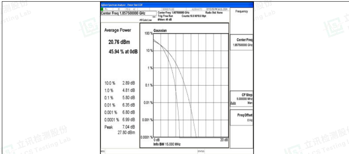
Band25-15MHz-16QAM-26115-75RB#0-PASS
