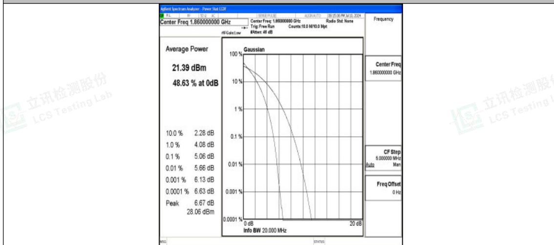
Band25-20MHz-QPSK-26140-100RB#0-PASS
