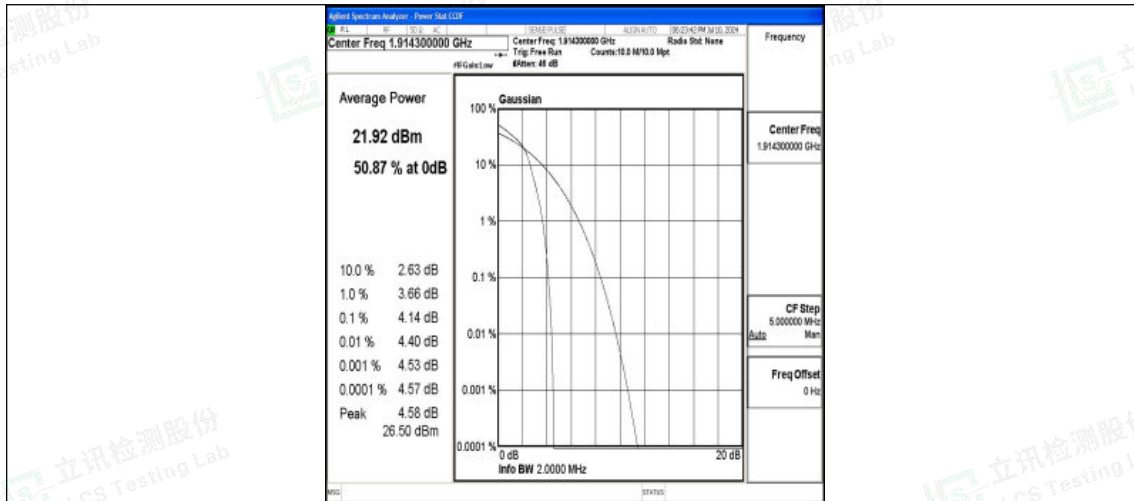
Band25-1.4MHz-16QAM-26683-1RB#0-PASS
