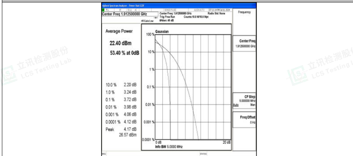
Band25-5MHz-QPSK-26665-1RB#0-PASS
