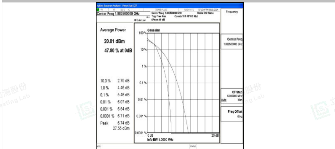
Band25-5MHz-16QAM-26365-25RB#0-PASS
