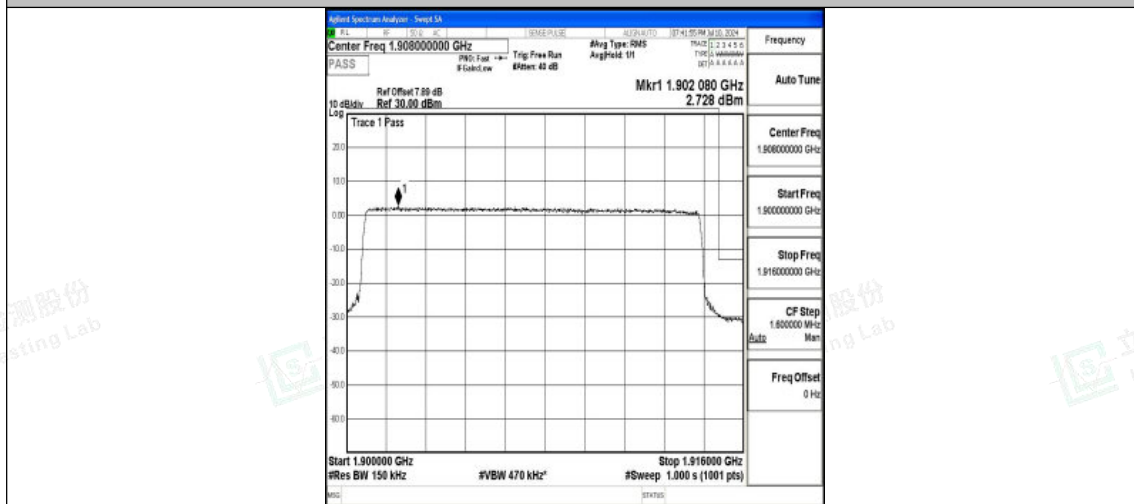
Band25_15MHz_16QAM_26615_75RB#0
