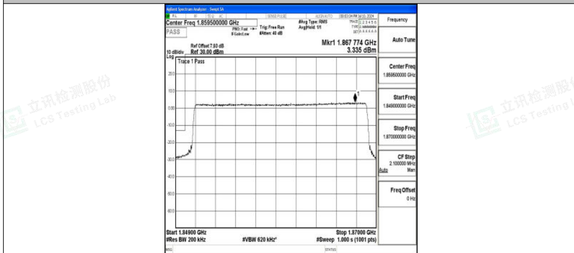
Band25_20MHz_QPSK_26140_100RB#0
