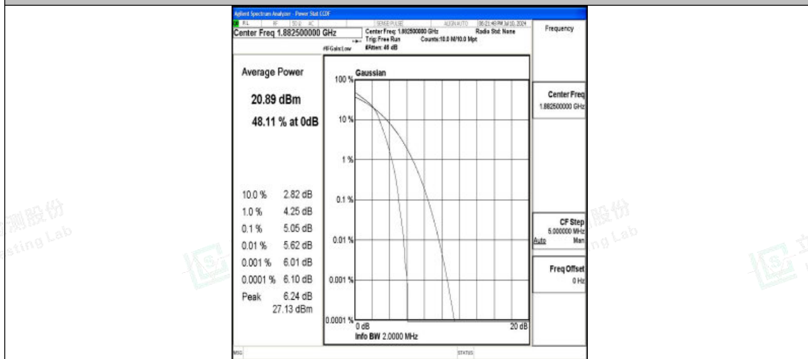
Band25-1.4MHz-16QAM-26365-6RB#0-PASS
