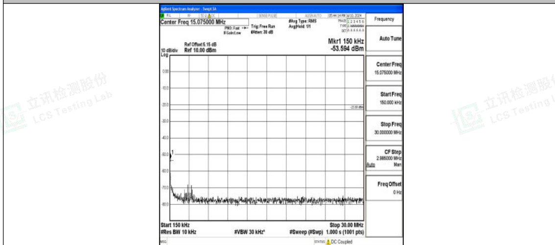
Band12_10MHz_QPSK_23060_1RB#0_0.15~30_0.15~30
