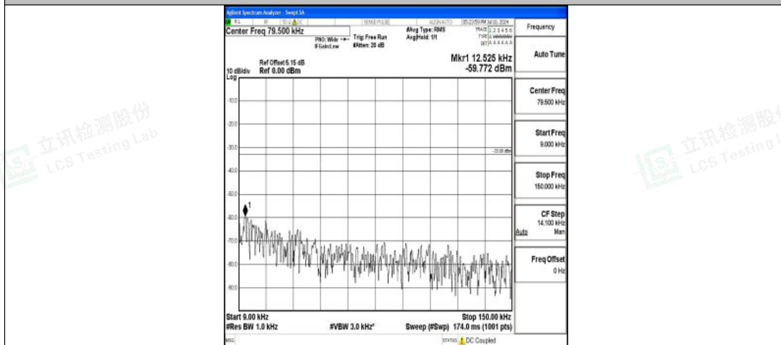
Band12_5MHz_16QAM_23155_1RB#0_0.009~0.15_0.009~0.15
