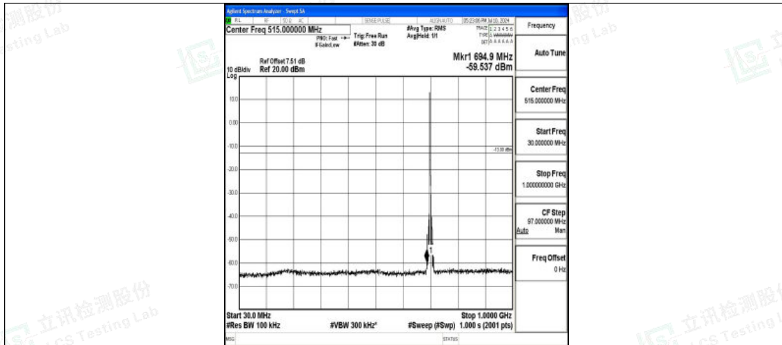
Band12_5MHz_16QAM_23095_1RB#0_30~1000_30~1000
