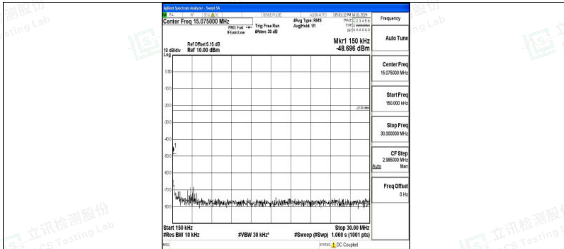
Band12_3MHz_16QAM_23165_1RB#0_0.15~30_0.15~30
