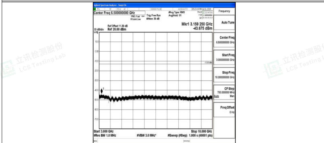
Band12_5MHz_16QAM_23095_1RB#0_3000~10000_3000~10000
