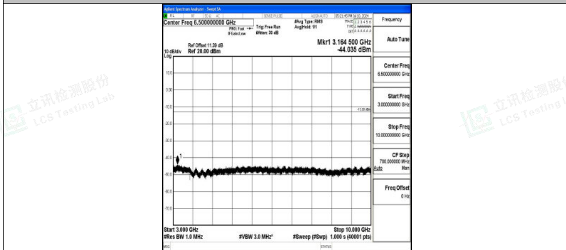
Band12_5MHz_QPSK_23035_1RB#0_3000~10000_3000~10000
