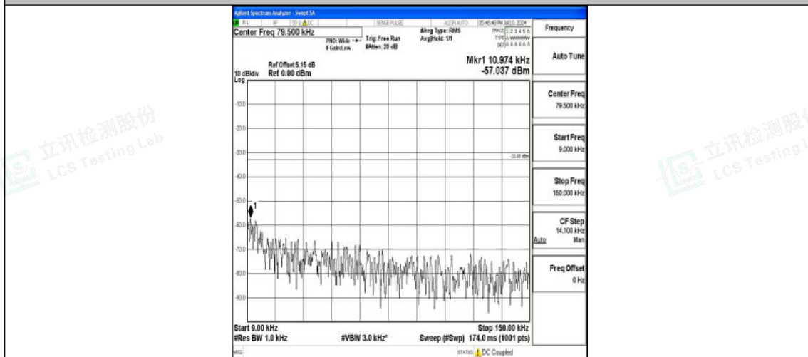
Band12_10MHz_16QAM_23130_1RB#0_0.009~0.15_0.009~0.15
