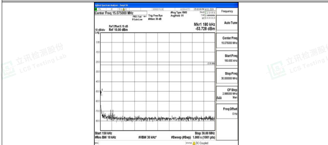
Band12_3MHz_16QAM_23095_1RB#0_0.15~30_0.15~30
