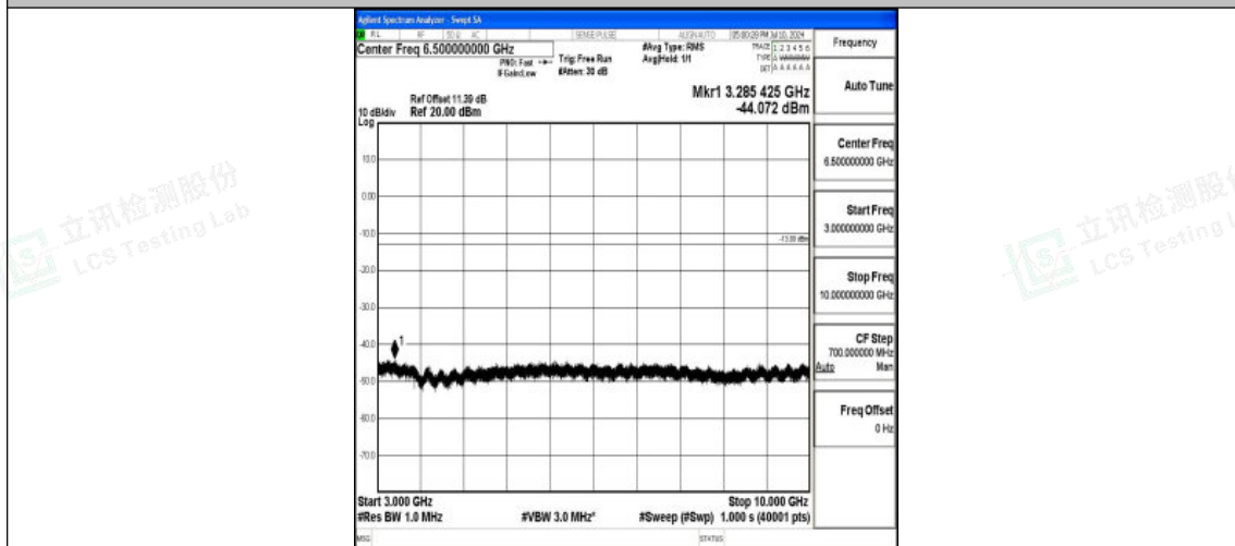
Band12_3MHz_16QAM_23095_1RB#0_3000~10000_3000~10000
