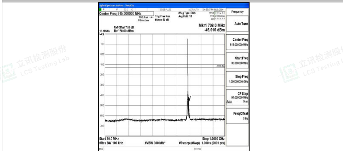
Band12_3MHz_16QAM_23025_1RB#0_30~1000_30~1000
