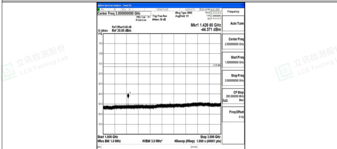
Band12_3MHz_16QAM_23165_1RB#0_1000~3000_1000~3000
