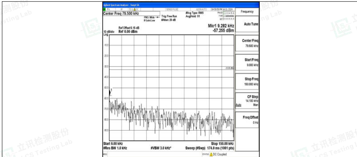
Band12_3MHz_16QAM_23025_1RB#0_0.009~0.15_0.009~0.15
