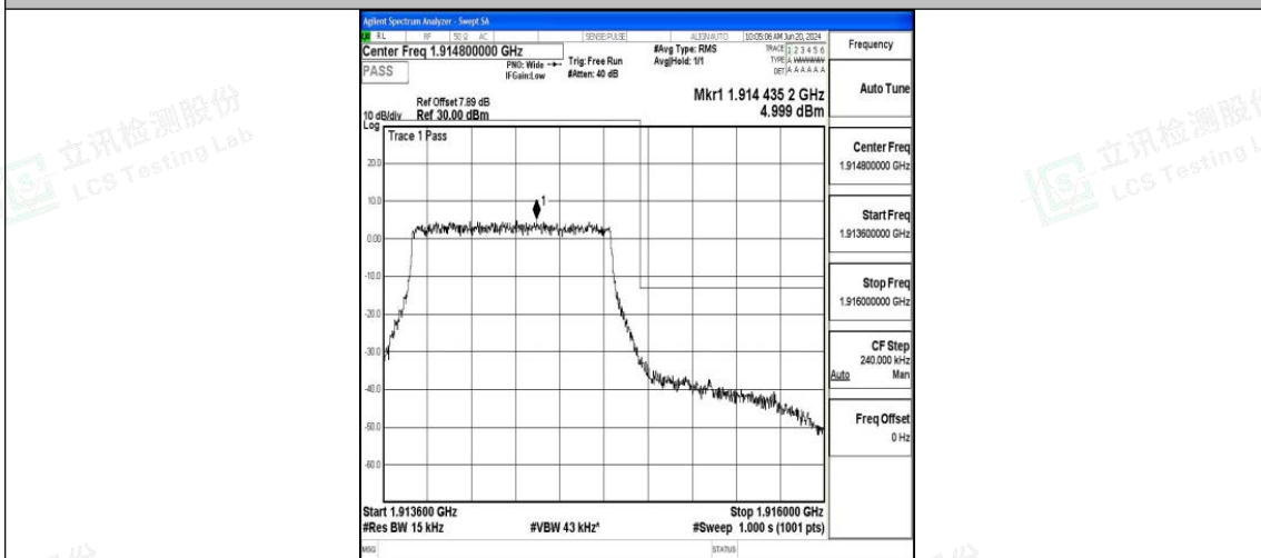
Band25_1.4MHz_QPSK_26683_6RB#0
