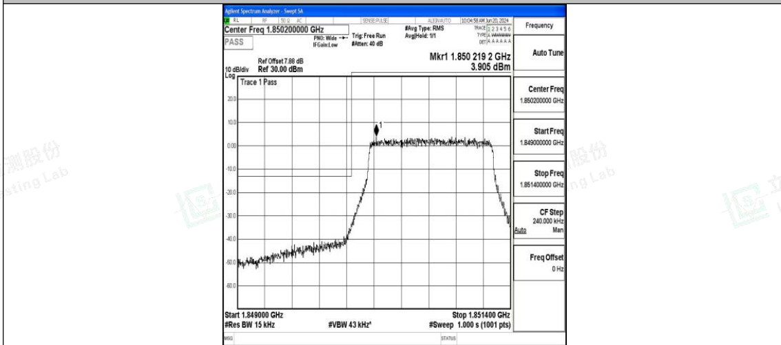
Band25_1.4MHz_16QAM_26047_6RB#0
