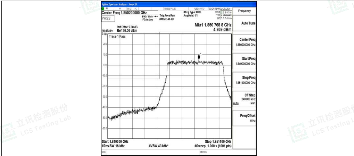
Band25_1.4MHz_QPSK_26047_6RB#0
