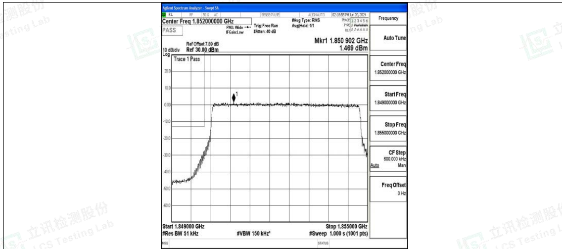
Band25_5MHz_16QAM_26065_25RB#0
