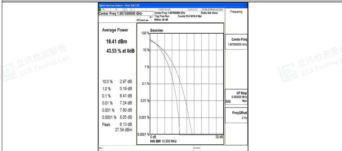
Band25-15MHz-16QAM-26615-75RB#0-PASS
