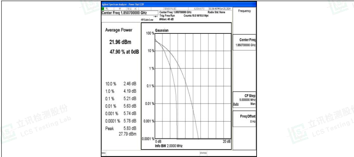
Band25-1.4MHz-QPSK-26047-1RB#0-PASS
