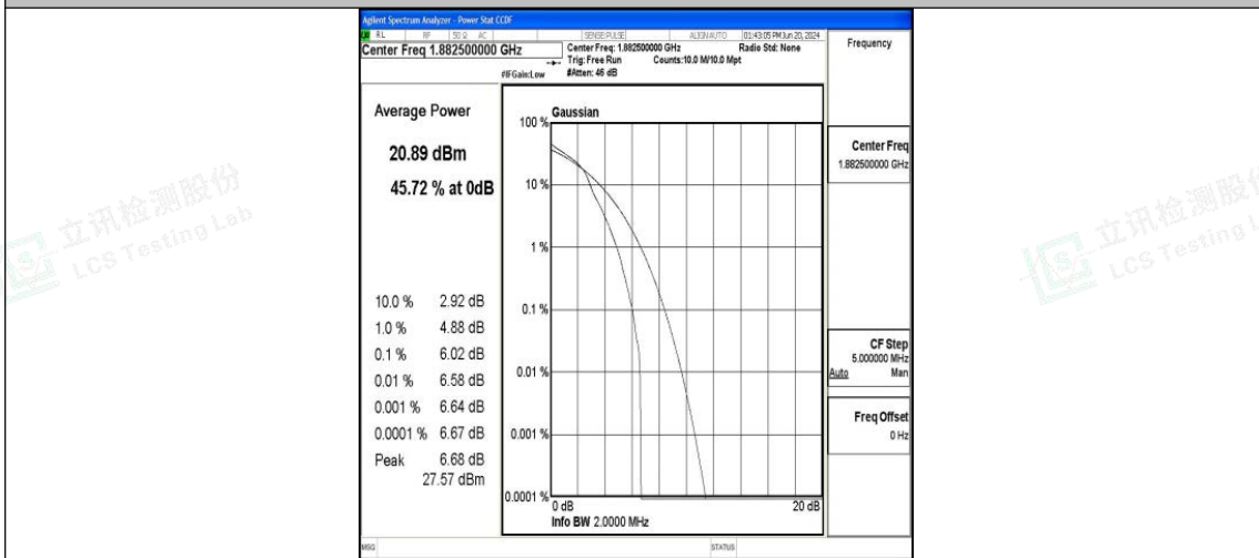
Band25-1.4MHz-16QAM-26365-1RB#0-PASS
