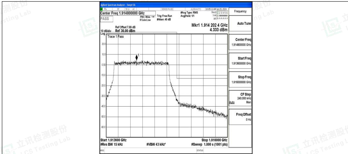
Band25_1.4MHz_16QAM_26683_6RB#0
