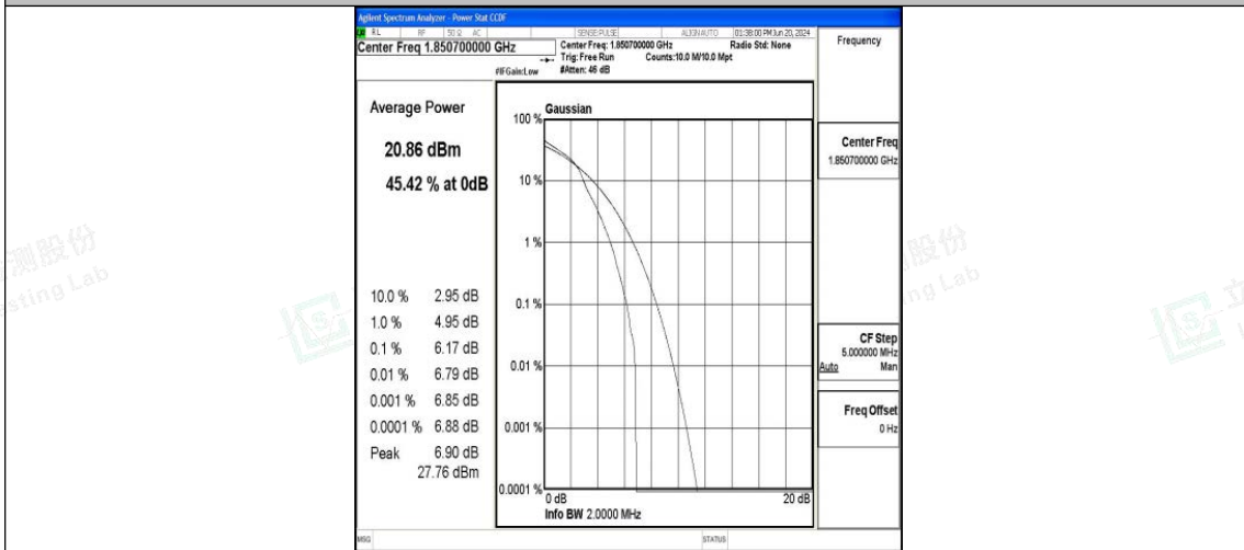
Band25-1.4MHz-16QAM-26047-1RB#0-PASS
