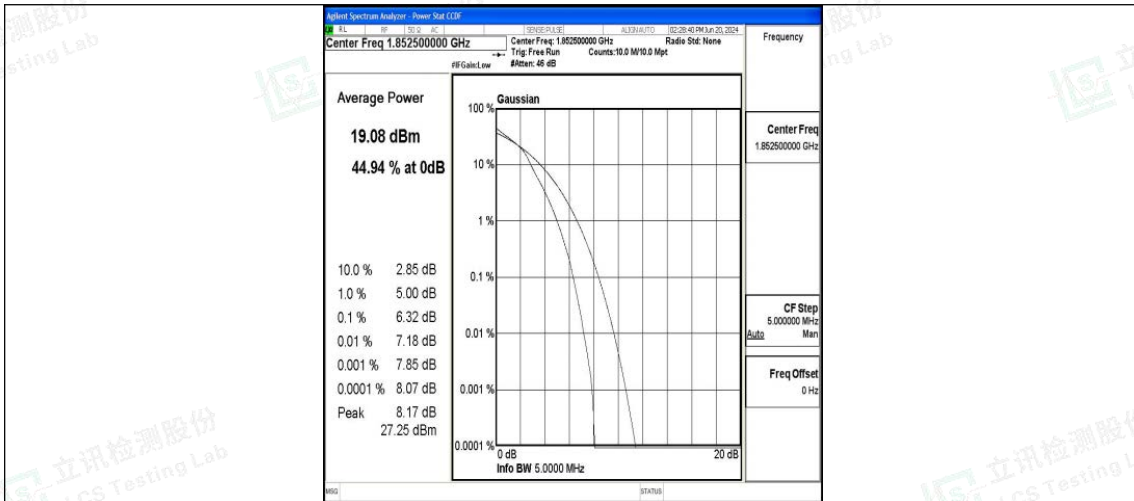
Band25-5MHz-16QAM-26065-25RB#0-PASS
