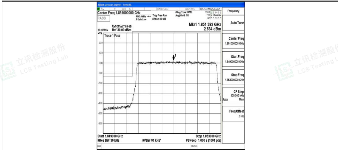
Band25_3MHz_16QAM_26055_15RB#0
