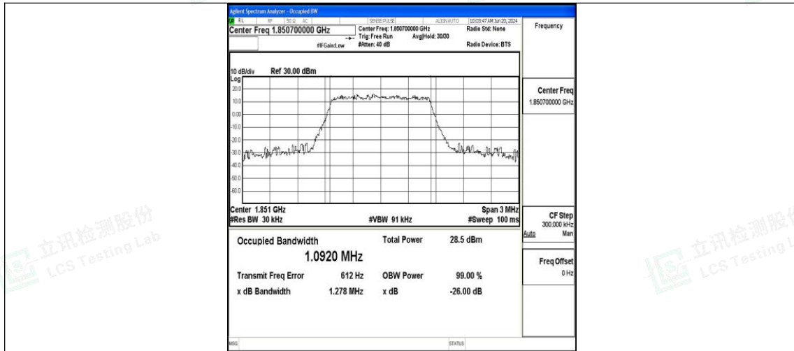
Band25-1.4MHz-QPSK-26047-6RB#0-PASS
