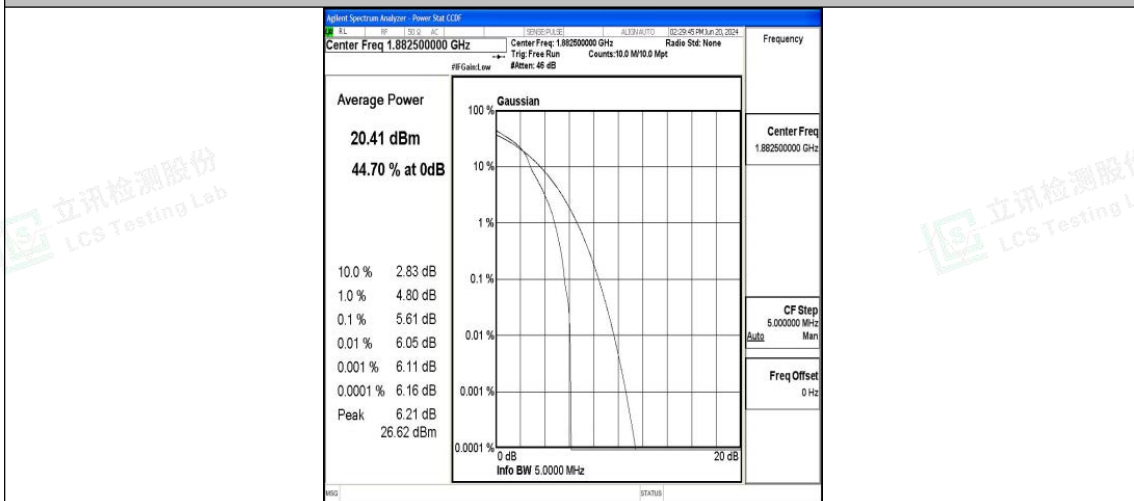
Band25-5MHz-16QAM-26365-1RB#0-PASS
