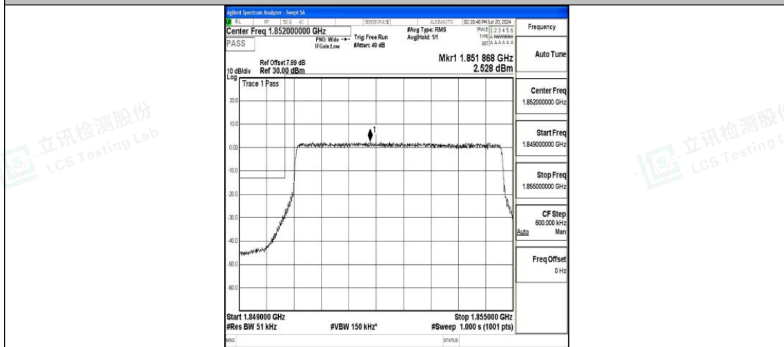
Band25_5MHz_QPSK_26065_25RB#0
