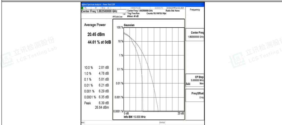
Band25-15MHz-16QAM-26365-1RB#0-PASS
