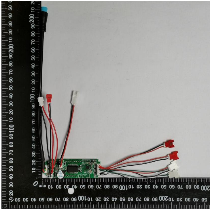
INTERNAL PHOTO OF SAMPLE
