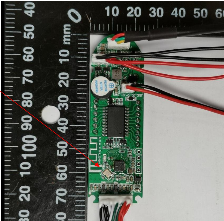
INTERNAL PHOTO OF SAMPLE PCB
