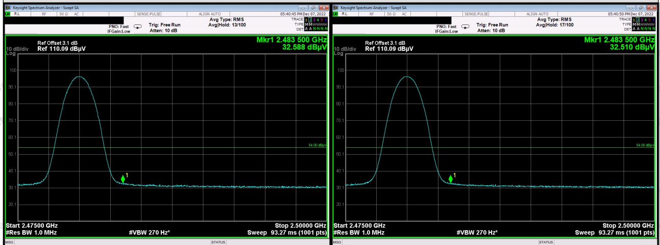
Average Value(Vertical)
