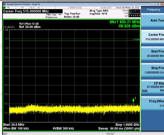
2.4G_Ant1_2441.4_30~1000
