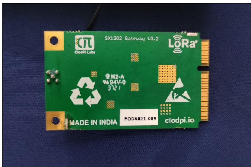
EUT Rear View
