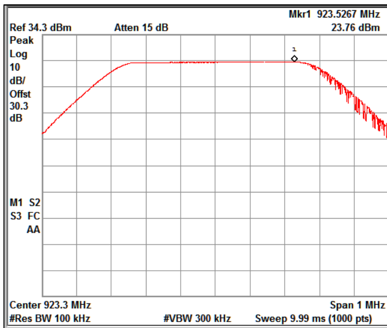
Reference plot for 923.3MHz
