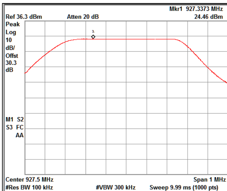
Reference plot for 927.5MHz
