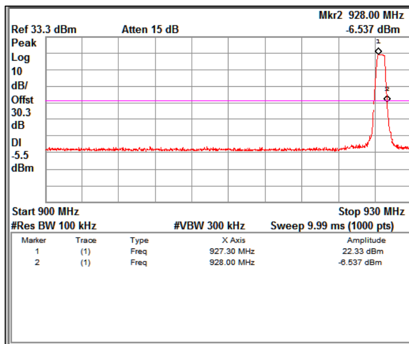
Band edge Channel Frequency 927.5MHz
