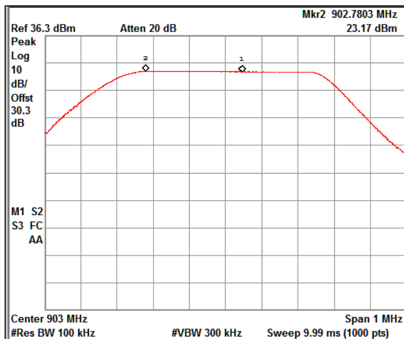
Reference plot for 903MHz
