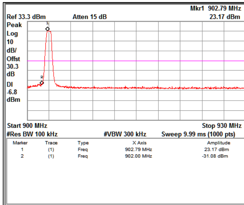
Band edge Channel Frequency 903MHz
