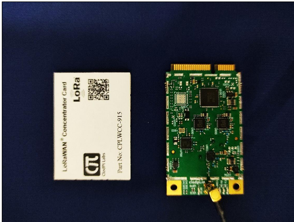
Module Without Shield enclosure
