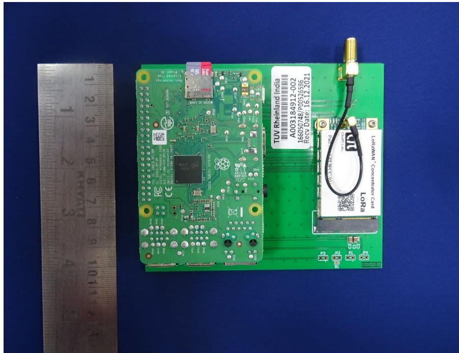
Test Supporting board and EUT Front view
