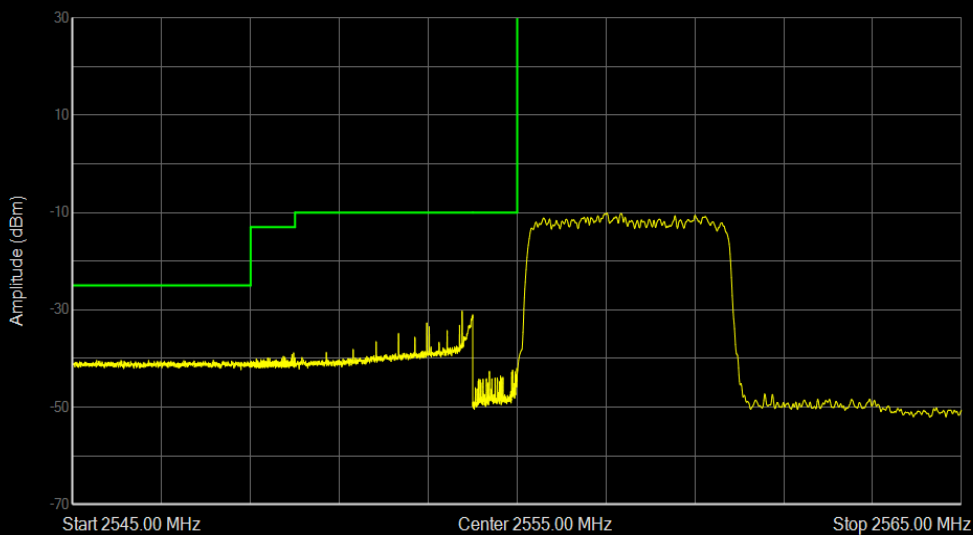
Band41 QAM16 BW=5MHz Channel=40265 RB Size=25 Position=#0
