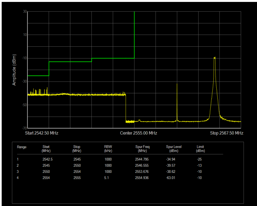
Band41 QAM16 BW=10MHz Channel=40290 RB Size=1 Position=#0
