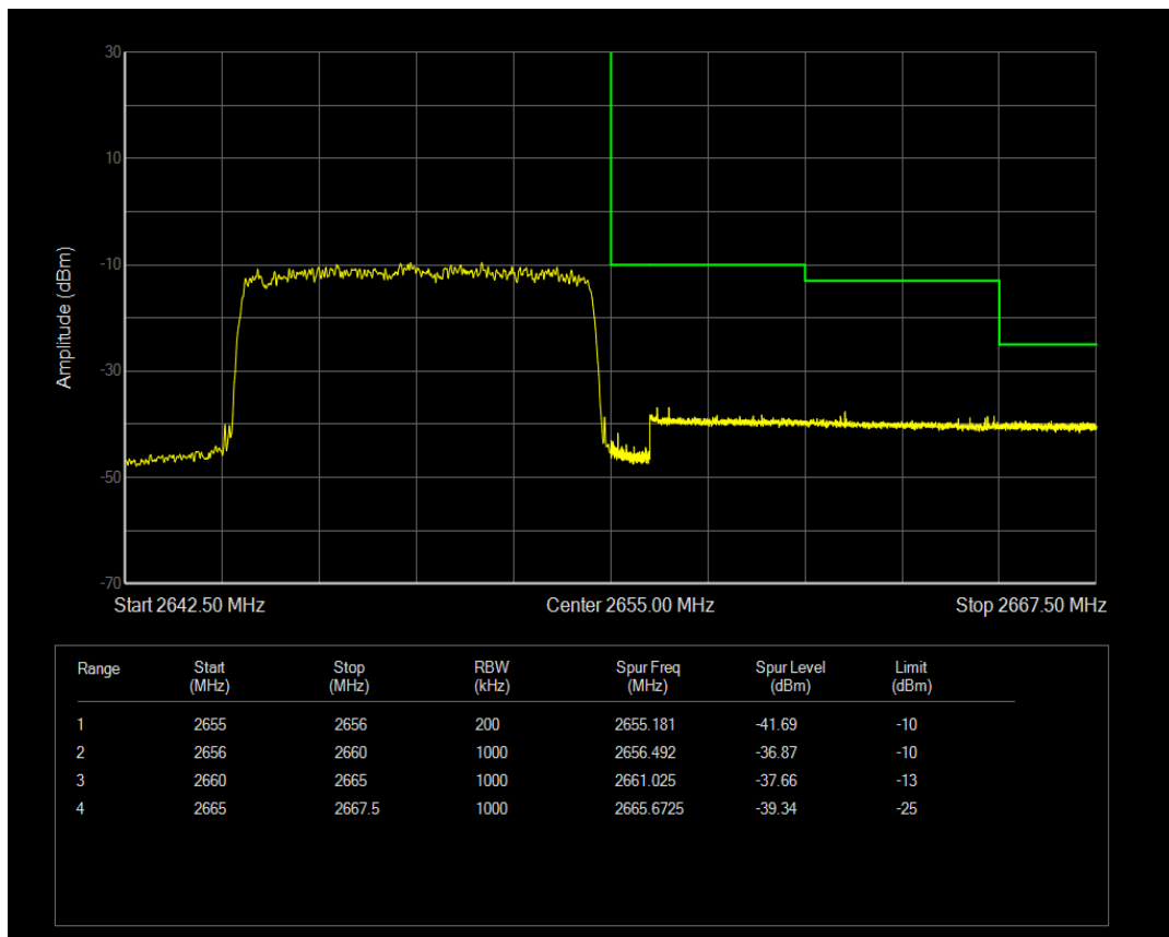
Band41 QAM16 BW=10MHz Channel=41190 RB Size=1 Position=#Max
