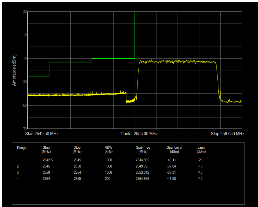
Band41 QAM16 BW=10MHz Channel=40290 RB Size=1 Position=#Max
