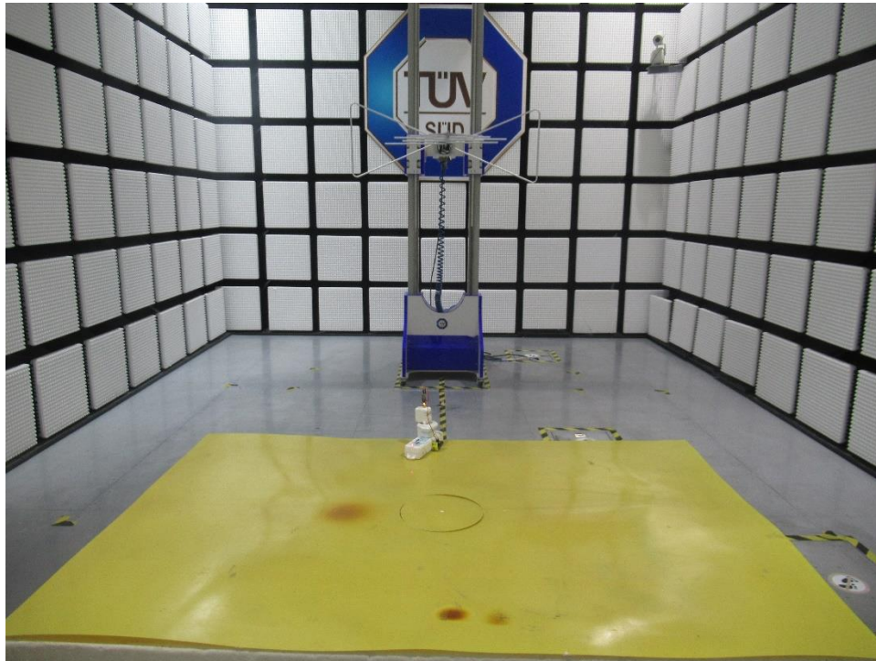
Test Setup for 30MHz to 1000MHz
