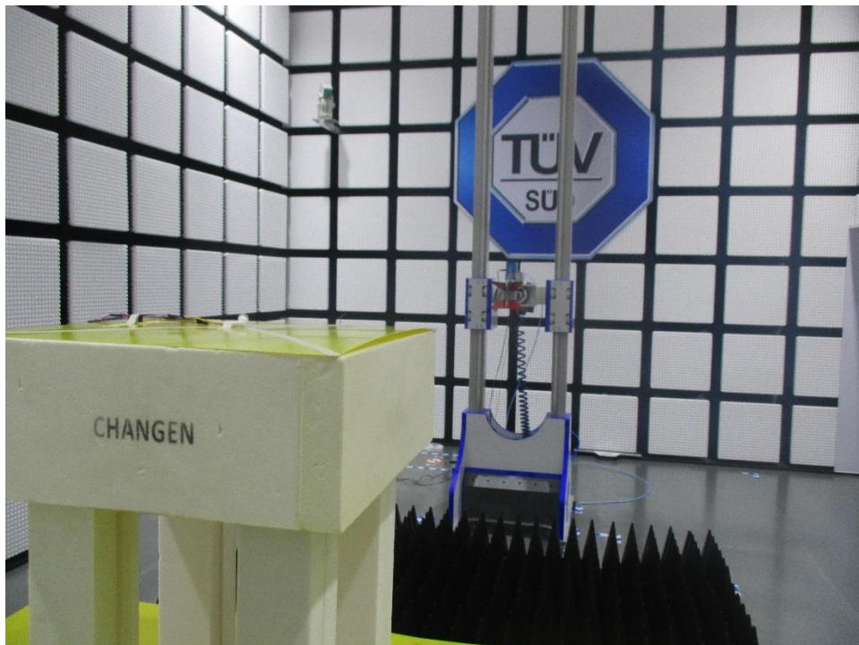
Test Setup for 1GHz to 18GHz
