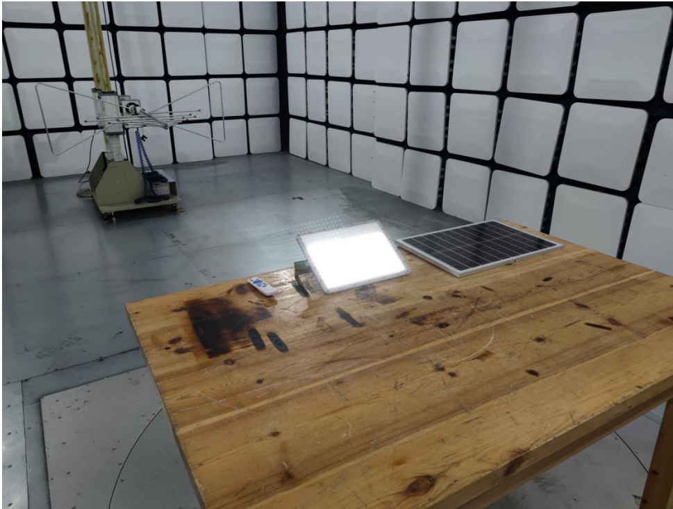
FCC ID: 2A32V-TK08-300W Photo of Radiation Emission Test
