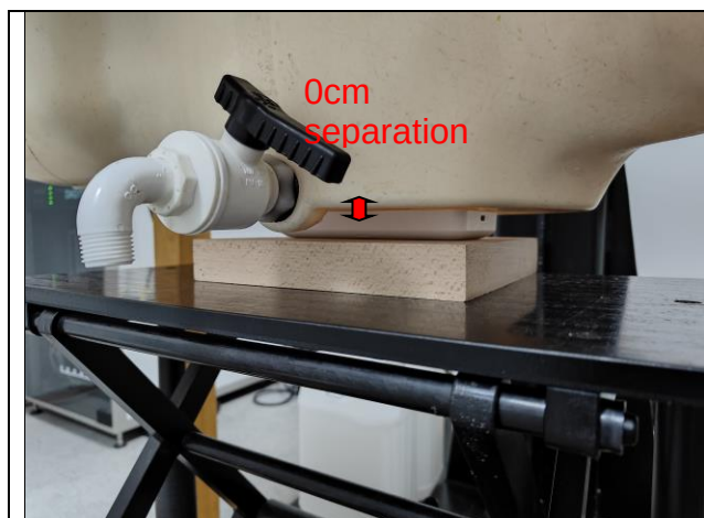
Body(Front side)
