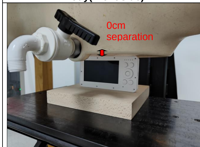
Body(Top edge)
