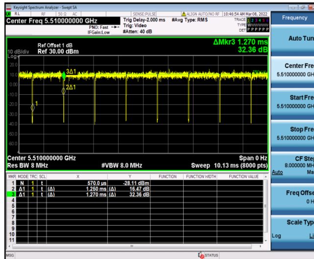
11AC40SISO_Ant1_5510
