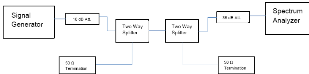
Figure 3-2 Test Setup for Conducted Measurement Radar Verification
