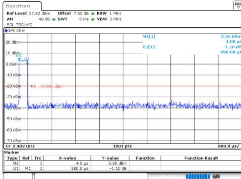
One Pulse NVNT 2-DH5 2402MHz
