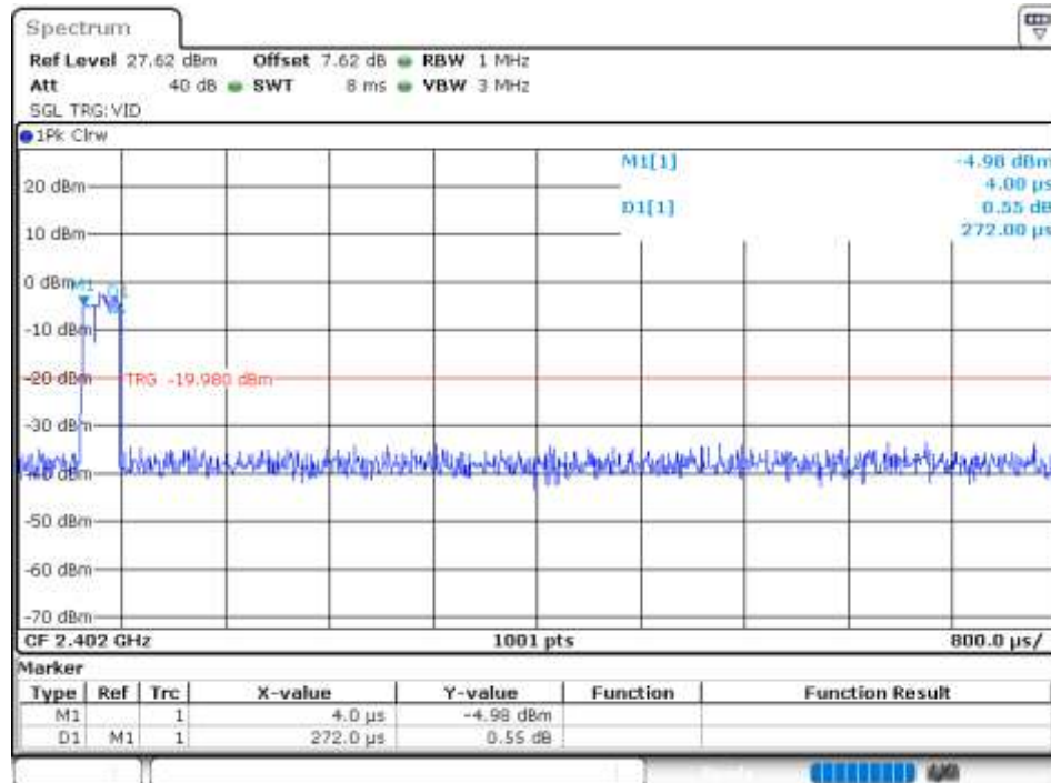
One Pulse NVNT 3-DH5 2402MHz
