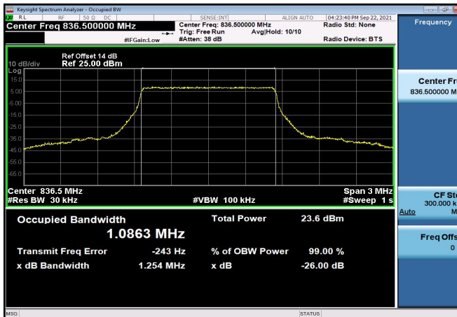
FDD05_MidRange_3_836.5_QPSK
