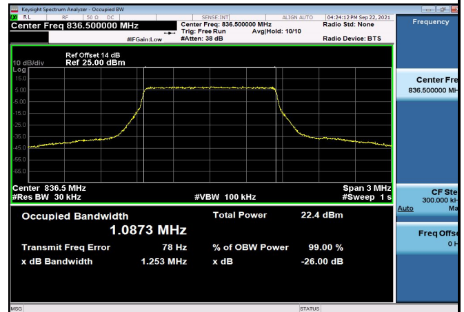
FDD05_MidRange_3_836.5_Q16
