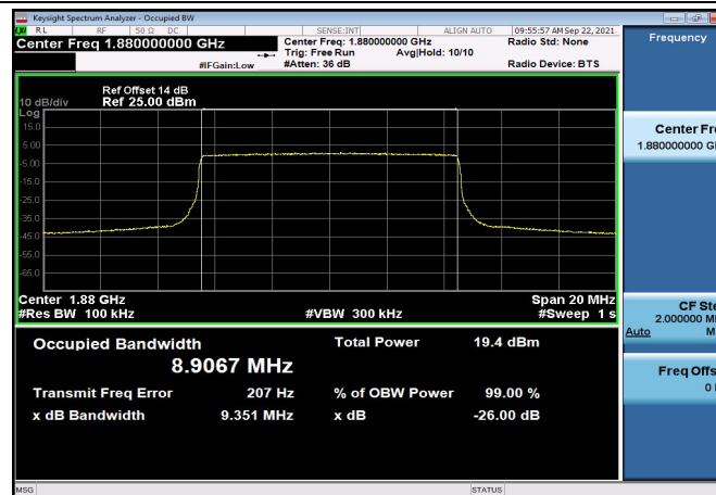
FDD02_MidRange_10MHz_1880MHz_QPSK
