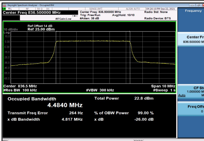
FDD05_MidRange_5_836.5_QPSK
