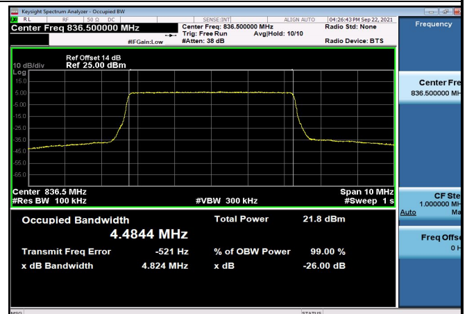
FDD05_MidRange_5_836.5_Q16
