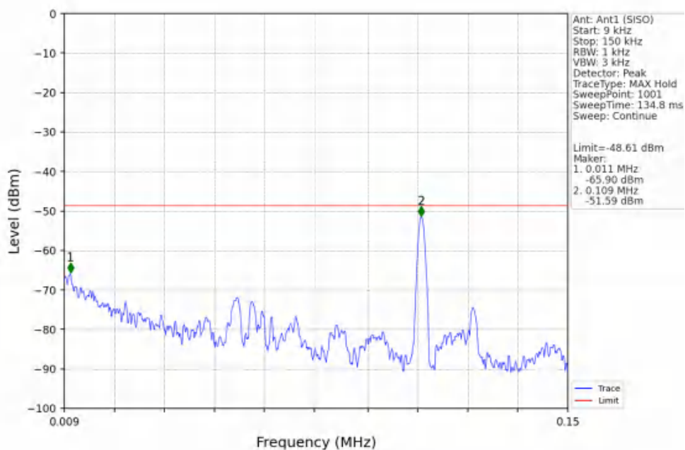
802.11ax(HEW40)_HCH_2452MHz_SU_ / _Ant1 (SISO)_ NTVN
