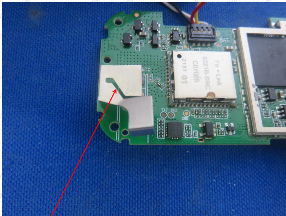
WIFI ANT
