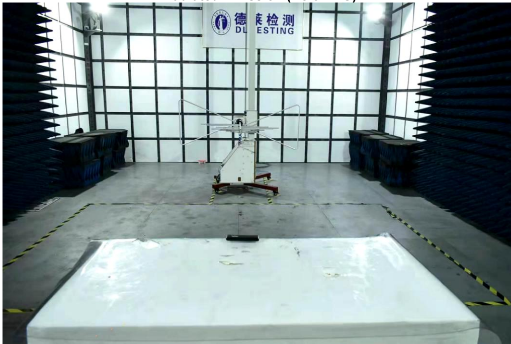
Radiated Emission (Below 1G)
