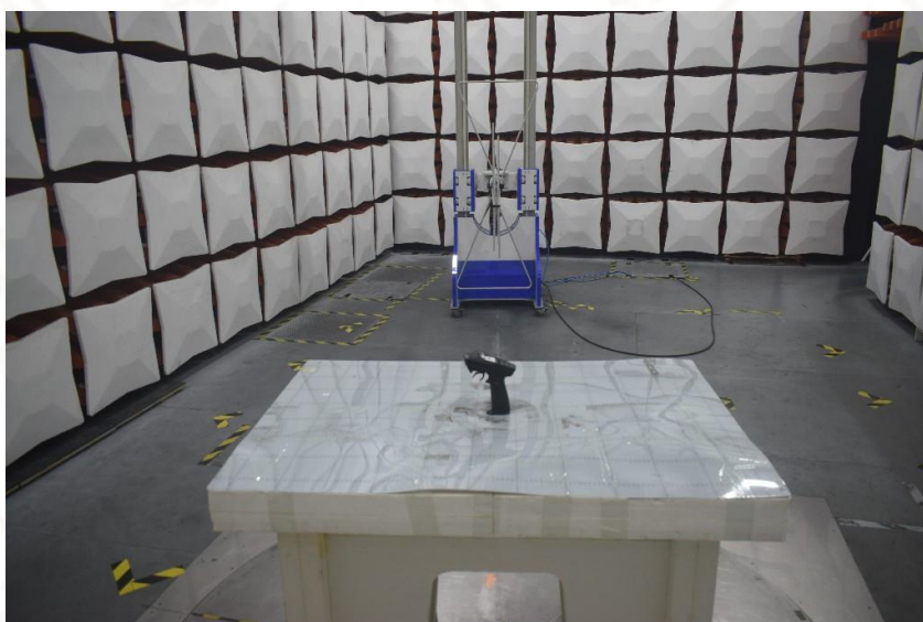
TX 30MHz~1GHz
