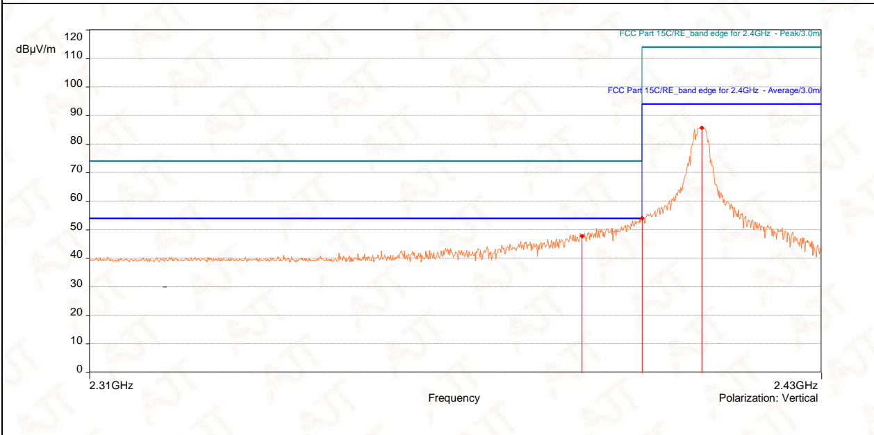
2410MHz Vertical
