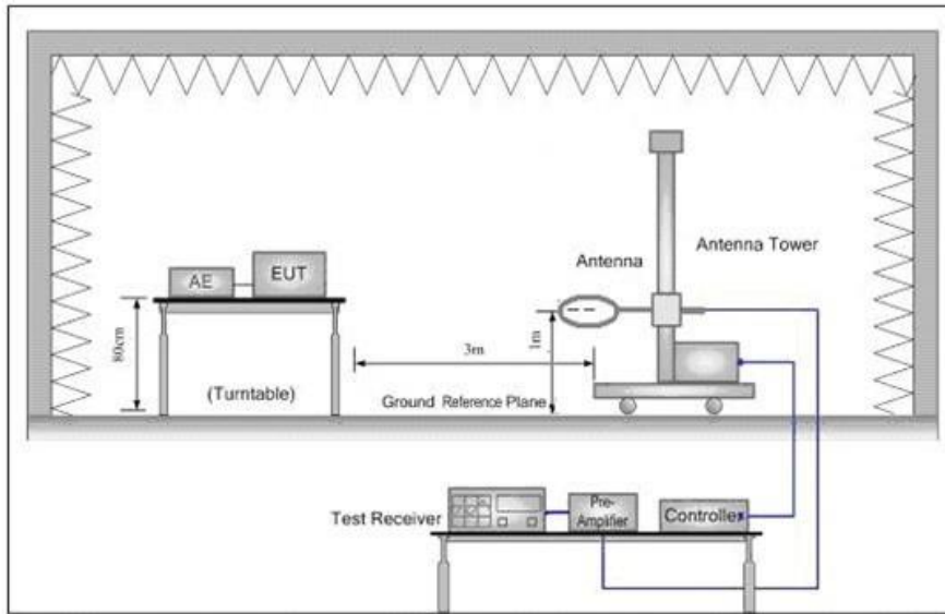
Below 30MHz
