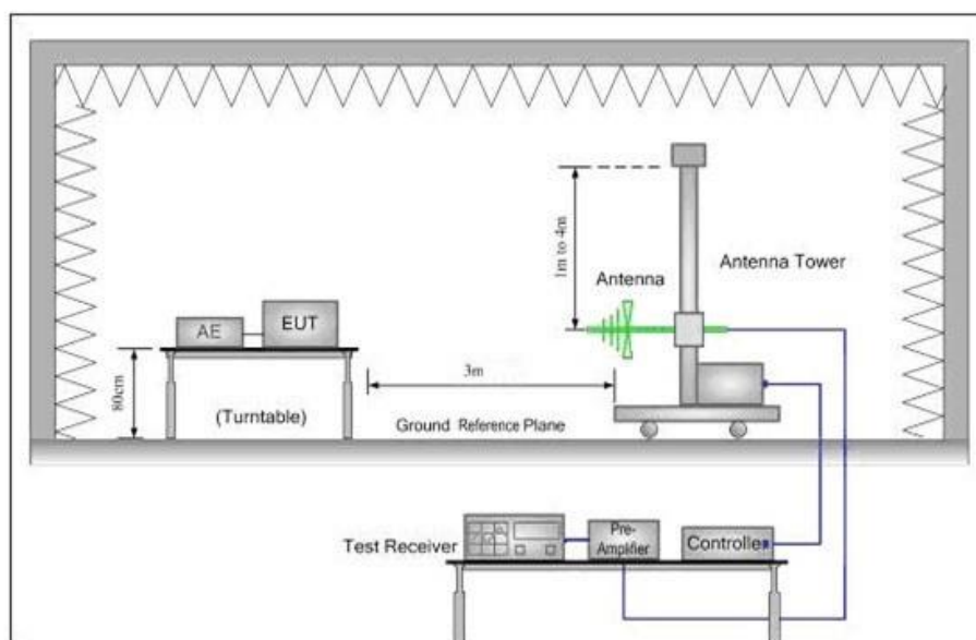
30MHz-1GHz
