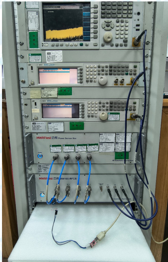
Photo of Setup for Conducted Measurement
