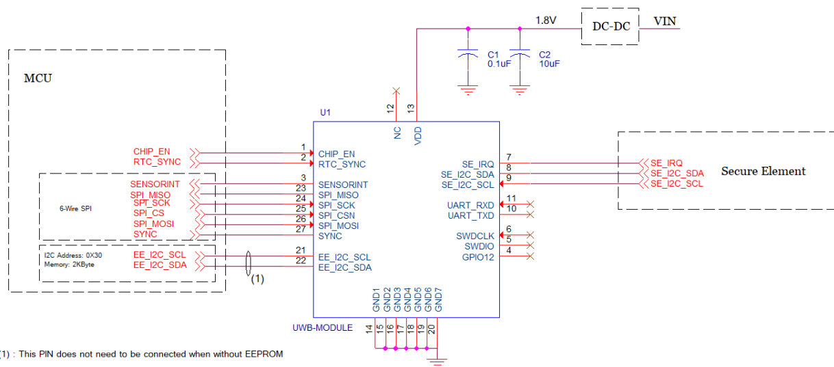
Reference schematics for SWM1000SR1503XFE
