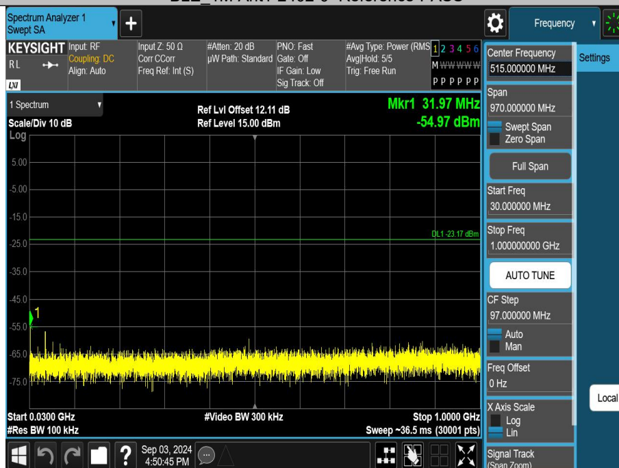
BLE_1M-Ant1-2402-30~1000-PASS
