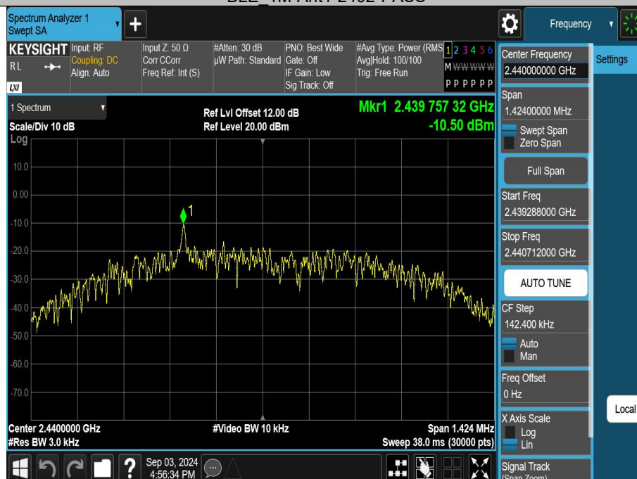
BLE_1M-Ant1-2440-PASS
