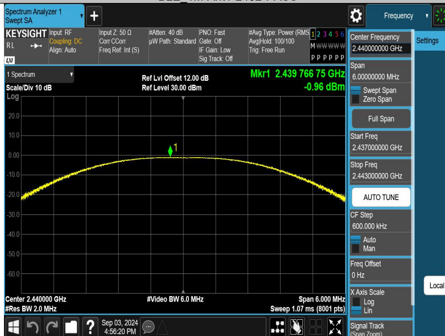
BLE_1M-Ant1-2440-PASS
