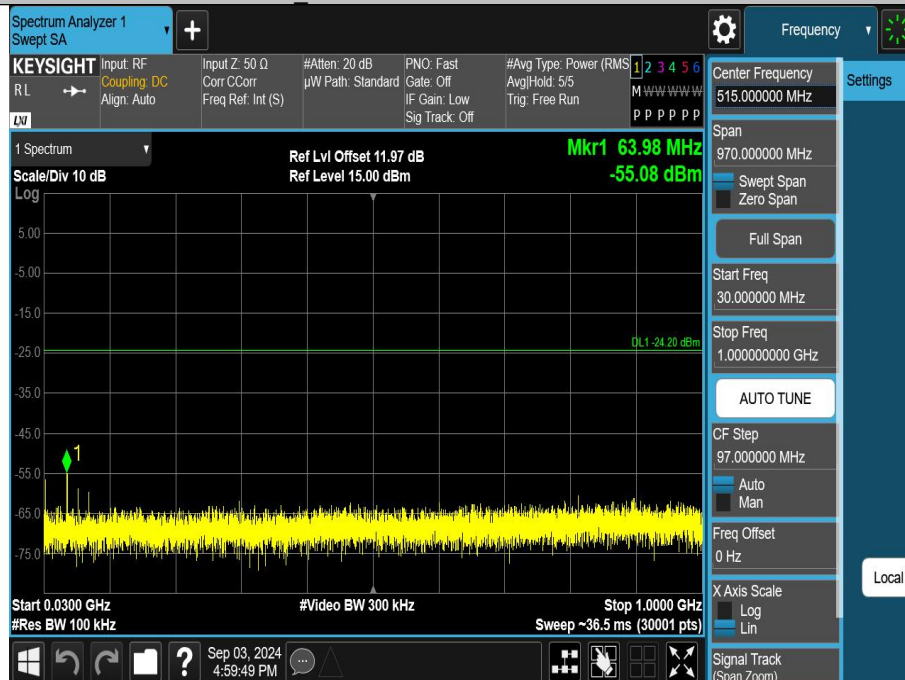
BLE_1M-Ant1-2480-30~1000-PASS
