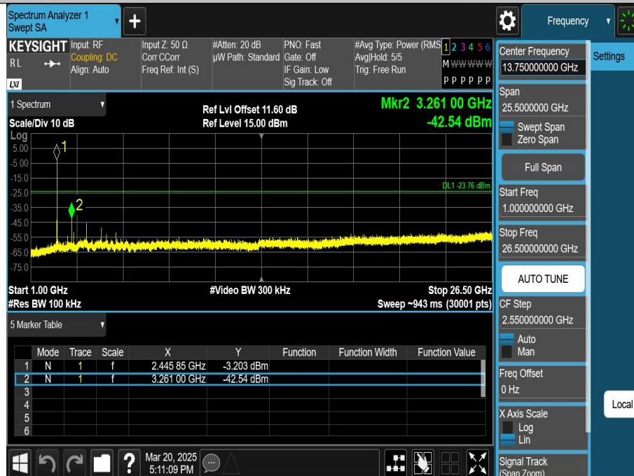
DH5-Ant1-2446-1000~26500-PASS
