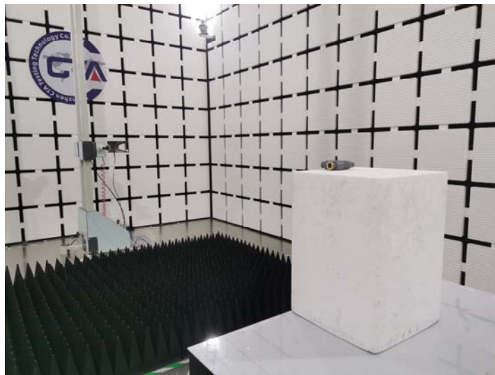
radiation H
