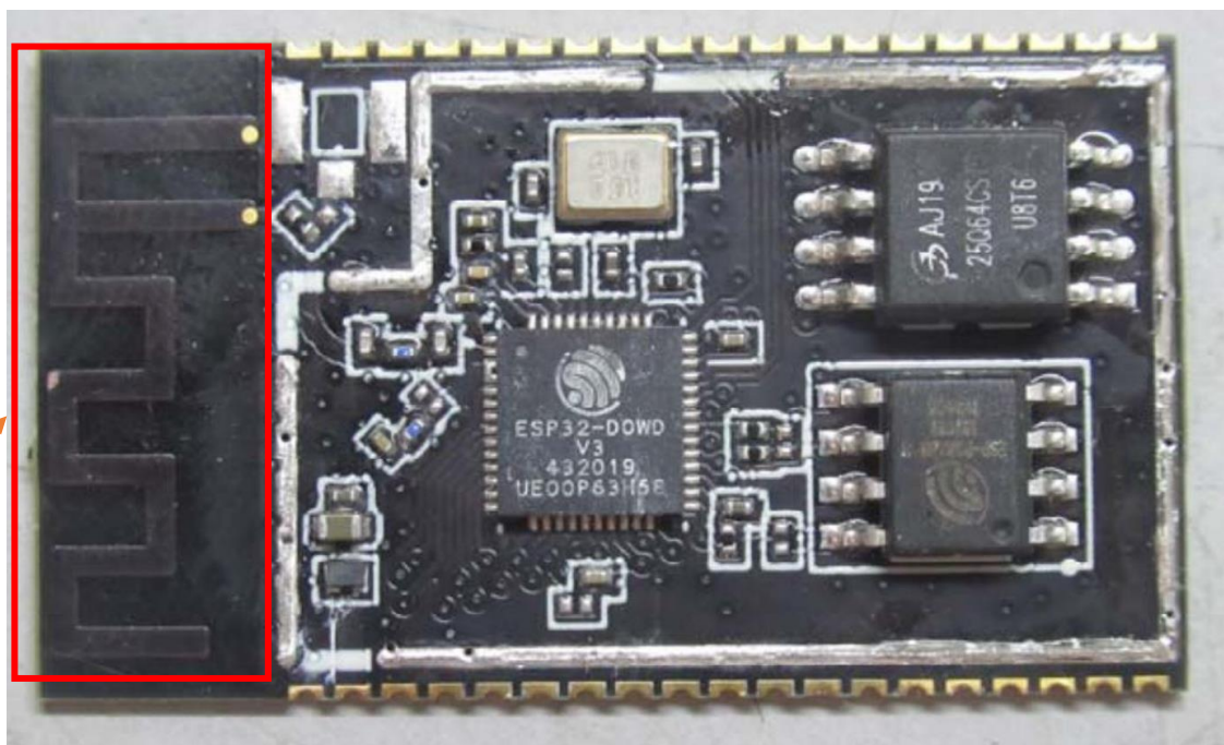
PCB Antenna
